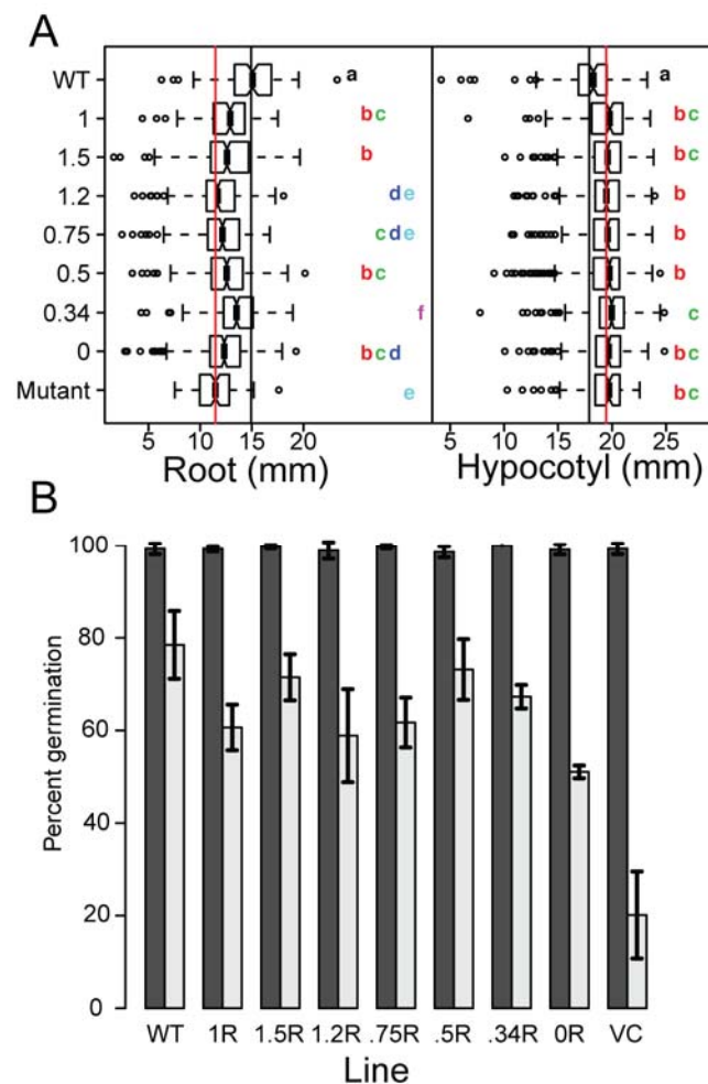
Figure 3. PFT1 STR alleles differ in their ability to rescue a pft1 loss-of-function mutant for early seedling phenotypes. A) Strains sharing letters are not significantly different by ANOVA with Tukey's HSD test. Black lines represent WT means, red lines represent pft1-2 means for each phenotype. Each allele is represented by at least two independent transgenic lines, N>100 for all phenotypes for each allele, pooled across at least two experiments; \alpha = 0.05 . Hypocotyl length and root length were assayed in 7d seedlings grown in dark conditions. B) Dark and light bars represent mean germination across 3 biological replicates on 0 mM NaCl and 200 mM
