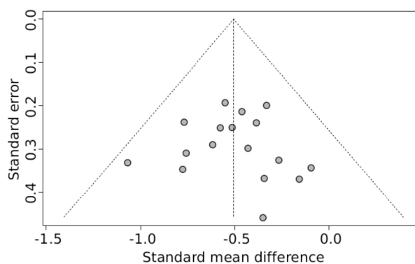
Figure 3. Standard error versus standard mean difference.
