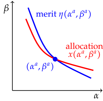
Figure 5b: Allocation rule implemented using only ordeals
