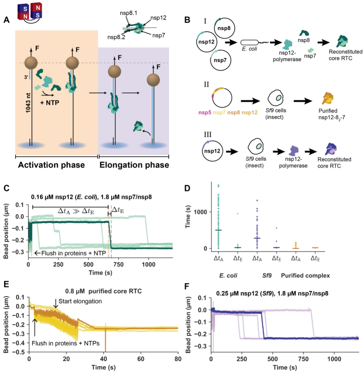
Figure 1: Slow activation by reconstituted SARS-CoV-2 core RTCs. (A) Schematic of the magnetic tweezers assay to monitor activation and elongation by the SARS-CoV-2 core RTC (Materials and Methods). (B) Schematic representation different methods of obtaining the core RTC used throughout this work. (I) nsp7, nsp8 and nsp12-polymerase were separately and recombinantly expressed in E. coli , (II) purification of core RTC complex after expressing a bacmid containing nsp5-Mpro (main protease), nsp8, nsp7, and nsp12-polymerase in Sf9 cells, (III) nsp7, nsp8 and nsp12-polymerase were separately and recombinantly expressed in E. coli and nsp12-polymerase was recombinantly expressed in Sf9 (Materials and Methods). Color coding for the different core RTCs is kept in subsequent figures to represent to related data. (C) Example time traces for the reconstituted SARS-CoV-2 core RTC using 0.16 \mu\text{M} nsp12-polymerase (see (I) in panel B) and 1.8 \mu\text{M} of nsp7 and nsp8. The orange and purple dashed lines indicate the end of the activation and elongation phases. \Delta t_A and \Delta t_E are their respective durations. (D) \Delta t_A and \Delta t_E for all recorded traces in experiments of which representative subsets are shown in panels C, E and F. Horizontal markers indicate the group medians.
