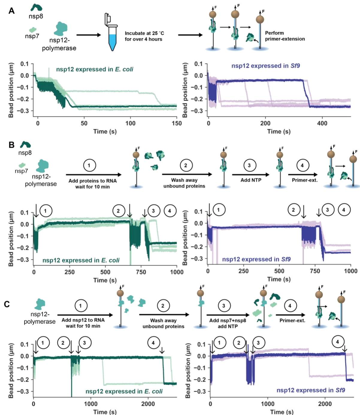
Figure 3: Presence of the template RNA reduces activation times. Example time traces are shown for a reconstituted core RTC. (A) Nsps were added together 4.5 hrs (nsp12-polymerase expressed in E. coli ) or 6.5 hrs (nsp12-polymerase expressed in Sf9 ) prior to diluting them to 0.2 μM nsp12, 1.8 μM nsp7 and nsp8 and performing primer-extensions. (B) (1) The proteins were added to the RNA tethering the magnetic beads in the flow chamber. (2) Ten minutes later 500 μL of reaction buffer was used to rinse the flow chamber from free-floating proteins. (3) Finally, ribonucleotides were added and (4) Activation typically started during step (3). (C) (1) After tethering the magnetic beads to the RNA, 0.2 μM of nsp12-polymerase and 500 μM of NTP were added. (2) Ten minutes later 500 μL of reaction
