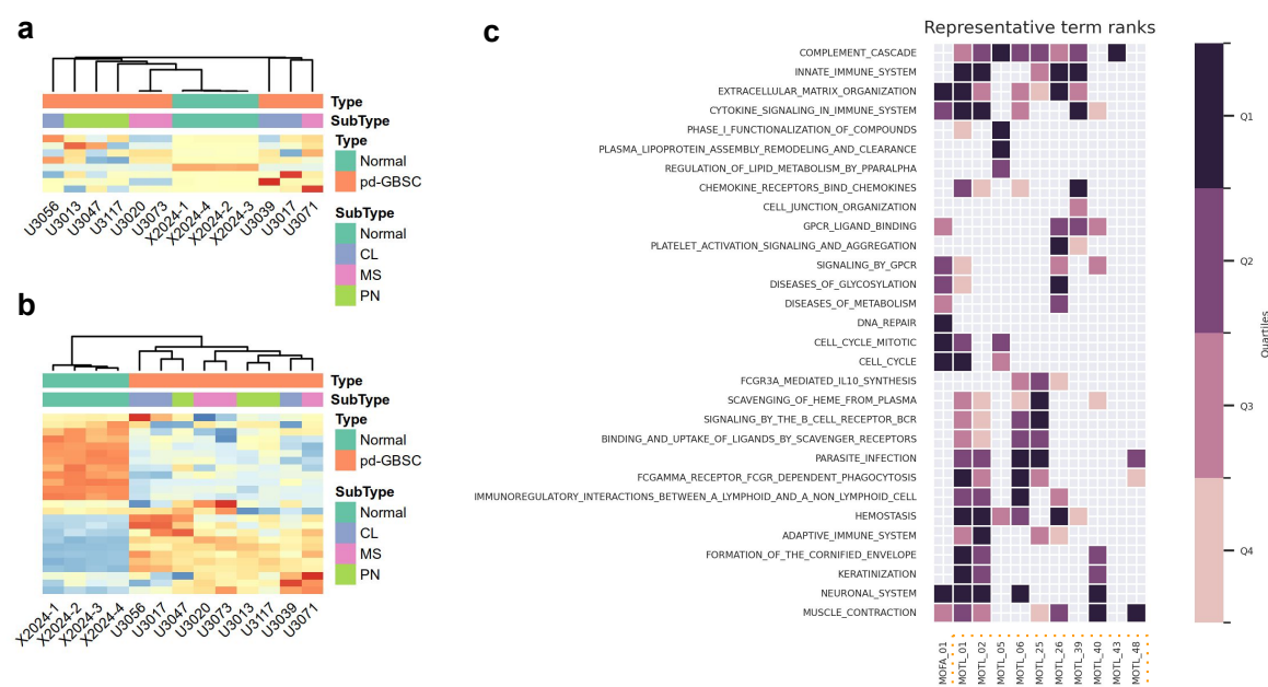
Figure 4: Heatmaps of factorizations and gene set enrichment analysis of glioblastoma data: The heatmaps are based on factorizations and subsequent gene set enrichment analysis of the target dataset comprised of multi-omics data (mRNA expression, DNA methylation) for all normal and patient-derived glioblastoma stem cell (pd-GBSC) samples. The multi-omics data was obtained from Santamarina-Ojeda et al., who also provided subtypes for the cancer samples, previously defined from transcriptomic signatures: CN (classical), PN (proneural), MS (mesenchymal). a Heatmap of the score matrix, Z , inferred with Direct MOFA factorization of the target dataset. The rows are the factors, the columns are the samples, and the cells are the row-wise centered and scaled factor values. The rows and columns were ordered with hierarchical clustering (complete-linkage). b Heatmap of Z matrix inferred with MOTL factorization of the target dataset. c Reactome enrichment results for direct MOFA and MOTL factors. We performed gene set enrichment analysis on the direct MOFA and the 11 MOTL factors that were differentially active between normal and cancer samples, and that explained at least 1% of mRNA variance. This yielded a set of Reactome processes and pathways significantly associated with either one direct MOFA factor or one or more of 10 different MOTL factors. The Reactome processes and pathways were filtered, clustered, and plotted with orsum. The colors represent the quartiles of enrichment significance for each factor (darker means more significant).
