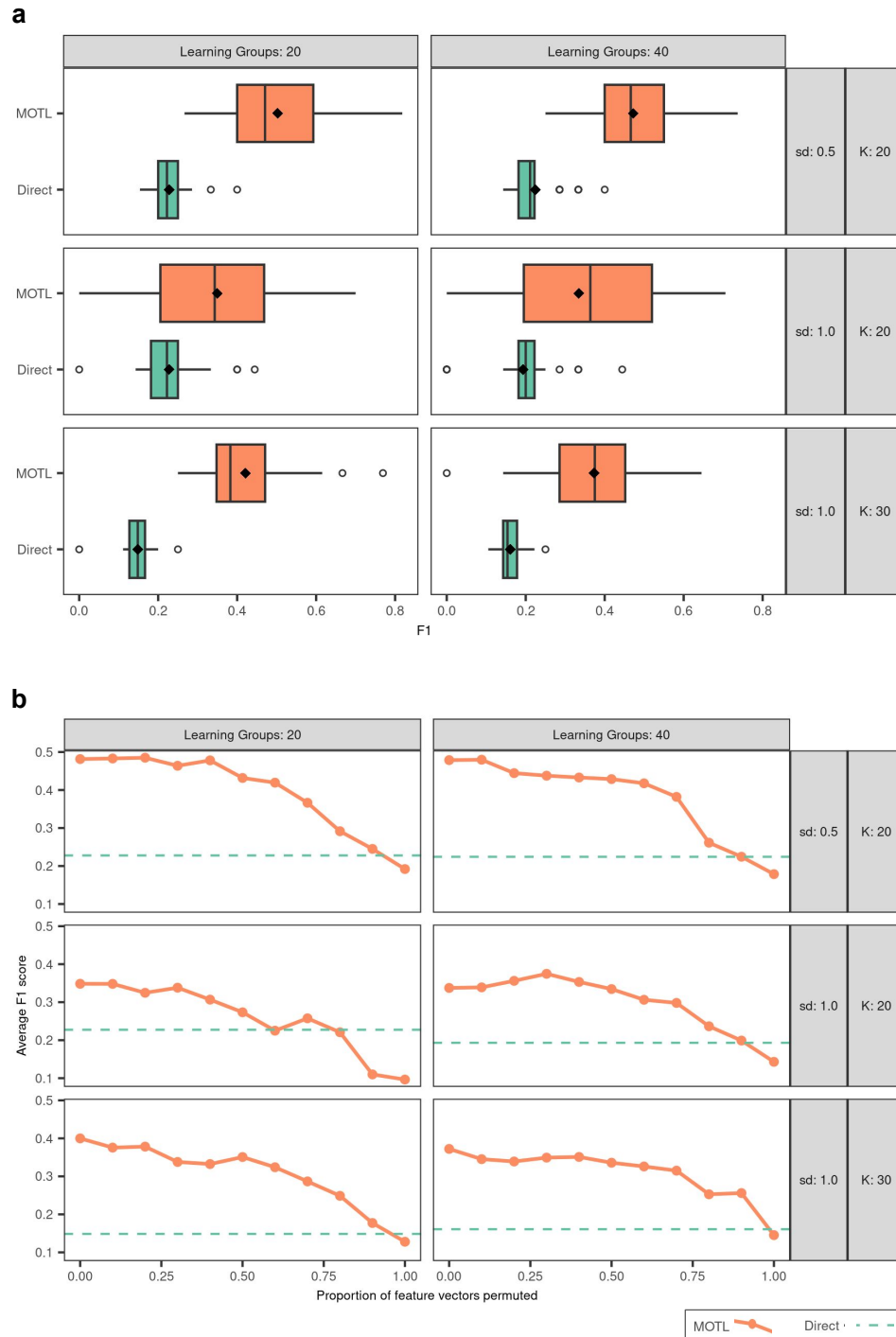
Figure 2: Evaluation of factorizations of small simulated multi-omics target datasets. a The boxplots represent the F1 scores obtained for factorizations with and without MOTL transfer learning, for different simulation configuration settings. Simulation configurations varied in the number of groups of samples used for the learning dataset ( Learning Groups ), the number of groundtruth factors ( K ), or the standard deviation used to simulate z_{nk} values ( sd ). F1 scores take a value between 0 and 1, and higher values indicate better factorizations. Each boxplot is based on 30 F1 scores. The hinges of the boxes are the 25 th and 75 th percentiles, the middle lines are medians, the diamonds are the mean values, and the whiskers are either extreme values or extend 1.5 times the inter-quartile range from the hinge. b The line plots represent the average F1 score obtained from MOTL factorizations, for different simulation configuration settings, after permuting the values in proportions of the feature vectors in the W^{(m)} matrices obtained from prior factorization of L . The dashed line is the average F1 score obtained with direct MOFA factorization for the simulation configuration.
