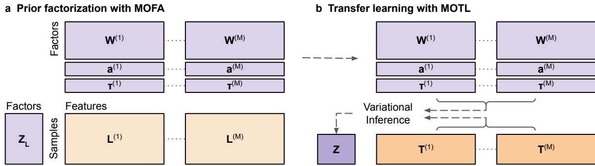
Figure 1: Overview of MOTL, our transfer learning approach to joint multi-omics matrix factorization based on variational Bayesian inference. a A multi-omics learning dataset, \mathbf{L} , consisting of M omics matrices, \mathbf{L}^{(m)} , m = 1, \dots, M , is factorized with MOFA to infer a matrix of feature weights, \mathbf{W}^{(m)} , vector of feature-wise intercepts, \mathbf{a}^{(m)} , and a vector of feature-wise precision parameter values, \boldsymbol{\tau}^{(m)} , for each \mathbf{L}^{(m)} . b The feature weight, intercept, and precision parameter values, inferred from the factorization of \mathbf{L} , are incorporated into the factorization of a multi-omics target dataset, \mathbf{T} , for which MOTL infers a matrix of sample scores, \mathbf{Z} , with variational inference.
