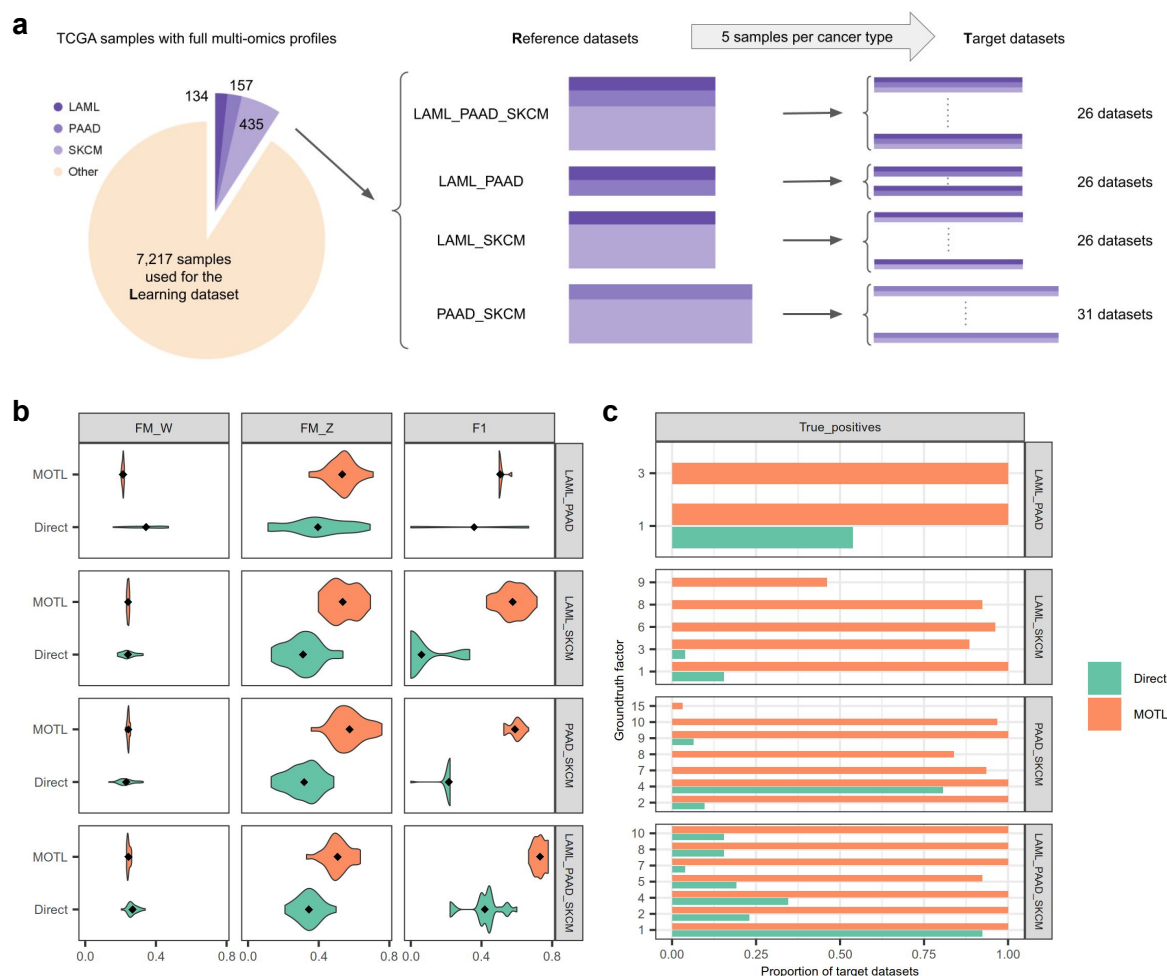
Figure 3: Evaluations using TCGA multi-omics data. a We created TCGA target, T , datasets from two or three cancer types: For each combination of cancer types we created a reference, R , dataset containing multi-omics data for all samples from the selected cancer types. We then randomly split R into non-overlapping T datasets, containing multi-omics data for five samples per cancer type. We did this for subsets of the set of cancer types \{LAML, PAAD, SKCM\} . In total we created, and split, four reference datasets, each of which contained multi-omics data for all samples from either two (LAML and PAAD, LAML and SKCM, PAAD and SKCM), or three (LAML, PAAD and SKCM) cancer types. For datasets containing PAAD and SKCM samples only, we included mRNA, miRNA, DNA methylation, and SNV data. We did not include SNV data in datasets containing LAML samples, due to the sparsity of SNV data for LAML. b Comparison of factorization approaches applied to TCGA multi-omics datasets. Violin plots of F-measure values for weight matrix factors ( FM\_W ), F-measure values for score matrix factors ( FM\_Z ), and F1 scores ( F1 ). For each evaluation score, higher values indicate better factorizations. Scores are plotted by factorization method and by the cancer types characterizing the target dataset samples. c Frequency with which differentially active groundtruth TCGA factors were true positives. A differentially active groundtruth factor was a true positive if it was predicted as being differentially active based on a factorization of a target dataset. Each bar represents the proportion of target datasets, for which the factorization led to the differentially active groundtruth factor being a true positive. Proportions are plotted by factorization method, and by the cancer types characterizing the reference and target dataset samples.
