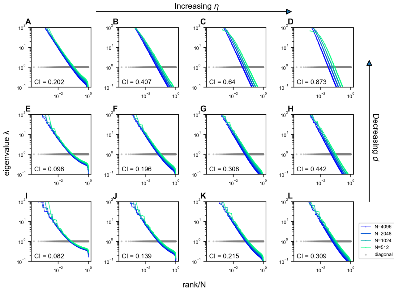
Figure S5. Impact of \eta and d on the scale invariance of covariance eigenspectra in the ERM with f(\vec{x}) = e^{-\|\vec{x}\|^\eta} . The columns from left to right correspond to \eta = 0.3, 0.5, 0.7, 0.9 , and the rows from top to bottom correspond to d = 1, 2, 3 (Eq. (2) and Eq. (11)). Other ERM simulation parameters: N = 4096 , \rho = 256 , L = (N/\rho)^{1/d} , \epsilon = 0.03125 and \sigma_i^2 = 1 . Each panel shows a single ERM realization. For visualization purposes, the views in some panels are truncated since we use the same range for the eigenvalues in all panels.
