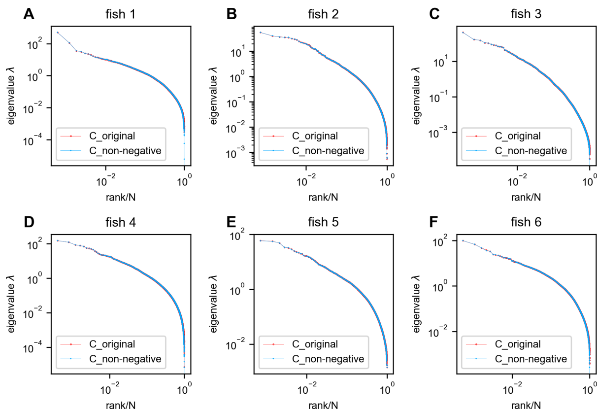
Figure S18. Negative covariances do not affect the eigenspectrum of the zebrafish data. Red: eigenspectrum of the original data covariance matrix. Blue: eigenspectrum of the covariance matrix with negative entries replaced by zeros. In this figure, all neurons recorded in each fish were utilized without any sampling.
