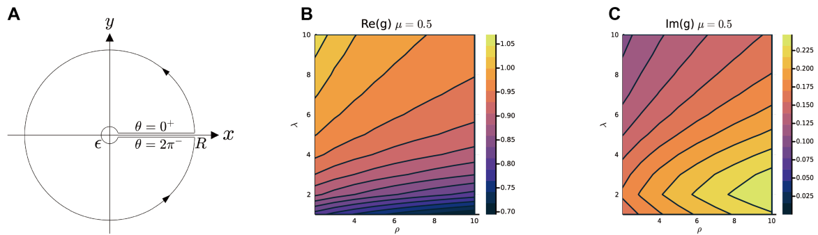
Figure S25. Calculate g_i and g_r . A. The path of the contour integral for g_i , g_r (Eq. (S67)). B-C. The heatmap of g_r and g_i with respect to \lambda and \rho . g_i , g_r in B, C are calculated by the numerical method (section 6.5.1). The parameters are N = 1024 , \rho = 10.24 , d = 2 , L = 10 , \mu = 0.5 , \epsilon = 0.03125 . \sigma_i^2 is i.i.d. sampled from a log-normal distribution with zero mean and a standard deviation of 0.5 in the natural logarithm of the \sigma_i^2 values; we also normalize E(\sigma_i^2) = 1 .
