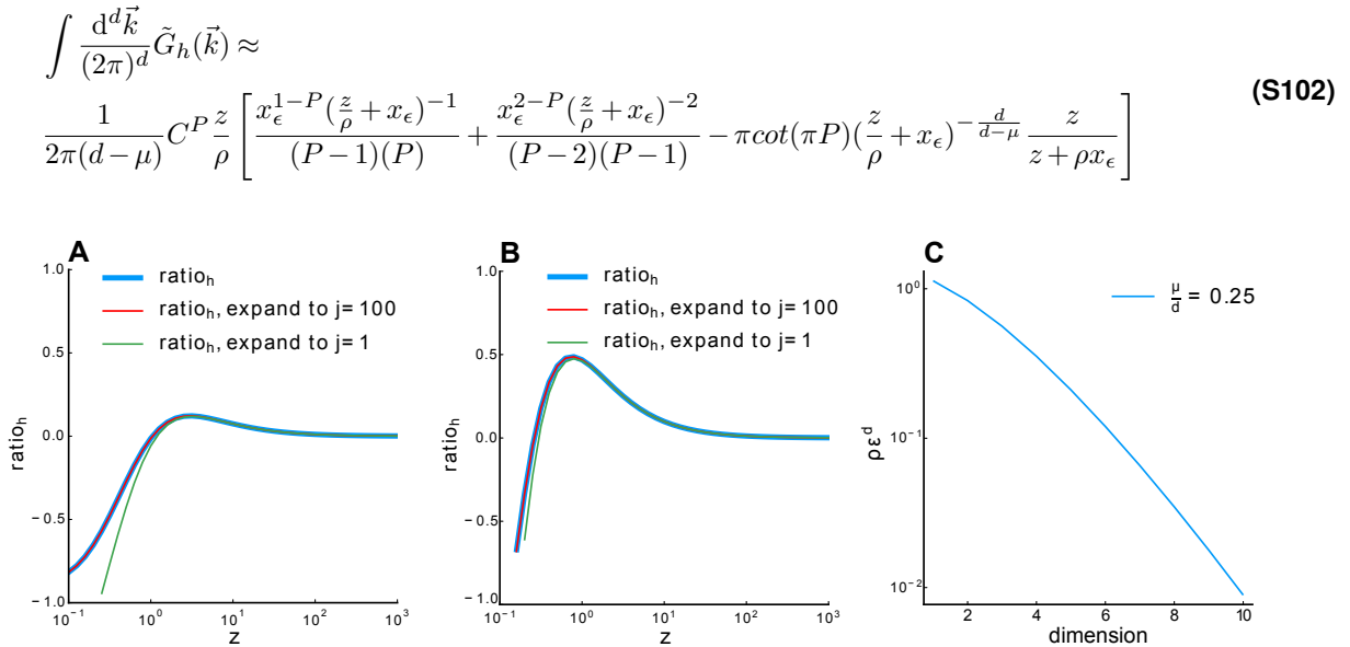
Figure S26. Relationship between ratio_h and z . A. \rho = 1024 , B. \rho = 256 . Blue line: ratio_h calculated numerically. Red line: 100-order expansion of Eq. (S101), which perfectly overlaps with the blue line. Green line: expansion to the first order. Other parameter: \mu = 0.5 , d = 2 , \epsilon = 0.03125 . C. Relationship between \rho \epsilon^d and dimension d with fixed \frac{\mu}{d} (Eq. (S105)).
