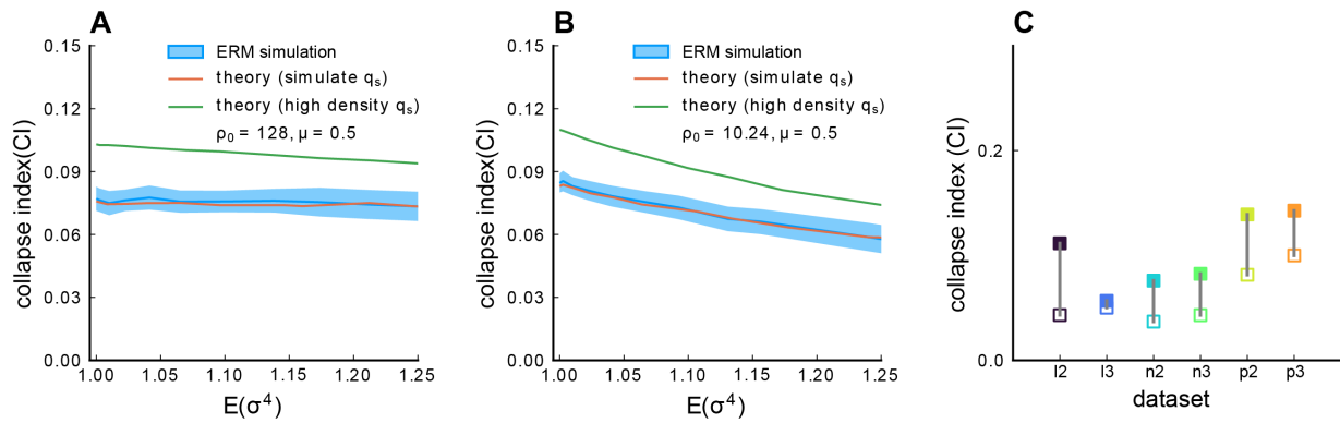
Figure S6. Impact of heterogeneous activity levels on the scale invariance. A. The CI as a function of the heterogeneity of neural activity levels E(\sigma_i^4) . We generate ERM where each neuron's activity variance \sigma_i^2 is i.i.d. sampled from a log-normal distribution where the logarithm of the variable follows a normal distribution with zero mean and a sequence of standard deviation (0, 0.05, 0.1, \dots, 0.5) in the natural logarithm of the values \sigma_i^2 . We also normalize E(\sigma_i^2) = 1 (Methods). The solid blue line is the average across 100 ERM simulations, and the shaded area represents the SD. The red line results from the Gaussian variational method with simulation value integration limit q_s^s . The green line is the result of the Gaussian variational method with high-density value integration limit q_s^h (Methods). \rho_0 = 128 . B. Same as A, but with a smaller \rho_0 = 10.24 . Other parameters: \mu = 0.5 , d = 2 , N = 1024 , L = (N/\rho)^{1/d} , \epsilon = 0.03125 . C. The collapse index (CI) of the correlation matrix (filled symbols) is larger than that of the covariance matrix (open symbols) across different datasets excluding those shown in Fig. 4. We use 7,200 time frame data across all the datasets. l2 to l3: light-sheet zebrafish data (2 Hz per volume); n2 to n3: Neuropixels mouse data, downsampled to 10 Hz per volume, p2 to p3: two-photon mouse data, (3 Hz per volume).
