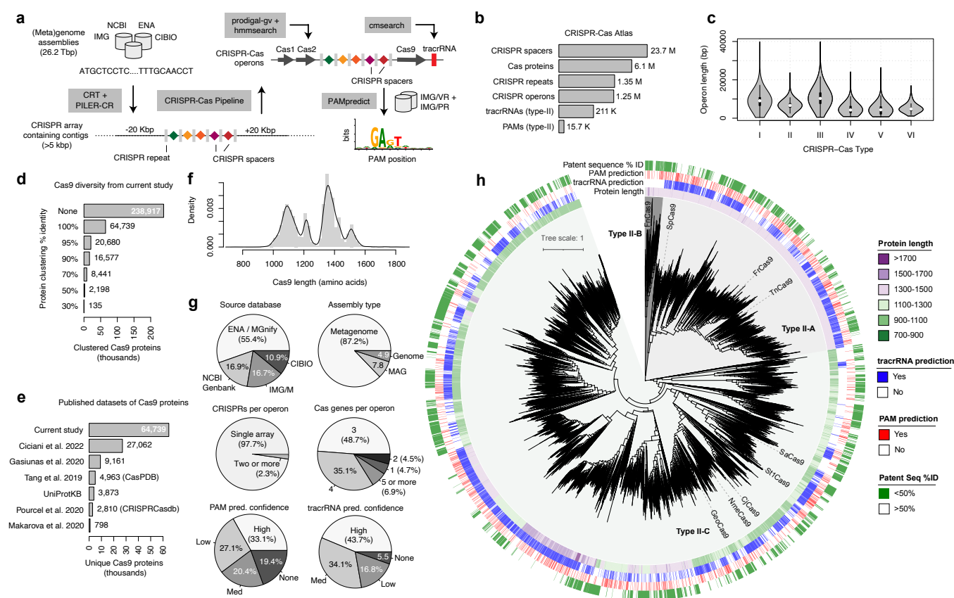
Fig. S1. Formation of the CRISPR-Cas Atlas. a) Pipeline for discovery and annotation of 1.25M CRISPR-Cas operons from 26.2 Tbp of genome and metagenome assemblies. b) Summary of different entities across the CRISPR-Cas atlas. c) Distribution of operon lengths across CRISPR-Cas types. d) 238,917 Cas9 proteins were identified from Type II CRISPR-Cas operons and clustered using MMseqs2. e) Comparison of the number of unique Cas9 proteins compared to previously published datasets (5, 22, 61, 76–78). UniProtKB was queried in March 2024 using search term: gene = Cas9. f) Length of 64,739 unique Cas9 proteins from the CRISPR-Cas Atlas. g) Summary statistics across 64,739 CRISPR-Cas operons. h) Phylogenetic tree of 8,441 Cas9s clustered at 70% identity. Phylogenetic tree built using FastTree2 (69) and visualized using iTOL (70).
