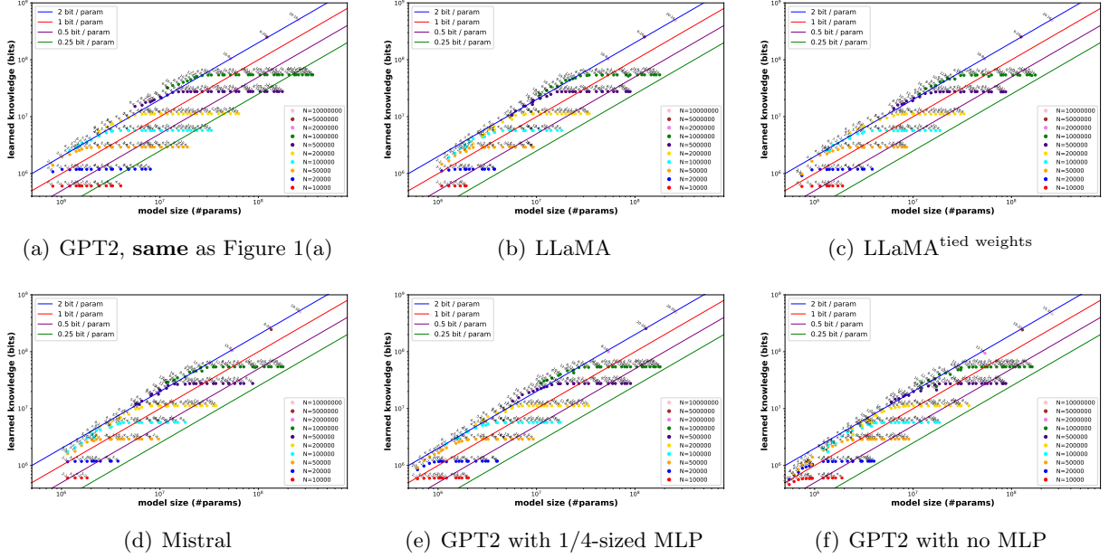
Figure 3: Scaling laws for other model architectures on the bioS( N ) data with 1000 exposures .
