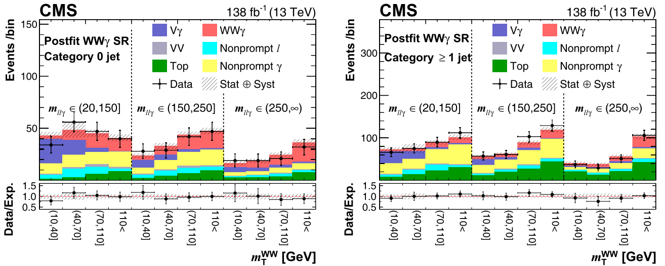
FIG. 3. The unrolled two-dimensional m_T^{WW} - m_{\ell\ell\gamma} distributions in category 0 jet (left) and \geq 1 jet (right) after the fit to data. The data are compared with the sum of the signal and expected background. The black points with error bars represent the data and their statistical uncertainties, whereas the hatched bands represent the total uncertainties in the predictions.
