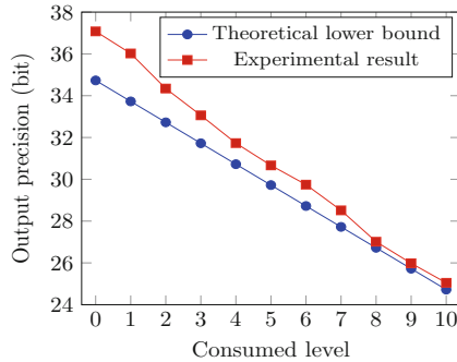
Fig. 1. Bit precision of encrypted plaintext
