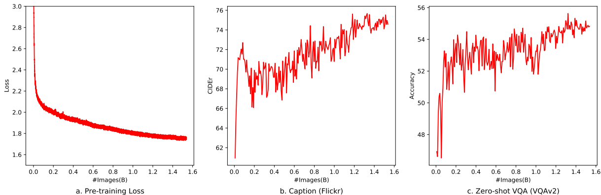
Figure 6: Visualization of the Convergence of the Pre-training Stage
