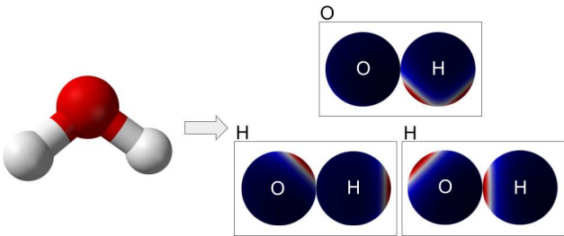
Figure 3. We represent a molecule with a set of Z functions on the sphere for each atom, where Z is the number of atom types in the dataset. Consider the \text{H}_2\text{O} molecule in the figure and let Z = 2 ; the rectangles show the two channels for each atom. The values on the sphere come from physically-based interactions between pairs of atoms, smoothed with a Gaussian kernel, and aggregated over atom types. For example, the sphere marked with an H on the top right sums up the Coulomb forces between the oxygen the two hydrogen atoms.
