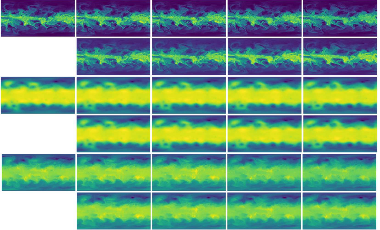
Figure 4. One day rollout of a few predictions of our model. Top two rows: specific humidity at 850 hPa (Q850). Middle two rows: geopotential height at 500 hPa (Z500). Bottom two rows: temperature at 850 hPa (T500). The first column shows the input values at t = 0 , and subsequent columns shows 6 h steps. On each group of two rows, the top shows the ground truth and the bottom one shows our predictions. Our predictions show that large spherical CNNs are capable of producing high resolution outputs with high frequency details.
