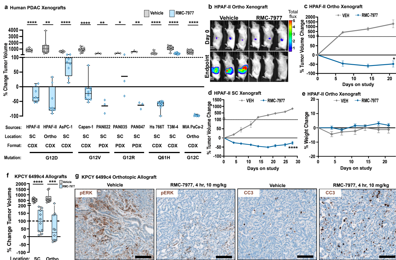
Fig 2. RMC-7977 exhibits anti-tumor activity in xenograft and allograft models of PDAC. (a-e) Human PDAC xenograft models implanted either subcutaneously (SC) or orthotopically (Ortho) into immunodeficient mice. Tumor-bearing mice were treated with Vehicle or RMC-7977 (10 mg/kg, po, q.d.; n=3-10) for 21-28 days. (a) Boxplot showing percent change in tumor volumes at endpoint compared with baseline at Day 0 in Vehicle and RMC-7977 treatment arms. Each symbol represents one mouse. Source and format of each cell line, KRAS mutation, and tumor locations are indicated in the graph. Study arms were compared by Student's unpaired t-test (*, p<0.05; **, p<0.01; ****, p<0.0001). (b) Representative bioluminescence images showing signal in HPAF-II orthotopic xenograft tumors at Day 0 and at Day 21 for Vehicle and RMC-7977 treatment arms. (c,d) Representative tumor growth curves for HPAF-II (c) orthotopic and (d) subcutaneous xenograft models treated with Vehicle or RMC-7977 (n=8/group), shown as percent tumor volume change from baseline over the course of treatment. Vehicle and RMC-7977 groups were compared by 2-way repeated measures ANOVA on the last measurement day of the vehicle group (*, p<0.05; ****p<0.0001). Error bars indicate \pm s.e.m. (e) Tolerability of RMC-7977 as assessed by percent animal body weight change from baseline over the course of treatment. Error bars indicate \pm s.e.m. (f,g) KPCY-derived PDAC cell line (6499c4) was transplanted either subcutaneously or orthotopically into syngeneic mice. Tumor-bearing mice were treated with Vehicle or RMC-7977 (10 mg/kg, po, q.d.; n=9-10/group). (f) Boxplot showing changes in subcutaneous and orthotopic tumor volumes at Day 14, compared with baseline at Day 0, in Vehicle and RMC-7977 treatment arms. Groups compared by Student's unpaired t-test (***, p<0.001; ****, p<0.0001). Tumor locations as indicated in the graph. (g) Representative IHC images of Vehicle and RMC-7977-treated KPCY allograft tumors stained for phospho-ERK T202/204 and CC3. Scale bars = 100 \mu m.
