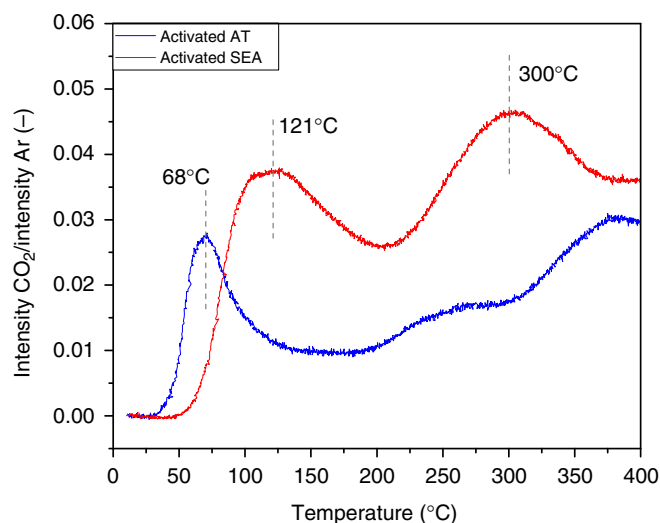
Fig. 4 CO-TPR of the 1wt.%Pt/ \text{CeO}_2 catalysts. The reducibility of the catalysts synthesized by AT and SEA methods was monitored by observing the formation of \text{CO}_2 . Both catalysts were synthesized using TAPN as precursor and were activated prior to the experiment
