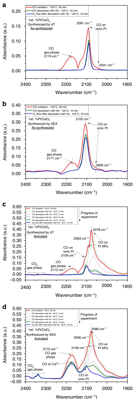
Fig. 3 CO oxidation reaction monitored by DRIFTS on the 1wt% Pt/ \text{CeO}_2 TAPN catalysts: a as-synthesized AT ( 125^\circ\text{C} ), b as-synthesized SEA (at 125^\circ\text{C} ), c activated AT ( 50^\circ\text{C} ), d activated SEA ( 50^\circ\text{C} )
