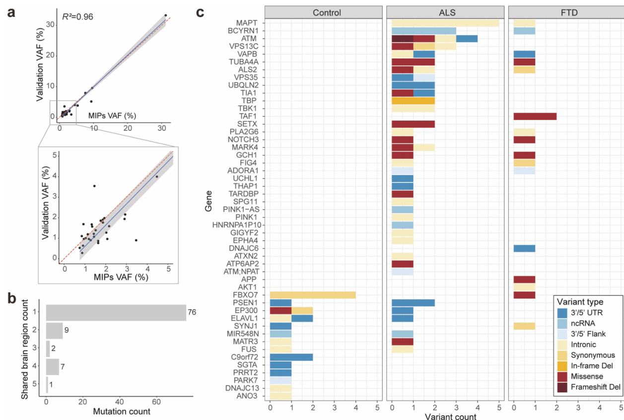
Fig. 3: Somatic variants in MIP sequencing data tend to be focal, protein-altering and are almost exclusively restricted to disease cases. (a) The observed VAFs of somatic variants in amplicon sequencing validation were consistent with the VAFs in original MIP sequencing. Forty somatic variants were validated and included in the plot. (b) Total somatic variant counts classified by the number of brain regions in which a given variant was identified. (c) Distribution of somatic variants in all neurodegenerative genes. Color codes indicate variant types. Note that somatic variants identified in controls are unlikely to alter function, with just one missense mutation (red) and the remaining being synonymous or noncoding substitutions.
