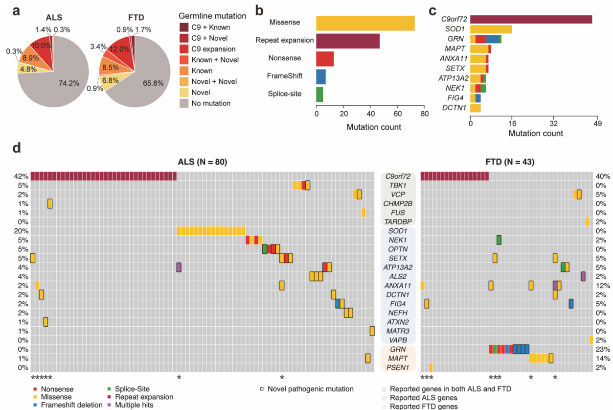
Fig. 2: C9ORF72 repeat expansion and pathogenic germline variants in ALS/FTD genes are prevalent in ALS and FTD. (a) Proportions of ALS and FTD cases with C9ORF72 repeat expansion, known, and novel pathogenic germline variants of ALS/FTD genes. Cases with multiple pathogenic mutations are indicated with '+' sign. (b) Distribution of C9ORF72 repeat expansion and known and novel pathogenic germline variants in ALS/FTD genes classified by mutation types. (c) Ranking of the top 10 mutated ALS/FTD genes. (d) Visualization of ALS and FTD cases (vertical columns) with known and novel pathogenic germline variants (horizontal rows) in ALS/FTD genes. Color codes indicate the types of mutations. Rectangular outline represents novel variants. Genes are grouped by their known involvement in the diseases. * indicates cases with multiple pathogenic mutations.
