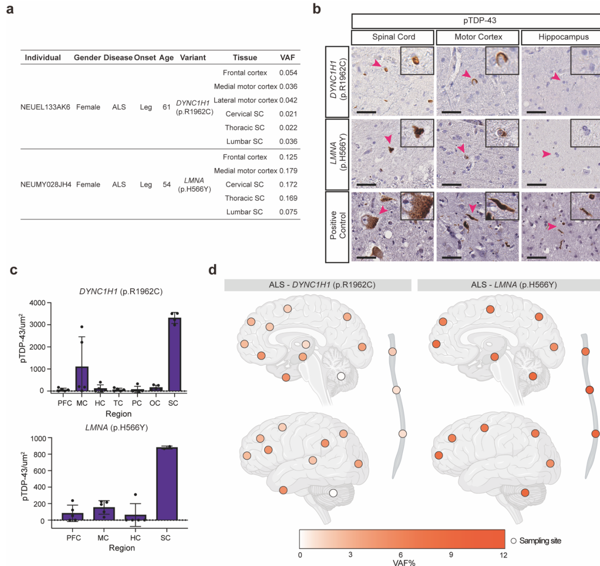
Fig. 6: Somatic variants in DYNC1H1 and LMNA in sALS. (a) Two pathogenic somatic SNVs that were shared by multiple tissue regions of the ALS cases. (b) Sections of the lumbar spinal cord, motor cortex, and hippocampus of the two sALS cases stained with a phospho-TDP43 antibody. Scale bar = 40 \mu m. Arrowheads indicate the cells shown in the insets, which are magnified to twice their original size. (c) Quantification of phospho-TDP43 staining of CNS tissue sections of the two sALS cases with DYNC1H1 and LMNA somatic mutations. Error bars indicate SD (n = 5). PFC: prefrontal cortex. MC: primary motor cortex. HC: hippocampus. TC: temporal cortex. PC: parietal cortex. OC: Occipital cortex. SC: spinal cord. (d) Regional distribution of VAFs of somatic variants in individual brains and spinal cords. Brain cortex is annotated by Brodmann areas. The color spectrum indicates the VAFs of somatic variants in amplicon sequencing. Dots indicate unavailable regions and white indicates regions without the somatic variants.
