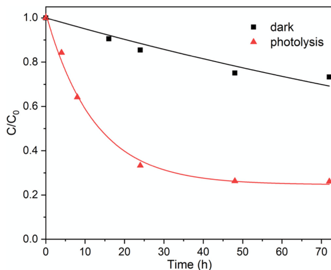
Fig. 6. Maprotiline ( 10 \mu\text{g/L} ) removal over time in a river water sample, in the dark and under UVA irradiation.
