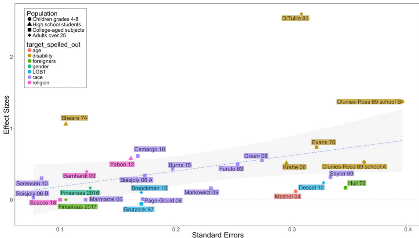
Figure 1. Standard error and effect size (Glass's \Delta ) of each experimental comparison. Colors of points and of labels correspond to target of intervention; shapes of plotted points correspond to population. Fitted line is ordinary least squares and gray bands are 95% confidence intervals. Boisjoly 'A' and 'B' refer, respectively, to effects associated with having black or 'other minority roommates'
