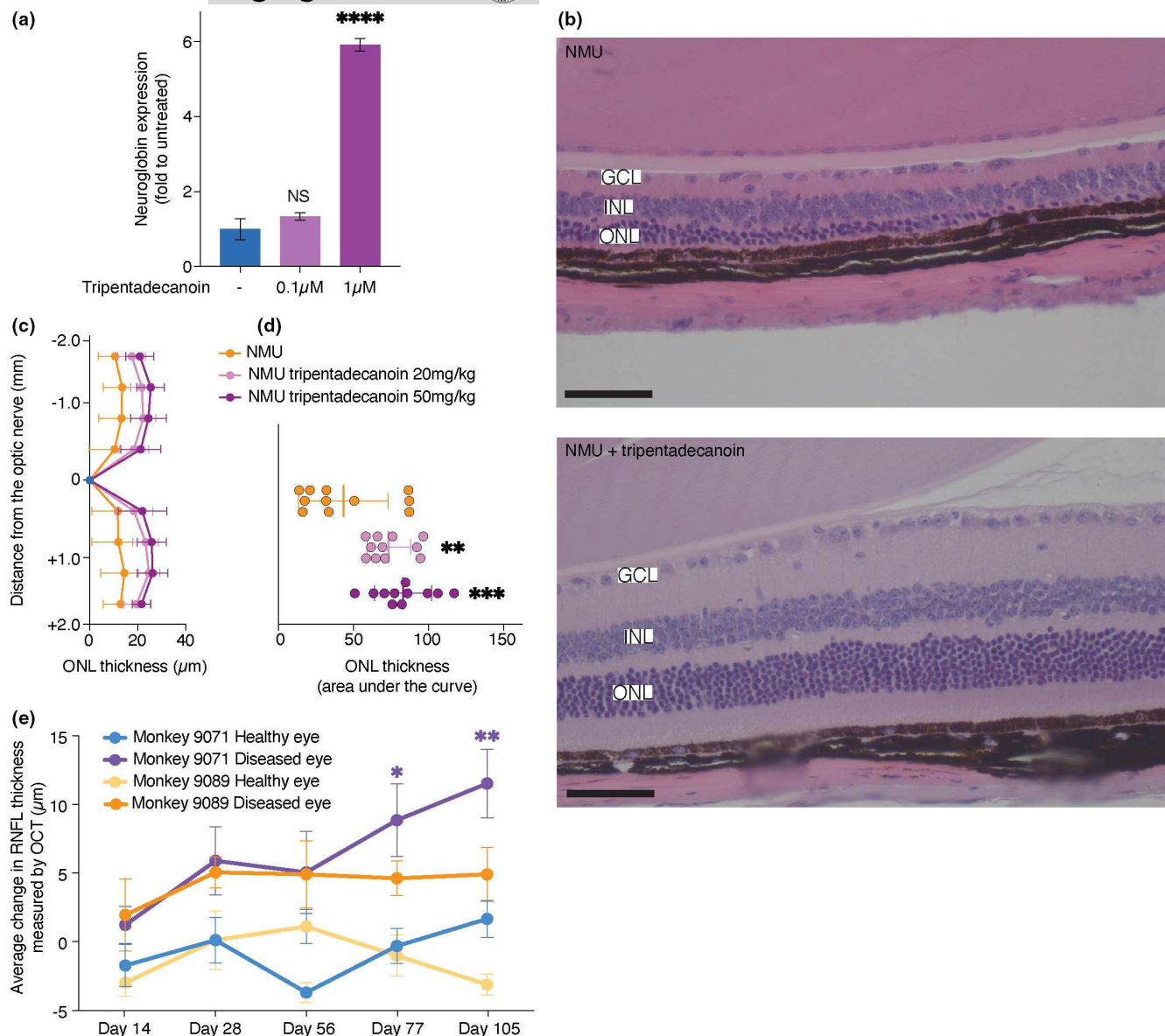
FIGURE 4 Tripentadecanoin induces neuroglobin expression in mouse primary cortex neurons and rescues N-nitroso-N-methylurea (NMU)-induced photoreceptor damage in mice. (a) Expression of neuroglobin mRNA over the control Rps28 mRNA presented as fold increase over untreated cells. p values are adjusted p values from an ANOVA comparing to untreated cells. **** <0.0001 (b) haematoxylin- and eosin-stained retinal sections of eyes from mice treated with NMU (top) or NMU + Tripentadecanoin (bottom). ONL: Outer nuclear layer, INL: Inner nuclear layer, GCL: Ganglion cell layer. Scale bar = 50 μm (c) outer nuclear layer thickness measured from the retina sections as a function of the distance to the optical nerve (mm). Mean \pm SD are presented. (d) Outer nuclear layer thickness presented as the area under the curve from panel c. p values are adjusted p values from an ANOVA comparing to NMU-treated cells. ** <0.005 ; *** <0.001 ; **** <0.0001 . (e) Average change of retinal nerve fibre layer measured by OCT in monkeys #9071 and #9089 treated with tripentadecanoin. In each case, the left healthy eye and right diseased eye were measured. Averages within an eye were compared to the data before treatment with an ANOVA. * <0.05 , ** <0.005
