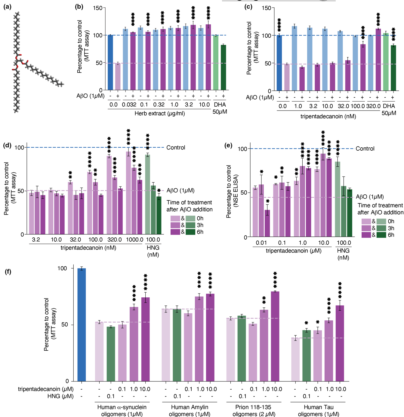
FIGURE 1 Ophioglossum whole extract and tripentadecanoin protect neurons against amyloid toxicity. (a) Structure of tripentadecanoin. (b–c) quantification of mouse primary cortex neurons viability (MTT assay) after exposure to AβO (1 μM) and pre-treatment with Ophioglossum extract or docosahexaenoic acid (DHA) (b) or pre-treatment with tripentadecanoin or DHA (c). (d) Quantification of mouse primary cortex neurons viability (MTT assay) after treatment with tripentadecanoin or Humanin (HNG) 0, 3 or 6 h after exposure to AβO (1 μM). (e) Quantification of human-induced pluripotent stem cells derived neurons viability (NSE assay) after treatment with tripentadecanoin or HNG 0, 3 or 6 h after exposure to AβO (1 μM). (f) Quantification of mouse primary cortex neurons viability (MTT assay) after treatment with tripentadecanoin or HNG 3 h after exposure to human α-synuclein oligomers (1 μM), human amylin oligomers (1 μM), prion Protein 118-135 oligomers (2 μM) or human tau oligomers (1 μM). p-values were obtained from ANOVA comparing to the toxin only treatment (A–E); * < 0.05; ** < 0.01; *** < 0.001; **** < 0.0001
