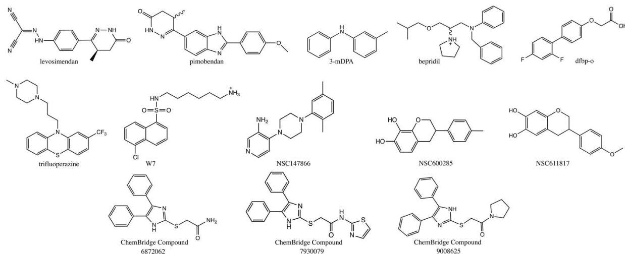
Figure 1. 2D structure of known cNTnC \text{Ca}^{2+} sensitivity modulators.
