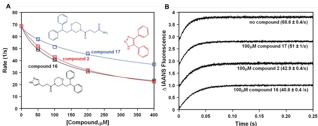
Figure 4. Effect of the hit compounds on the Ca^{2+} dissociation rate from the chimera. Panel (A) shows the plot of the apparent rates of Ca^{2+} dissociation from the chimera in the presence of increased concentration of compounds 2, 16 or 17. Each data point represents an average of at least three measurements \pm standard error. Data were fit with an asymmetric sigmoid curve. Panel (B) shows representative stopped-flow traces as Ca^{2+} is removed from the chimera in the absence or presence of 100 \mu M of compounds 2, 16 or 17. The traces have been normalized and staggered for clarity.
