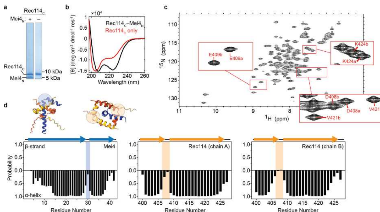
Fig. 2: Spectroscopic analysis of Rec114c complexes with Mei4N. (a) SDS-PAGE of purified proteins. (b) CD spectra for Rec114c with or without co-expressed Mei4N. (c) Two-dimensional \{^1\text{H}-^{15}\text{N}\} HSQC spectrum of Rec114c-Mei4N complexes. Insets show examples of distinct peaks assigned to cognate residues from the two Rec114c chains. (d) TALOS-N secondary structure analysis confirming helix-turn-helix segments in Rec114c and Mei4N. The arrows above the plots show positions of helices predicted by AlphaFold2. Shaded regions are the turns highlighted in the AlphaFold2 model (insets).
