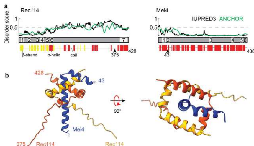
Fig. 1: Structural prediction for trimers of Rec114c and Mei4N. (a) Sequence-based secondary structure and disorder predictions (Methods) suggest that the C terminus of Rec114 and N terminus of Mei4 are ordered and primarily \alpha -helical. Numbered segments are the SSMs from Kumar et al. (2010). (b) AlphaFold2 structure prediction for a heterotrimer of Rec114c and Mei4N.
