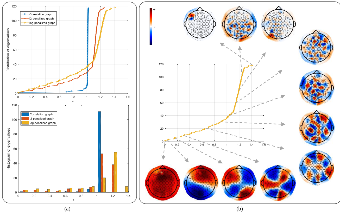
Fig. 3. a) Distribution and histogram of eigenvalues in the log-penalized, l_2 -penalized, and correlation graphs for subject aa . b) Eigenvectors and some of the corresponding eigenvalues of the log-penalized graph.
