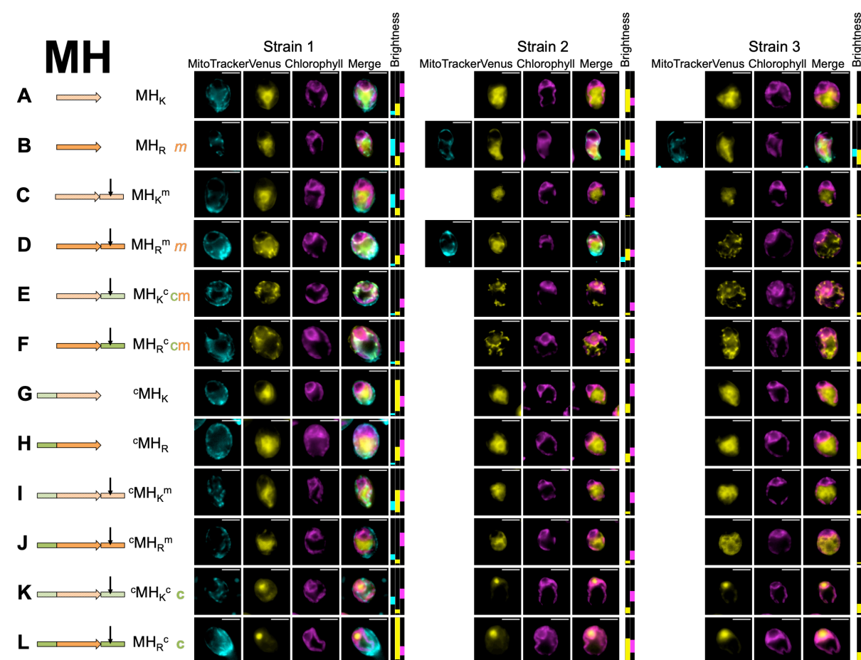
Fig. S18. Microscopy for biological replicates of TP control mitochondrial \gamma -carbonic anhydrase 2 mTP helical element (MH). Three independent transformant lines (Strains 1-3) are shown for each combination of modifications (A-L), represented by a cartoon and a shorthand description (cf. Fig. 2). Where a construct was interpreted as generating reporter localization in mitochondria or chloroplast, this is indicated by an orange ‘m’ or a green ‘c’ respectively in bold for full targeting or in italics for partial targeting. Scale bars are 5 \mu m.
