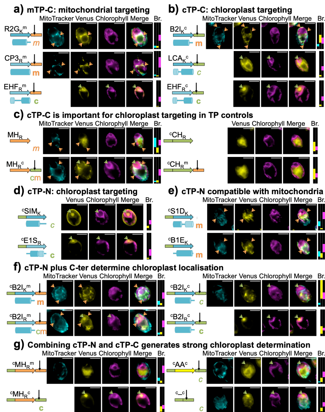
Fig. 4. TP N- and C-termini enable chloroplast targeting by HA-RAMPs.
