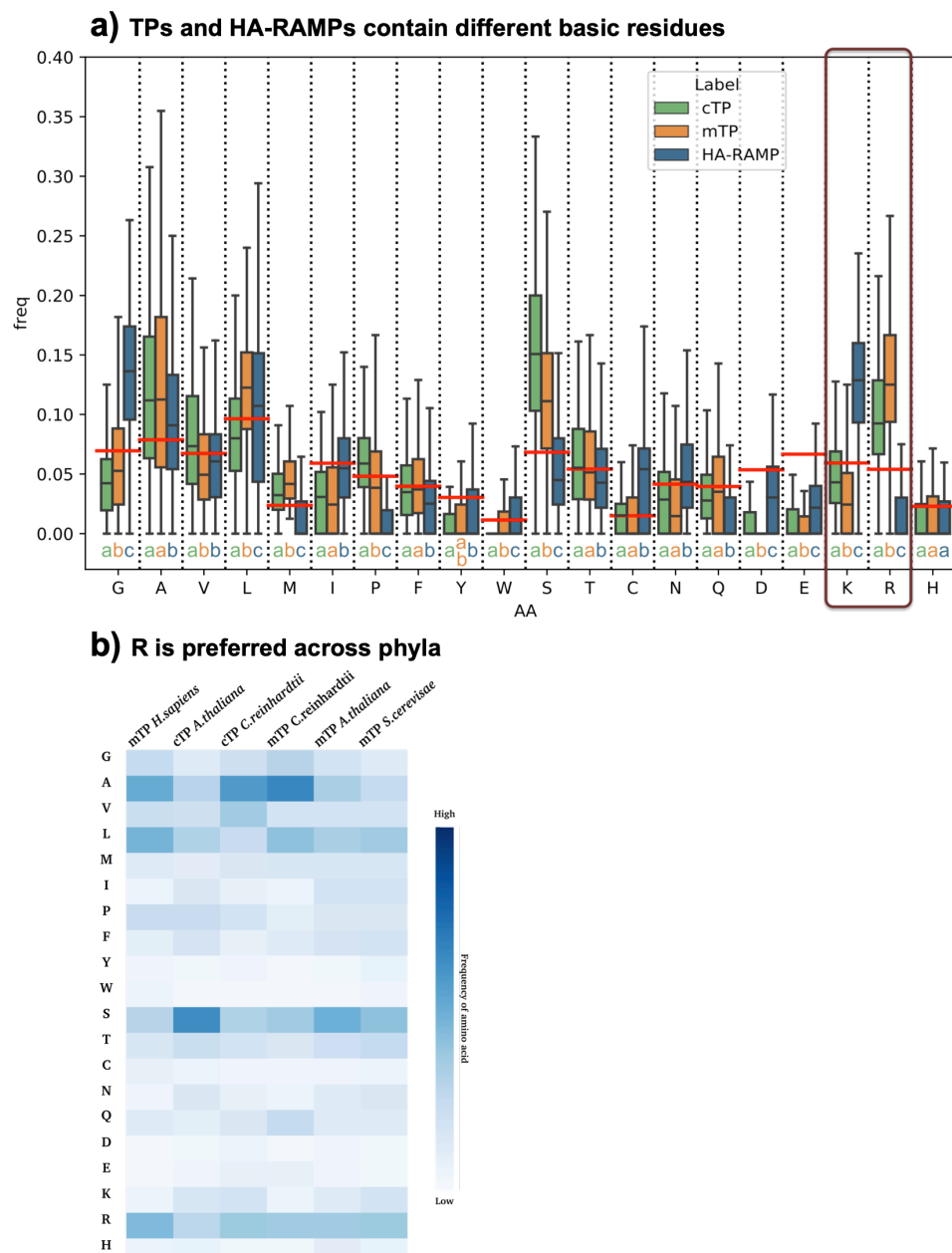
Fig. S20. Comparison of amino acid frequencies reveals K/R shift. (a) Amino acid frequencies are shown as boxplots (center line: median; box limits: upper and lower quartiles; whiskers: min/max values within 1.5x interquartile range) for Chlamydomonas cTPs in green, Chlamydomonas mTPs in orange and HA-RAMPs in blue. To give a baseline for comparison, the average across UNIPROT is given for each amino acid as red horizontal line. For each residue, different letters underneath distributions indicate a significant difference: groups that share the same letter are significantly different at p < 0.05 (Multiple Kruskal Wallis tests followed by Dunn post-hoc tests) from groups attributed a different letter. (b) Amino acid frequencies are shown as heatmap for human, plant, algal and yeast TP.
