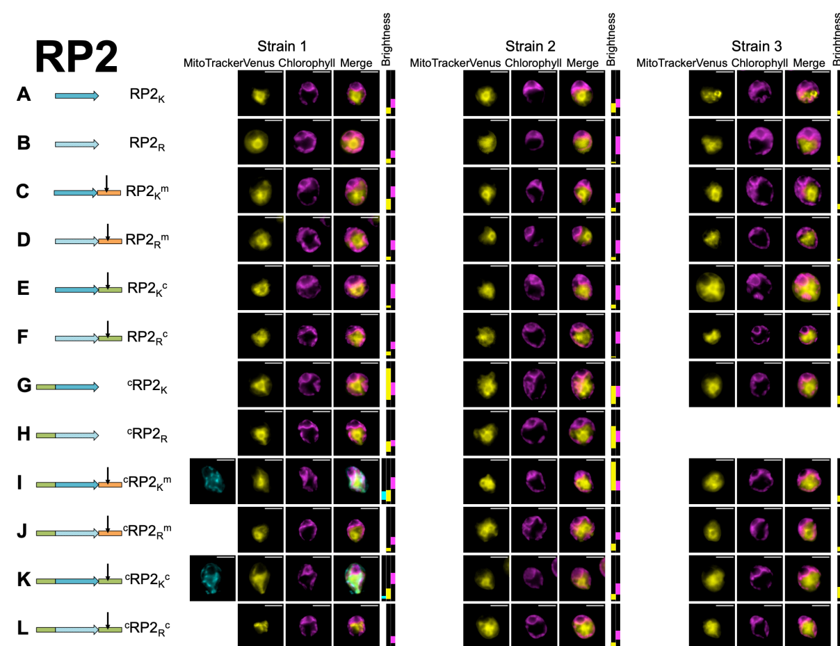
Fig. S16. Microscopy for biological replicates of negative control Random Peptide 2. Three independent transformant lines (Strains 1-3) are shown for each combination of modifications (A-L), represented by a cartoon and a shorthand description (cf. Fig. 2). Where a construct was interpreted as generating reporter localization in mitochondria or chloroplast, this is indicated by an orange ‘m’ or a green ‘c’ respectively, in bold for full targeting or in italics for partial targeting. Scale bars are 5µm.
