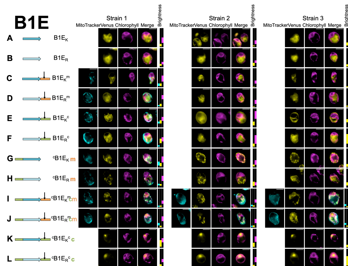
Fig. S5. Microscopy for biological replicates of Brevinin 1E. Three independent transformant lines (Strains 1-3) are shown for each combination of modifications (A-L), represented by a cartoon and a shorthand description (cf. Fig. 2). Where a construct was interpreted as generating reporter localization in mitochondria or chloroplast, this is indicated by an orange ‘m’ or a green ‘c’ respectively, in bold for full targeting or in italics for partial targeting. Scale bars are 5µm.
