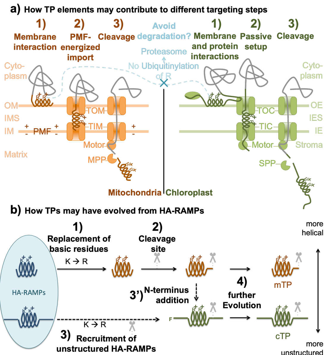
Fig. 7. Proposed functioning and evolution of TPs. Abbreviations: OM – outer membrane, IMS – inter-membrane space, IM – inner membrane, OE – outer envelope, IES – inter-envelope space, IE – inner envelope, PMF – proton motive force, TOM – translocon of the outer mitochondrial membrane, TIM – translocon of the inner mitochondrial membrane, TOC – translocon of the outer chloroplast envelope, TIC – translocon of the inner chloroplast envelope, MPP – matrix processing peptidase, SPP – stromal processing peptidase, R – Arginine, K – Lysine, F – Phenylalanine, mTP – mitochondrial targeting peptide, cTP – chloroplast transit peptide. (a) A number of roles for TP elements during protein import are suggested. Since ubiquitinylation targets K residues, a preference for R in TPs may increase preprotein stability. R may also play a role in lipid interactions. (1) membrane
