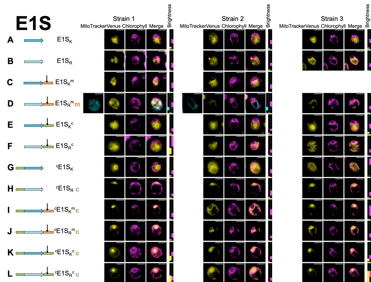
Fig. S10. Microscopy for biological replicates of Esculentin 1S. Three independent transformant lines (Strains 1-3) are shown for each combination of modifications (A-L), represented by a cartoon and a shorthand description (cf. Fig. 2). Where a construct was interpreted as generating reporter localization in mitochondria or chloroplast, this is indicated by an orange ‘m’ or a green ‘c’ respectively, in bold for full targeting or in italics for partial targeting. Scale bars are 5µm.
