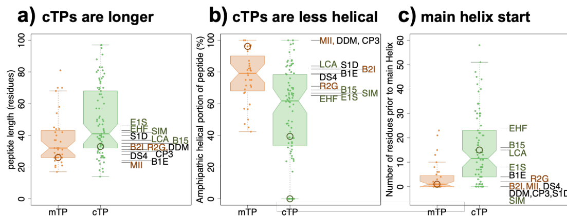
Fig. 5. Chloroplast and mitochondrial targeting HA-RAMPs match cTPs and mTPs respectively. For salient properties, Chlamydomonas mTPs and cTPs are compared to our 13 HA-RAMPs. TP distributions are shown as boxplots (center line: median; box limits: upper and lower quartiles; whiskers: min/max values within 1.5x interquartile range), coloured points represent individual peptides. The position of the CAG2-mTP and RBCA-cTP is circled in each graph. The non-zero value for RBCA-cTP in (B) and the single circle in (C) report on the amphipathic helix established by an NMR-study 16 , since no helix could be predicted by our approach. HA-RAMPs are colour-coded by preferred targeting: orange = mt-set; green = cp-set (cf. Fig. 2). (a) cTPs are significantly longer than mTPs ( p=0.0017 ), and cp-set are longer than mt-set HA-RAMPs ( p=0.0184 ). (b) Helices make up a significantly smaller fraction of cTPs than mTPs ( p<0.0001 ), and HA-RAMPs show a similar trend (0.1122). (c) cTPs contain significantly longer sequence stretches upstream of the longest predicted helix than mTPs ( p<0.0001 ), as do cp-set compared to mt-set HA-RAMPs ( p=0.0205 ). Reported p -values were obtained through two-way t -tests for TPs and one-way t -tests for HA-RAMPs.
