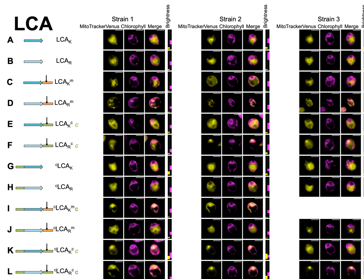
Fig. S11. Microscopy for biological replicates of Leucocin A. Three independent transformant lines (Strains 1-3) are shown for each combination of modifications (A-L), represented by a cartoon and a shorthand description (cf. Fig. 2). Where a construct was interpreted as generating reporter localization in mitochondria or chloroplast, this is indicated by an orange ‘m’ or a green ‘c’ respectively, in bold for full targeting or in italics for partial targeting. Scale bars are 5µm.
