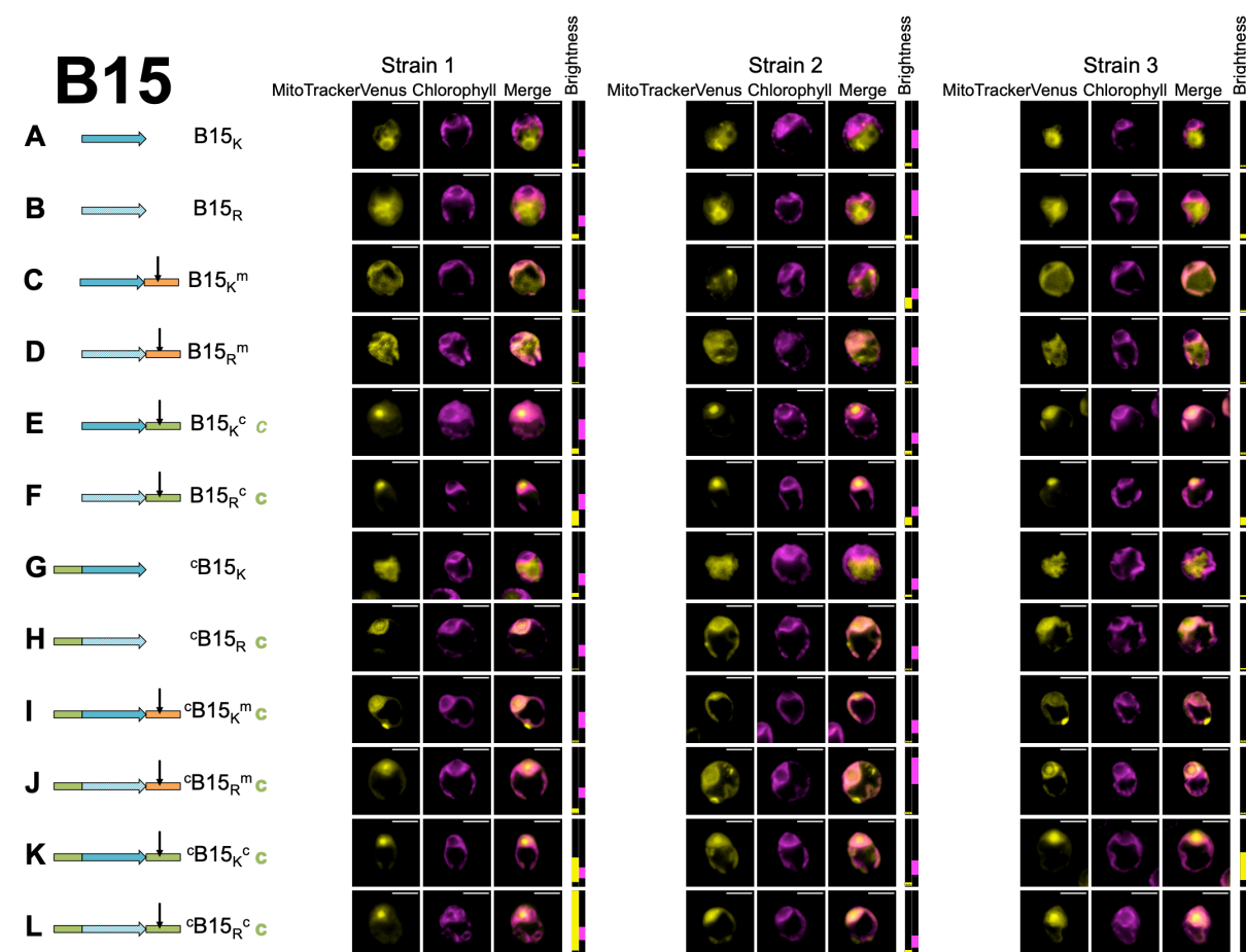
Fig. S13. Microscopy for biological replicates of Bacillocin 1580. Three independent transformant lines (Strains 1-3) are shown for each combination of modifications (A-L), represented by a cartoon and a shorthand description (cf. Fig. 2). Where a construct was interpreted as generating reporter localization in mitochondria or chloroplast, this is indicated by an orange ‘m’ or a green ‘c’ respectively, in bold for full targeting or in italics for partial targeting. Scale bars are 5µm.
