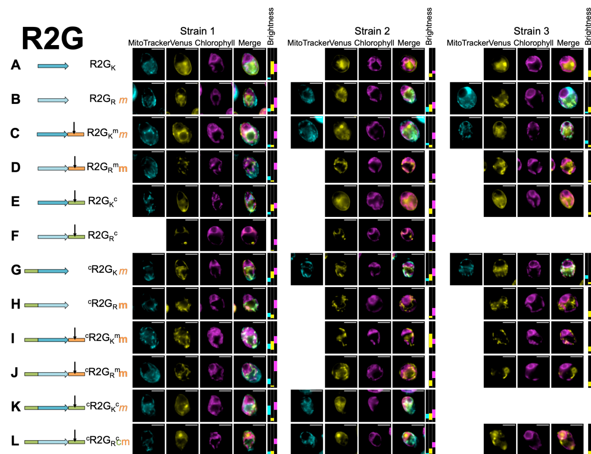
Fig. S4. Microscopy for biological replicates of Ranatuerin 2G. Three independent transformant lines (Strains 1-3) are shown for each combination of modifications (A-L), represented by a cartoon and a shorthand description (cf. Fig. 2). Where a construct was interpreted as generating reporter localization in mitochondria or chloroplast, this is indicated by an orange ‘m’ or a green ‘c’ respectively, in bold for full targeting or in italics for partial targeting. Scale bars are 5µm.
