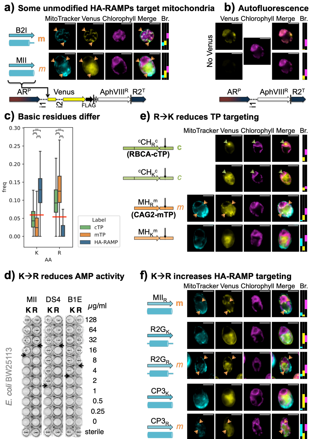
Fig. 3. K is for killing, R is for targeting. (a) Indicated peptides were inserted upstream of a Venus fluorescent protein reporter in a bicistronic expression system for Chlamydomonas 61 . AR P : hybrid HSP70a-RBCS2 promoter, i1: RBCS2 intron 1, i2: RBCS2 intron 2, FLAG: FLAG-tag, |: stop codon, *: bicistronic bridge sequence tagcat, AphVIII R : Paromomycin resistance gene, R2 T : RBCS2 terminator. Epifluorescence microscopy images of selected examples are shown. False-coloured
