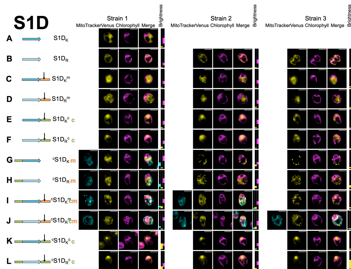
Fig. S9. Microscopy for biological replicates of Sarcotoxin 1D. Three independent transformant lines (Strains 1-3) are shown for each combination of modifications (A-L), represented by a cartoon and a shorthand description (cf. Fig. 2). Where a construct was interpreted as generating reporter localization in mitochondria or chloroplast, this is indicated by an orange ‘m’ or a green ‘c’ respectively, in bold for full targeting or in italics for partial targeting. Scale bars are 5µm.
