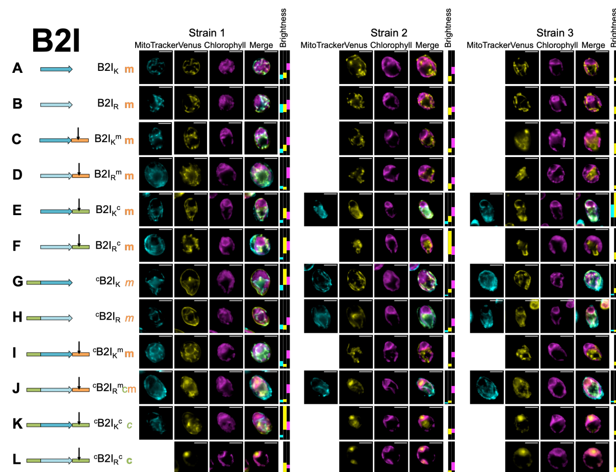
Fig. S2. Microscopy for biological replicates of Brevinin 2ISb. Three independent transformant lines (Strains 1-3) are shown for each combination of modifications (A-L), represented by a cartoon and a shorthand description (cf. Fig. 2). Where a construct was interpreted as generating reporter localization in mitochondria or chloroplast, this is indicated by an orange ‘m’ or a green ‘c’ respectively, in bold for full targeting or in italics for partial targeting. Scale bars are 5μm.
