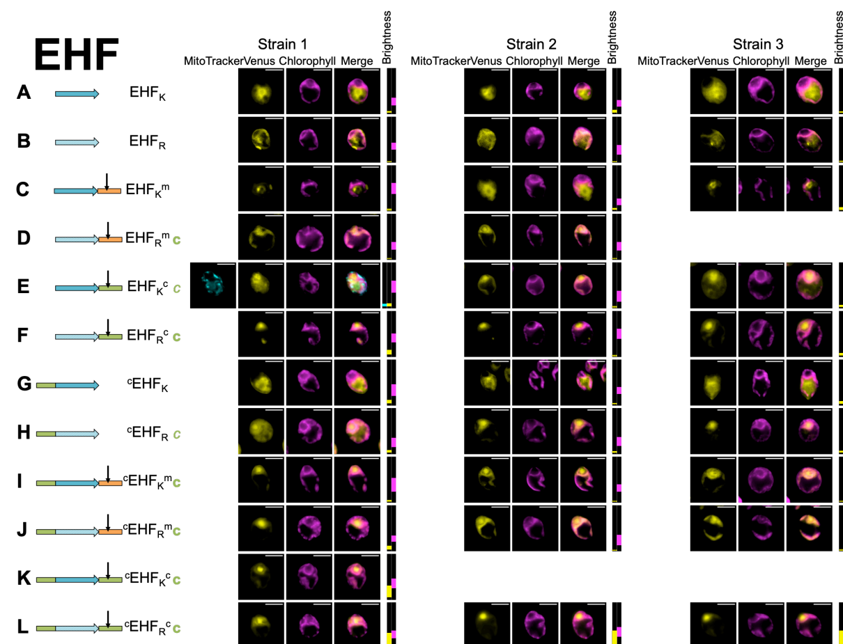
Fig. S14. Microscopy for biological replicates of Enterocin HF. Three independent transformant lines (Strains 1-3) are shown for each combination of modifications (A-L), represented by a cartoon and a shorthand description (cf. Fig. 2). Where a construct was interpreted as generating reporter localization in mitochondria or chloroplast, this is indicated by an orange ‘m’ or a green ‘c’ respectively, in bold for full targeting or in italics for partial targeting. Scale bars are 5µm.
