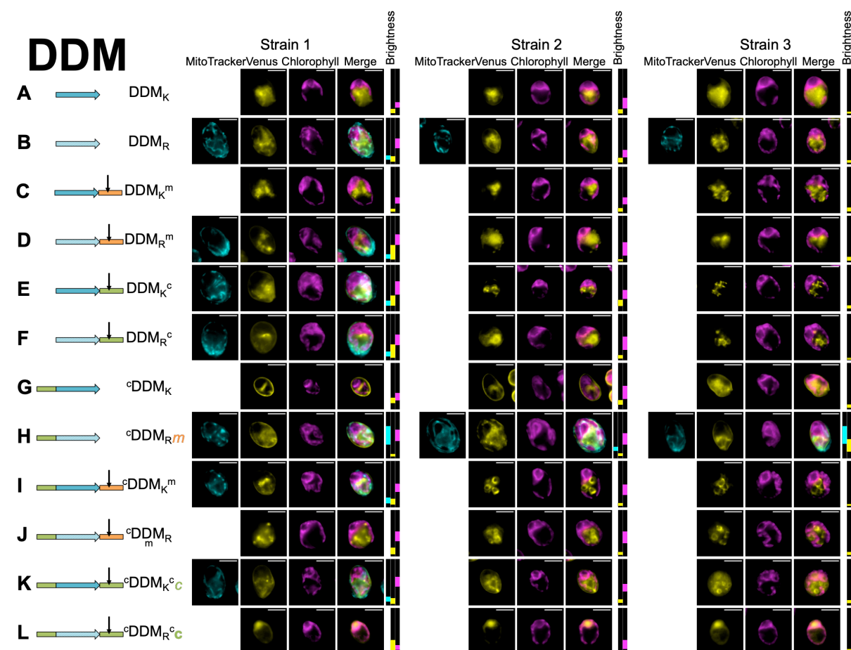
Fig. S7. Microscopy for biological replicates of Dermadistinctin M. Three independent transformant lines (Strains 1-3) are shown for each combination of modifications (A-L), represented by a cartoon and a shorthand description (cf. Fig. 2). Where a construct was interpreted as generating reporter localization in mitochondria or chloroplast, this is indicated by an orange 'm' or a green 'c' respectively, in bold for full targeting or in italics for partial targeting. Scale bars are 5µm.
