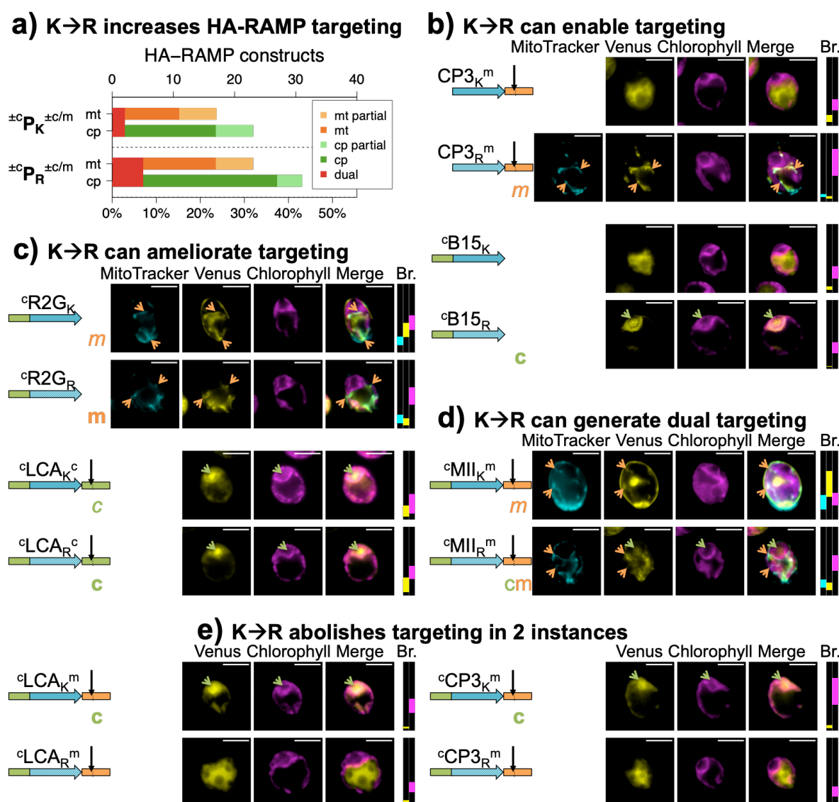
Fig. S23. K→R generally improves HA-RAMP targeting. (a) An overview graph showing how many, out of 13 HA-RAMPs studied, show targeting to either mitochondria (mt) or chloroplast (cp), or both (dual) before and after K→R represented. (b-e) Epifluorescence microscopy images of selected examples are shown as in Fig. 3.
