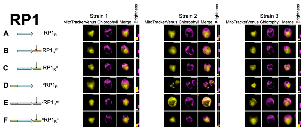
Fig. S15. Microscopy for biological replicates of negative control Random Peptide 1. Three independent transformant lines (Strains 1-3) are shown for each combination of modifications (A-F), represented by a cartoon and a shorthand description (cf. Fig. 2). Where a construct was interpreted as generating reporter localization in mitochondria or chloroplast, this is indicated by an orange ‘m’ or a green ‘c’ respectively, in bold for full targeting or in italics for partial targeting. Scale bars are 5µm.
