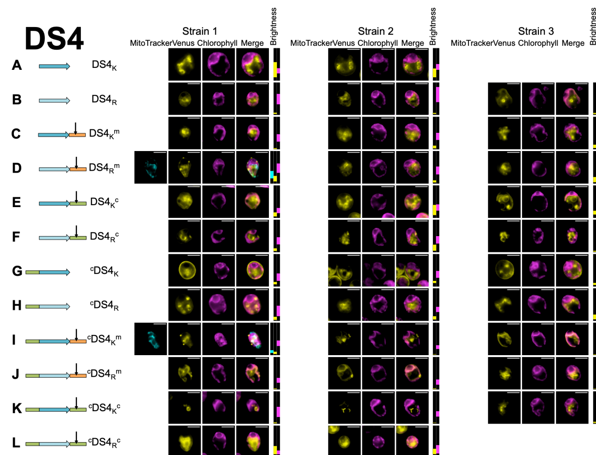
Fig. S6. Microscopy for biological replicates of Dermaseptin S4. Three independent transformant lines (Strains 1-3) are shown for each combination of modifications (A-L), represented by a cartoon and a shorthand description (cf. Fig. 2). Where a construct was interpreted as generating reporter localization in mitochondria or chloroplast, this is indicated by an orange 'm' or a green 'c' respectively, in bold for full targeting or in italics for partial targeting. Scale bars are 5µm.
