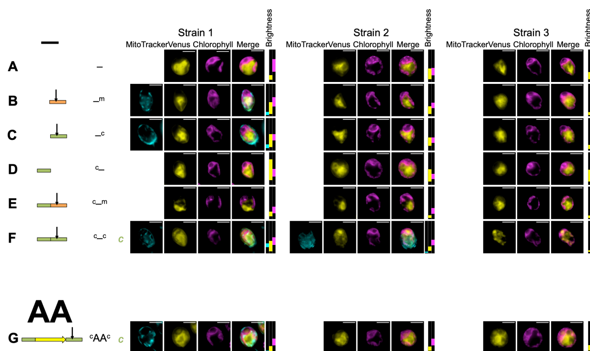
Fig. S19. Microscopy for biological replicates of no-peptide and Alanine-screen controls. Three independent transformant lines (Strains 1-3) are shown for each combination of elements (A-G), represented by a cartoon and a shorthand description (cf. Fig. 2). Where a construct was interpreted as generating reporter localization in mitochondria or chloroplast, this is indicated by an orange ‘m’ or a green ‘c’ respectively, in bold for full targeting or in italics for partial targeting. Scale bars are 5μm.
