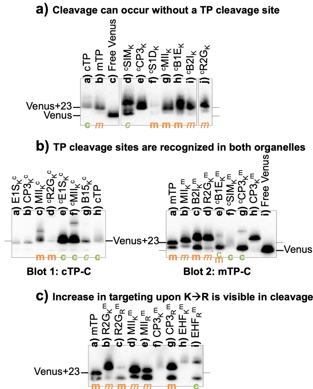
Fig. 6. Import is associated with maturation of the preprotein. Western Blots used an \alpha -FLAG antibody on selected constructs as indicated above blots. Where a construct was interpreted as generating reporter localization by fluorescence microscopy (cf. Fig. 2, Fig. S2-S19) in mitochondria or chloroplast, this is indicated by an orange 'm' or a green 'c' respectively, in bold for full targeting or in italics for partial targeting. In (a) some lanes were spliced for clarity; the uncropped blot is provided in Fig. S27.
