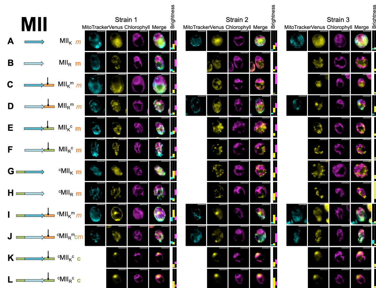
Fig. S3. Microscopy for biological replicates of Magainin 2. Three independent transformant lines (Strains 1-3) are shown for each combination of modifications (A-L), represented by a cartoon and a shorthand description (cf. Fig. 2). Where a construct was interpreted as generating reporter localization in mitochondria or chloroplast, this is indicated by an orange ‘m’ or a green ‘c’ respectively, in bold for full targeting or in italics for partial targeting. Scale bars are 5µm.
