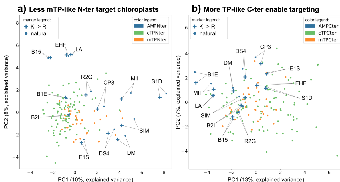
Fig. S21. Principal component analyses reveal that N- but not C-termini differ between cTPs and mTPs. Principal component (PC) analyses of auto-cross-correlated Z-scale values 10 for (a) N-termini (15 residues) and (b) C-termini (33 residues, encompassing -10 to +23 relative to the cleavage site for TP) respectively of Chlamydomonas cTPs (in green) and mTPs (in orange) as well as the 13 HA-RAMPs under study (in blue; crosses denote HA-RAMPs after K→R).
