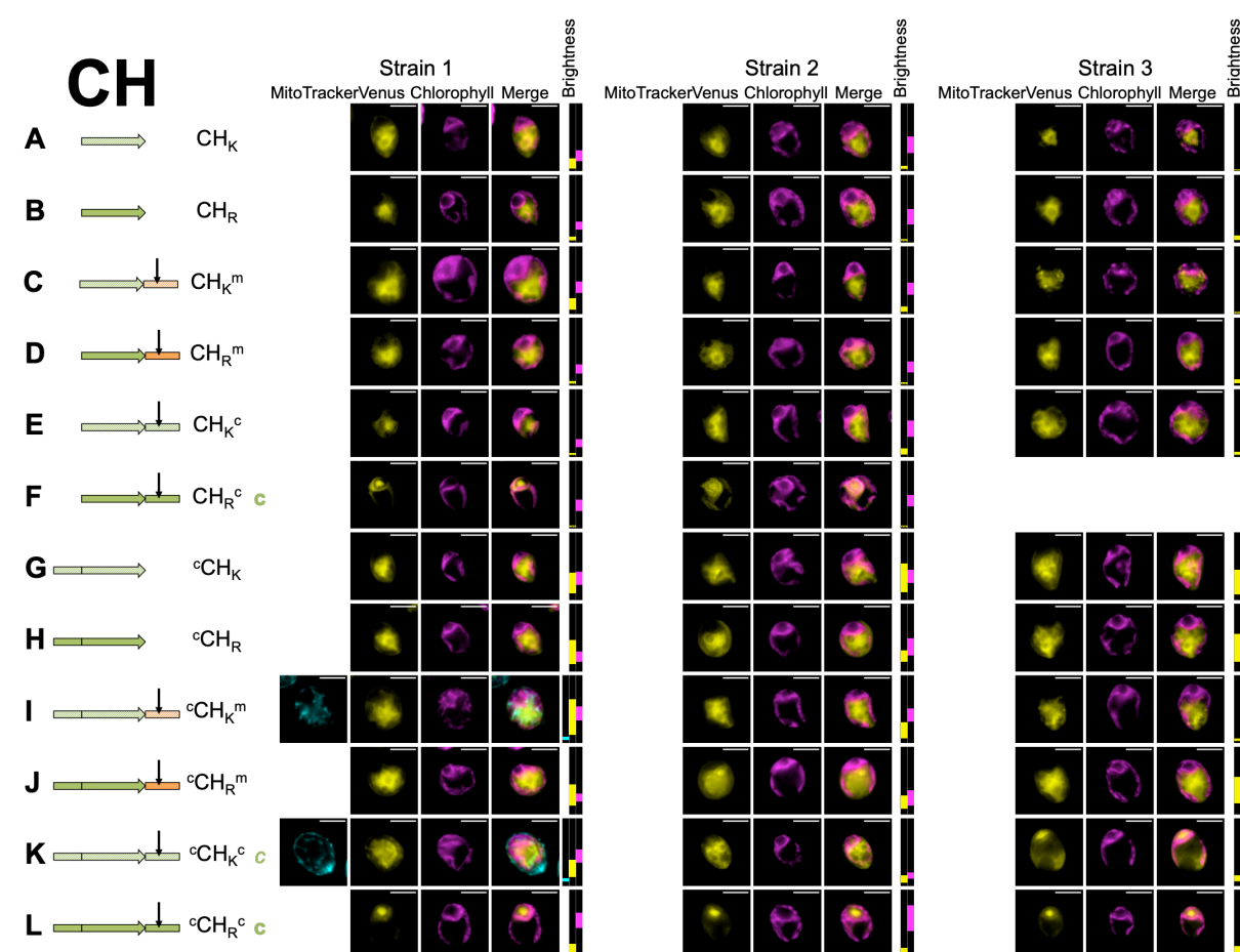
Fig. S17. Microscopy for biological replicates of TP control Rubisco activase cTP helical element (CH). Three independent transformant lines (Strains 1-3) are shown for each combination of modifications (A-L), represented by a cartoon and a shorthand description (cf. Fig. 2). Where a construct was interpreted as generating reporter localization in mitochondria or chloroplast, this is indicated by an orange ‘m’ or a green ‘c’ respectively, in bold for full targeting or in italics for partial targeting. Scale bars are 5µm.
