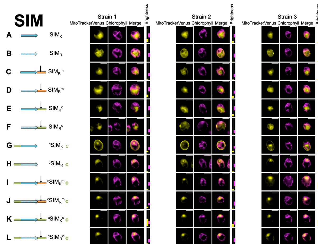
Fig. S12. Microscopy for biological replicates of SI Moricin. Three independent transformant lines (Strains 1-3) are shown for each combination of modifications (A-L), represented by a cartoon and a shorthand description (cf. Fig. 2). Where a construct was interpreted as generating reporter localization in mitochondria or chloroplast, this is indicated by an orange ‘m’ or a green ‘c’ respectively, in bold for full targeting or in italics for partial targeting. Scale bars are 5µm.
