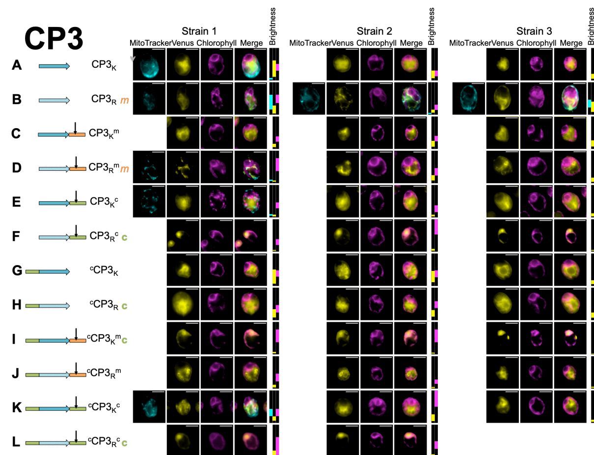
Fig. S8. Microscopy for biological replicates of Cecropin P3. Three independent transformant lines (Strains 1-3) are shown for each combination of modifications (A-L), represented by a cartoon and a shorthand description (cf. Fig. 2). Where a construct was interpreted as generating reporter localization in mitochondria or chloroplast, this is indicated by an orange ‘m’ or a green ‘c’ respectively, in bold for full targeting or in italics for partial targeting. Scale bars are 5µm.
