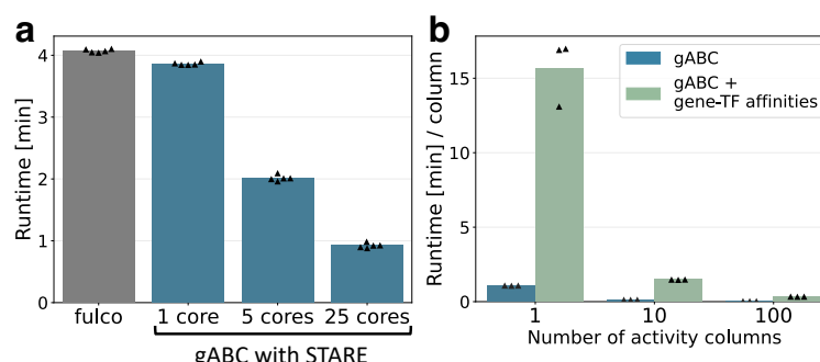
Figure 4. Runtime of the STARE pipeline. (a) Runtime of the original ABC pipeline by (Fulco et al.) and our ABC-scoring implementation with a different number of cores. Any writing of output files was omitted. Calculations were done for K562 cells, scoring 155,976 candidate enhancers for 24,586 genes in a 10 MB window. The bars show the mean of five runs. (b) Runtime divided by the number of activity columns for the ABC-scoring alone and when additionally calculating the gene-TF affinity matrix. Writing and compression of output files is included. Calculations were done on single-cell heart data (Hocker et al., 2021) with 286,777 candidate enhancers, for 55,765 genes in a 5 MB window. 818 TFs were assessed. The bars' height represent the mean of three runs.
