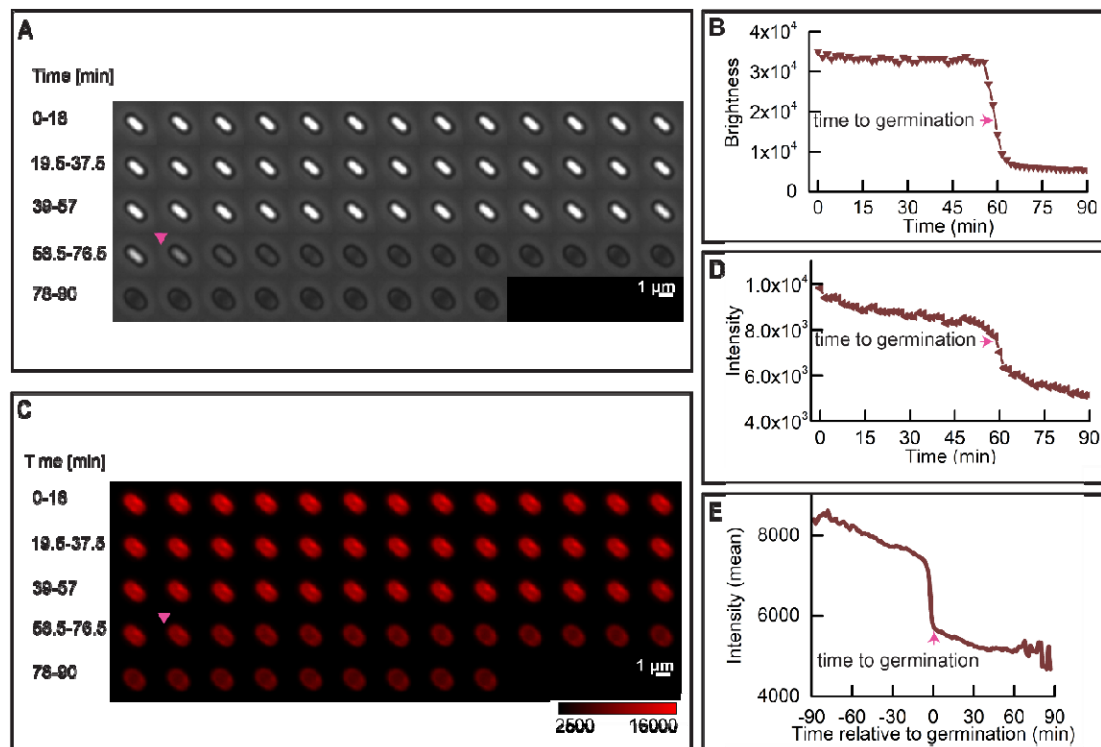
Figure 3. Dynamic behavior of the DiIC 12 stained wild-type spore IM during germination. Spore germination was triggered by (10 mM each) AGFK as described in Methods. (A) Phase brightness of a PS832 (DiIC 12 ) spore. (B) The spore brightness profile corresponding to the images shown in panel A. (C) The fluorescence time lapse images of the same spore shown in panel A. (D) The DiIC 12 stained IM intensity profile corresponding to images in panel C. The magenta arrow indicates the 'time to germination'. (E) Average of 170 synchronized single DiIC 12 spore fluorescence intensity traces. Synchronization defines t=0 min as the 'time to germination'. 289 spores were tracked by microscopy for 90min, and 58.8% of them completed germination.
