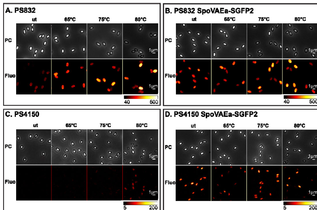
Figure 6. The effect of 5 hours of heat-treatment on PS832 SpoVAEa-SGFP2. The phase contrast (PC) and widefield fluorescence (Fluo) images of spores of wild type strain PS832 (A), PS832 SpoVAEa-SGFP2 spores (B), (C) PS4150, and (D) PS4150 SpoVAEa-SGFP2 after different heat treatments. (A) and (B) are the images corresponding to Fig. 5C-5D. (B) and (C) are the images corresponding to Fig. 5E-5F. The fluorescent image intensity display range for each strain is the same.
