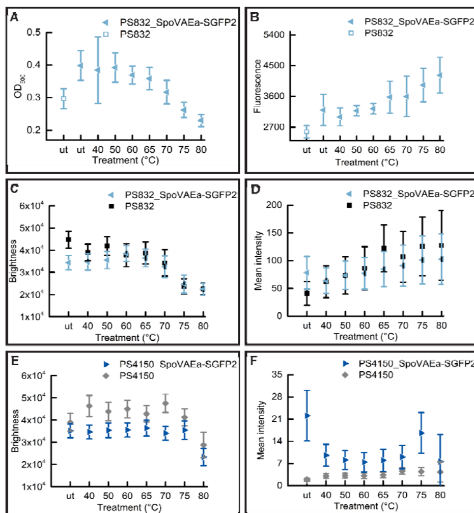
Figure 5. Changes in SpoVAEa-SGFP2 dormant spore refractility and fluorescence intensity at population and single spore levels after 5 hours of heat treatment at various temperatures. (A) The
