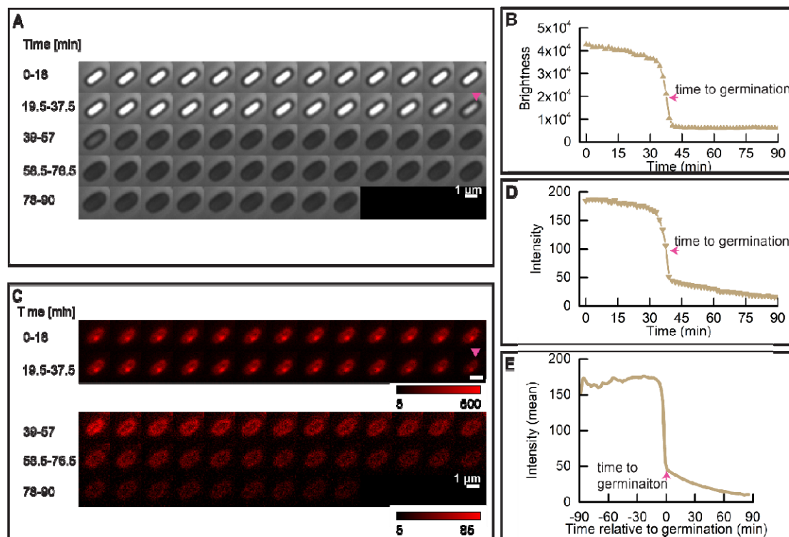
Figure 4. Dynamic behavior of the FM5-95 stained IM during wild-type spore germination. Spore germination was triggered by (10 mM each) AGFK as described in Methods. (A) Phase brightness of a PS832 (FM5-95) spore. (B) The spore brightness profile corresponding to the images shown in panel A. (C) The fluorescence time lapse images of the same spore shown in panel A. (D) The FM5-95 stained IM intensity profile corresponding to images in the panel C. The magenta arrow indicates the 'time to germination'. (E) Average of 277 synchronized single FM5-95 spore fluorescence intensity traces. Synchronization defines t=0 min as the 'time to germination'. 369 spores were tracked by microscope for 90min, and 75.1% of them completed germination.
