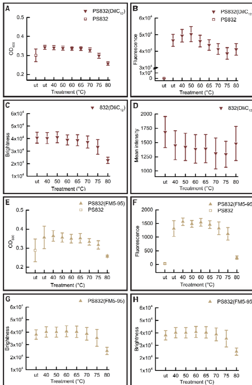
Figure 7. The change of lipid probe stained dormant spore refractility and fluorescence intensity at population and single spore levels after 5 hours of treatment at various temperatures. (A) The change of OD 600 of PS832 (DiIC 12 ) dormant spore populations measured by a plate reader. Untreated PS832 spores were used as control. (B) The corresponding fluorescence intensity of spores in panel A. (C) The change of individual PS832 (DiIC 12 ) spores' brightness measured by a phase contrast microscopy. ≥ 612 spores were examined in each group. (D) The corresponding fluorescence intensity of spores in panel C. (E) The brightness of individual PS832 (FM5-95) dormant spores. ≥ 932 spores were examined in each group. (F) The corresponding fluorescence intensity of spores in panel E. The numbers of individual spores examined by microscopy are given in Table. S2.
