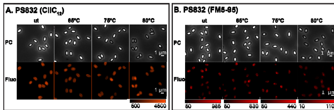
Figure 8. The effect of 5 hours of heat-treatment on the fluorescence intensity of probe stained spores. The phase contrast (PC) and widefield fluorescence (Fluo) images of wild type PS832 spores stained by DiIC 12 (A), and FM5-95 (B) after different heat treatments: (A) images corresponding to Fig. 7C-7D; and (B) images corresponding to Fig. 7G-7H. The fluorescence images displayed for DiIC 12 spores are all in the same range, whereas, the FM5-95 fluorescence images displayed are in different ranges due to the big decline in brightness at higher temperatures.
