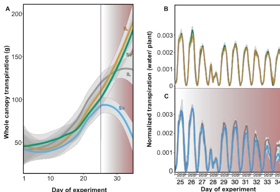
Figure 2. Whole canopy transpiration dynamics of Svevo (Sv) and IL20 (IL) under well-watered (WW) and drought stress (DS) treatments. (A) Daily transpiration dynamics along with the experiment. The increasing drought intensity is represented with the pink background colour intensity. The vertical purple line represents the point that drought stress application started. Hourly dynamics of normalized transpiration rate of Svevo and IL20 under (B) WW and (C) DS. The line curves represent the genotype means ( n=5 ) within water treatment, and shaded colours indicate the standard error.
