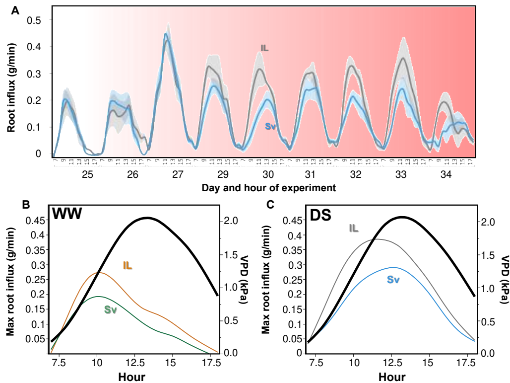
Figure 5. Root influx dynamics of Svevo (Sv) and IL20 (IL) under well-watered (WW) and drought stress (DS) treatments. (A) Hourly root influx dynamics throughout the increasing drought intensity. The increasing drought intensity is represented with the pink background colour intensity. The average maximum hourly root influx was calculated for the last 5 days (30-34) of the experiment under (B) WW and (C) DS treatments. Hourly vapour pressure deficit (VPD) is represented by the black line. The genotype curves represent the means ( n=5 ) within water treatment, day and hour. Shaded colours indicate the standard error.
