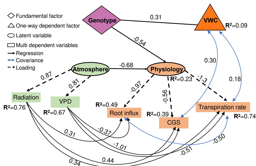
Figure 6. Scheme of the genetic-physiological-atmospheric network path under drought stress. Black and solid one-directional arrows represent standardized parameter estimates for regressions, and dashed arrows represent the loadings standardized parameter estimates. The blue two-directional arrows represent the standardized parameter estimates for covariance and R^2 for the endogenous variables. Only significant paths are presented ( P \leq 0.05 ).
