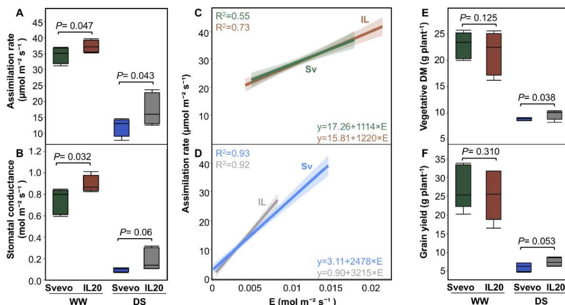
Figure 4. Leaf gas exchange, water-use efficiency and productivity of Svevo (Sv) and IL20 (IL) under well-watered (WW) and drought stress (DS) treatments. (A) Assimilation rate during the booting developmental stage. (B) Stomatal conductance during the booting developmental stage. Seasonal average of leaf water-use efficiency (A/E) under (C) WW and (D) DS treatments. (E) Vegetative dry matter (DM) and (F) grain yield. Differences between genotypes within water treatment were analysed using a t-test ( n=5 ). Genotypic differences in A/E under specific water treatment were obtained by applying a parallelism test.
