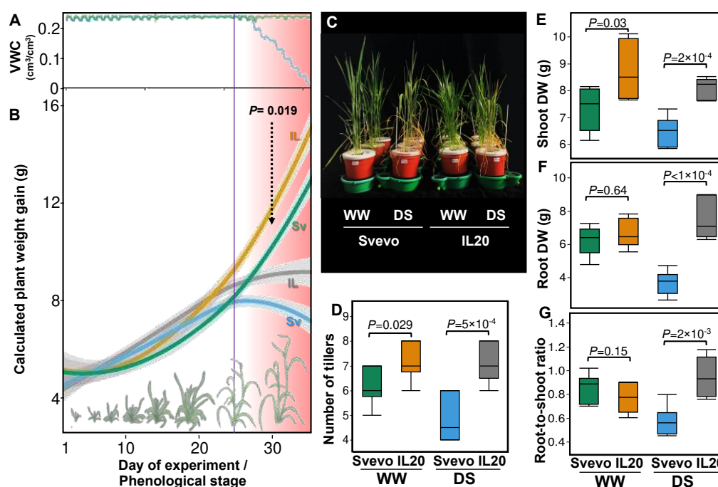
Figure 1. Longitudinal weight gain and its distribution under contrasting water treatments. (A) Volumetric water content (VWC) and (B) calculated weight gain dynamics of Svevo (Sv) and IL20 (IL) under well-watered (WW) and drought stress (DS) treatments along with the different wheat phenological stages. The vertical purple line represents the point that drought stress application started. The increasing stress intensity is represented by the pink background colour intensity. The line curves represent the genotype mean within water treatment and day ( n=5 ). Shaded colours indicate the standard error. (C) Svevo and IL20 under contrasting water treatments on the last day of the experiment. (D) Number of tillers, (E) shoot dry weight (DW), (F) root DW, and (G) root-to-shoot ratio of the two genotypes under contrasting water treatments. Differences between genotypes within water treatment were analysed using a t-test ( n=5 ) on the last day of the experiment (35 days after transplanting).
