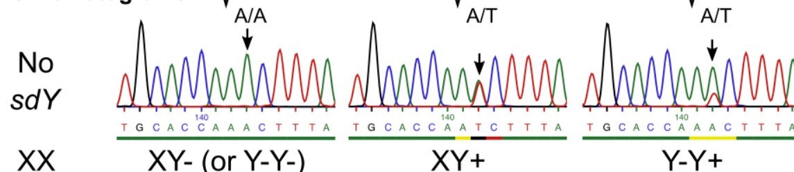
Figure 2. Sex chromosomes, sex genotypes and sex phenotypes in Chinook salmon. (A) Schematic representation of sex chromosomes and the hypothetical relation between sex genotypes and sex phenotypes in Chinook salmon. According to our model, phenotypic females can be normal XX females or XY females (XY-) bearing a Y chromosome (Y-) with a single copy sdY-N183 gene. Phenotypic males can be XY males (XY+) bearing a Y chromosome (Y+) with two copies of the sdY gene i.e., sdY-I183 and sdY-N183 , or Y-Y+ resulting from the crossing of an XY+ male with an XY- female. In turn, a Y-Y+ males crossed with an XY- female can also generate Y-Y- phenotypic females. (B). Representative chromatograms of the sequences around the sdY I183N mutation (exon 3) in Chinook salmon. XY females (XY-) are homozygotes A/A for the I183N mutation and males are heterozygotes (A/T). Y-Y- females cannot be discriminated from XY- females based on the chromatogram analysis (single A peak of homozygosity in both cases), but XY+ and Y-Y+ could be in theory identified based on the relative peak height of the A/T “pseudo” alleles. With a 1:1 ratio of sdY-I183 and sdY-N183 , XY+ males should have an equal A/T peak height and Y-Y+ with a 1:2 ratio of sdY-I183 and sdY-N183 should have an A peak height double from the T peak at the same position. Such chromatogram examples are shown in panel B but due to potential variability of the sequencing reactions this genotyping approach was not retained as an accurate approach to discriminate XY- males from Y-Y+ males in our analyses.
