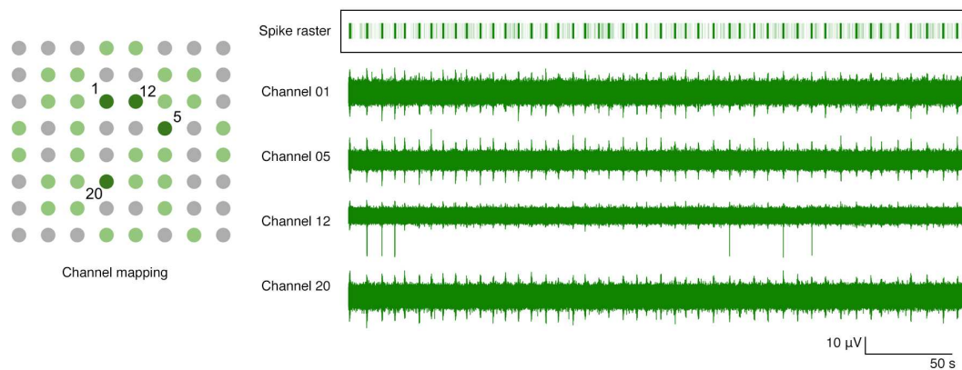
Figure 7. Bursting activity across four channels with channel mapping. Channel mapping shows 64 electrodes in well B2 of the Axion plate. Light green dots are the 32 electrodes recorded by Piphys. Dark green dots mark channels 1, 5, 12 and 20 whose raw recording plots are on the right. The spike raster superimposes all the detected spikes in the shown channels. Each light green vertical line in the raster indicates a spike, and the dark green bar is the result of superimposing multiple spikes in the burst. The bars in the raster plot align with the bursts throughout these four channels.
