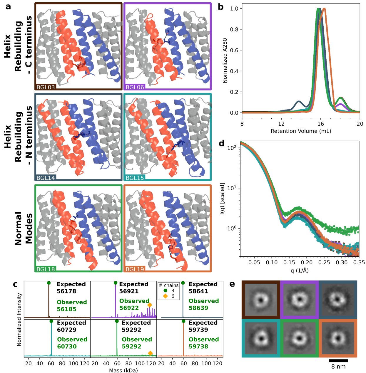
Figure 2: Characterization of BGL homotrimers
