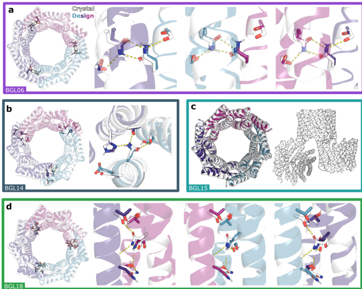
Figure 3. Crystal structures of BGL homotrimers
