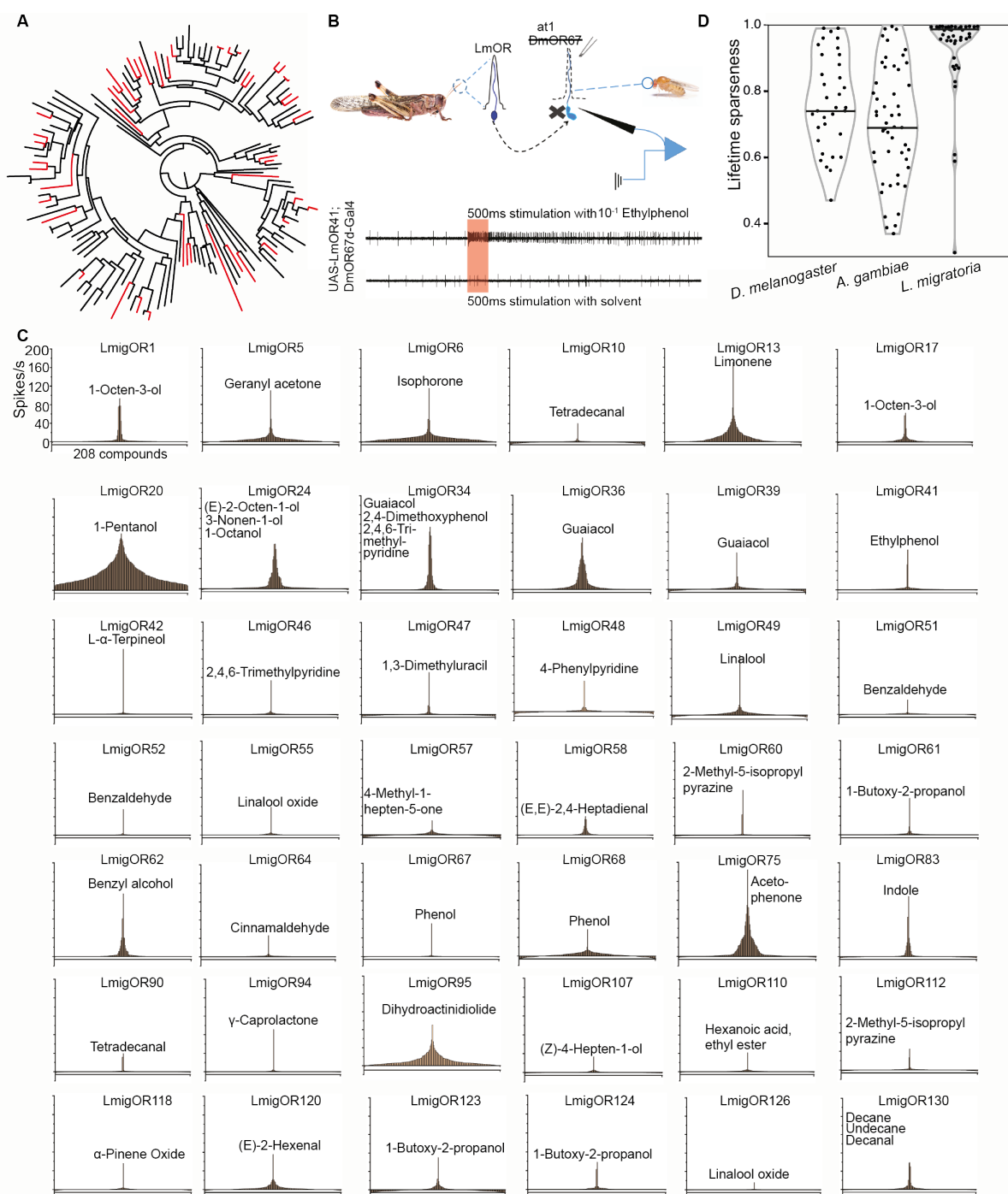
Fig. 2. Response profiles of locust odor receptors. A. Maximum likelihood tree based on amino acid sequences of 139 annotated odorant receptors genes of L. migratoria . B. Schematic of the heterologous expression system using an empty Drosophila at1 neuron with example traces from an at1 neuron mis-expressing LmigOR41 stimulated with ethylphenol (upper trace) or solvent (red bar, stimulus duration). C.
