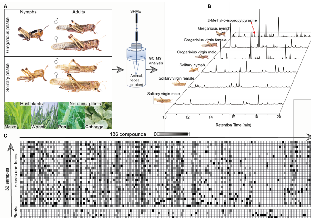
Figure 1. Odorants of potential ecological relevance. A. Example sources of which headspace samples were analyzed (i.e. 32 headspaces of both phases of nymphs, of immature, virgin, and mated females and males, and the corresponding feces of all of them, as well as 2 host- and 2 non-host plants). B. Gas chromatograms revealing 2-methyl-5-isopropylpyrazine as an odorant specific for 4-5 instar nymphs. C. Heat map presentation of 186 volatile compounds identified in the headspace of different sources normalized for each compound (N=4-8 per source; for a heat map presentation of additional, less volatile compounds that were identified in the bodies of nymphs and adults, see Suppl. Figure 1; for the quantification of all compounds see Suppl. Table 1).
