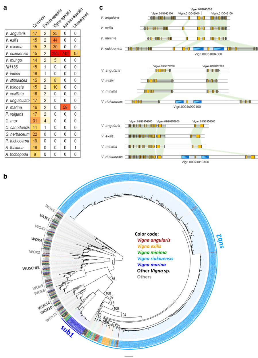
Figure 3. Amplification of WOX-related genes in the genus Vigna . a. Copy number variation in WOX-related orthogroups. b. A phylogenetic tree of WOX transcription factor superfamily. Bootstrap values are presented on Vigna -specific clusters. Clusters of broadly conserved WOX genes are indicated with gene names in black or grey. Subclusters in Vigna -specific clusters are indicated as sub1 and sub2. c. Examples of genomic regions around sWOX gene loci in V. riukuensis and the syntenic regions in other related species. Yellow and gray boxes indicate CDS and UTRs, respectively. Blue boxes with sky blue triangles indicate LTRs. Green shade indicates orthologous genes across species.
