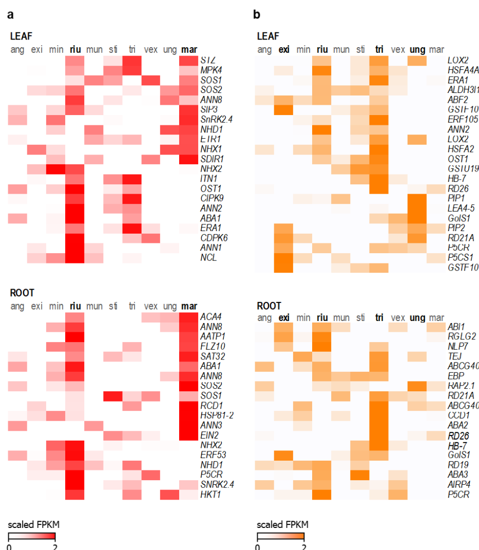
Figure 4. Expression of stress-related genes in Vigna species. a. Genes related to salt tolerance. b. Genes related to drought tolerance. The normalized FPKM values were log2-transformed and then centered with mean among species. Color scales indicate expression levels, where zero is the means. ang, exi, min, riu, mun, sti, tri, vex, ung and mar indicate V. angularis , V. exilis , V. minima , V. riukuensis , V. mungo , V. stipulacea , V. trilobata , V. vexillata , V. unguiculata ssp. dekindtiana and V. marina , respectively.
