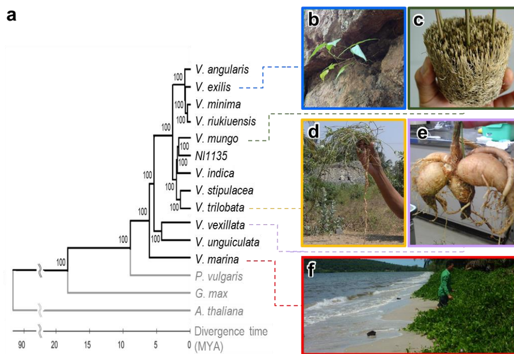
Figure 1. Phylogenetic tree based on the genomic data and photos of representative species. a. NJ tree of Vigna , Phaseolus , Glycine and Arabidopsis . Numbers beside branches represent bootstrap values (%) based on 1000 replications. b. V. exilis growing on a limestone rock. c. Root of V. mungo growing upward under flooded condition. d. Tap root of V. trilobata with few lateral roots. e. Tuber of V. vexillata . f. V. marina in a beach.
