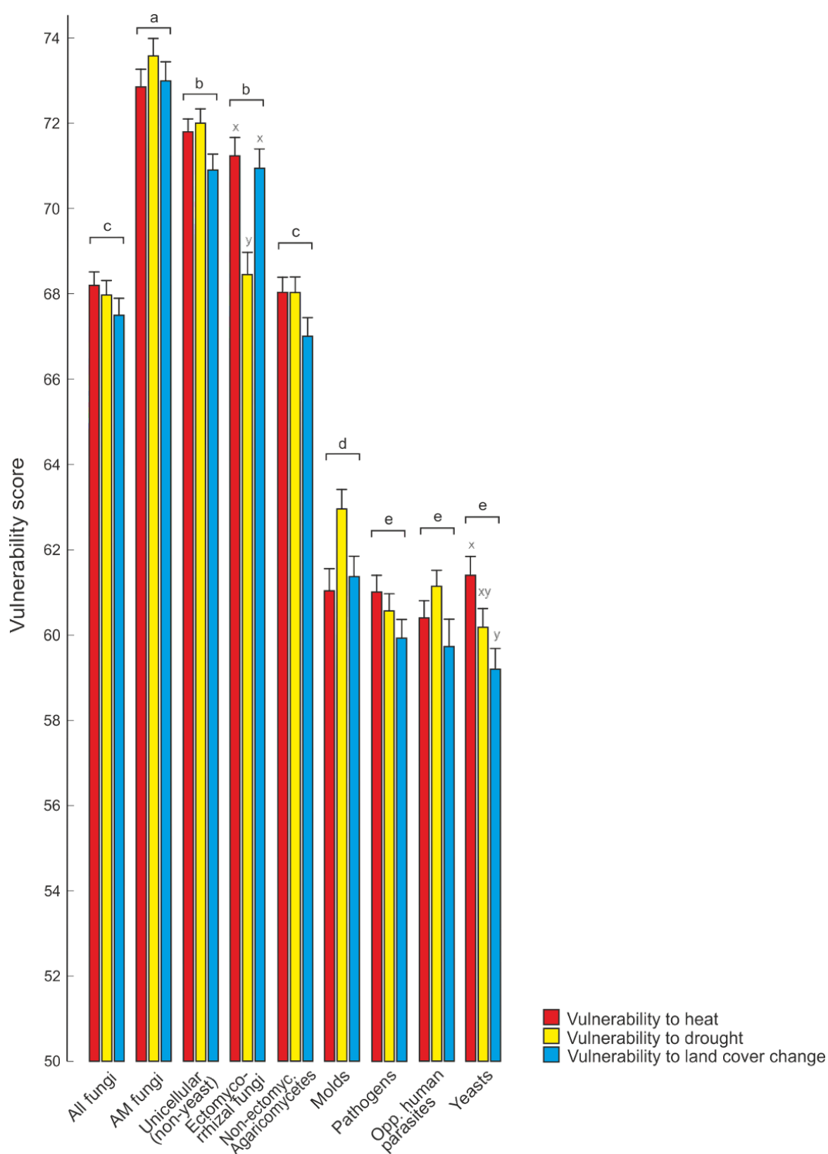
Fig. 9. Vulnerability of fungi and functional groups to global change drivers. Different letters indicate statistically significant ( P < 0.001 ) differences among functional groups (a-e) and among global change drivers within functional groups (x-z).
