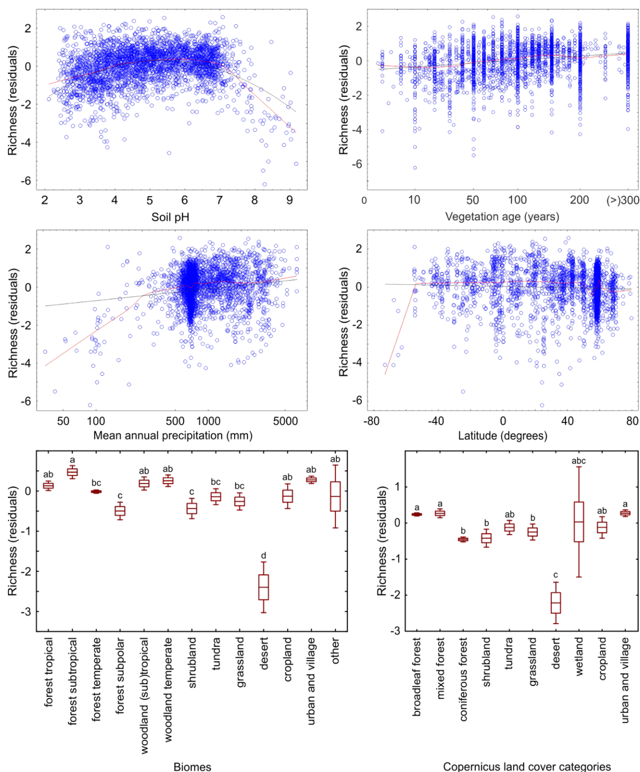
Fig. 4. Response of \alpha -diversity of all fungi to soil pH, vegetation age, mean annual precipitation, latitude, biomes, and land cover categories. For continuous predictors, black lines indicate linear and polynomial fits and red lines indicate lowess fits. For categorical predictors, boxes represent standard error around the mean (central line), whiskers depict 95% CI and letters above boxes indicate statistically significant different groups ( P < 0.001 ).
