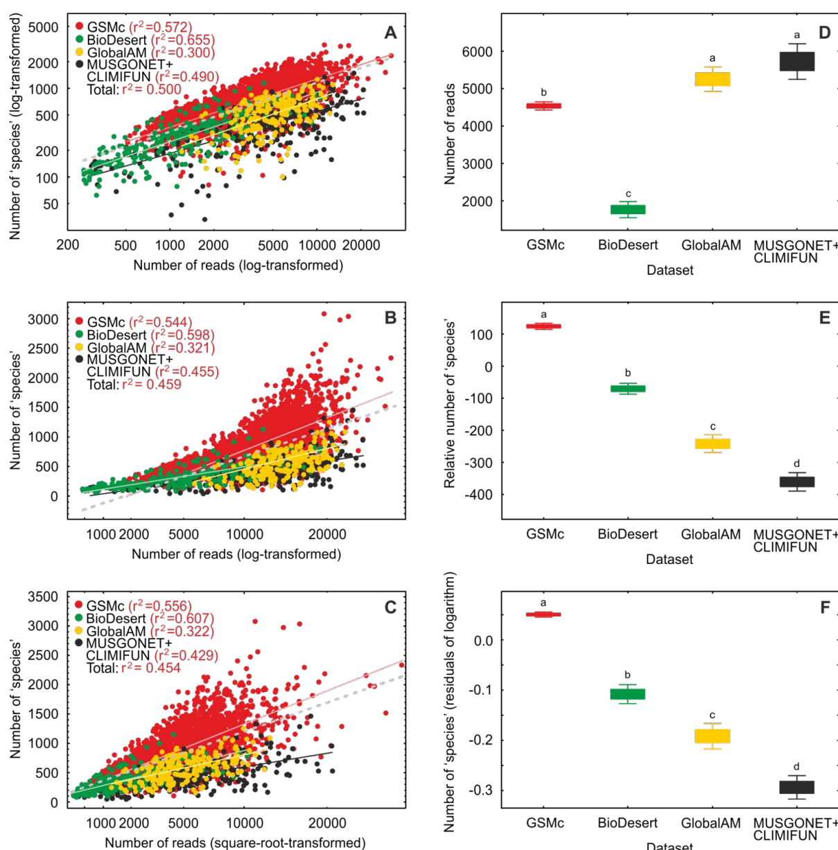
Fig. 3. Relative 'species' accumulation curves (A-C), sequencing depth (D) and 'species' richness (E-F) across four datasets. (A) The log-log relationship between the number of reads and 'species' richness that was used for calculation of residuals and further analyses; (B-C) Relatively lower performance of log-linear relationships of log-transformed and square-root-transformed sequencing depth; (D) Initial differences in sequencing depth among datasets; (E-F) Fungal 'species' richness differences relative to the average in the raw data (E) and residuals of the log-log regression analysis (F). In D-F, boxes indicate standard errors around the mean and whiskers indicate 95% confidence intervals; letters above whiskers indicate statistically significant differences among datasets (using log-transformed data for D-E). These analyses indicate that the log-log transformation for calculating residuals is relatively more robust compared with other methods and that richness estimates from studies with different methods cannot be directly compared.
