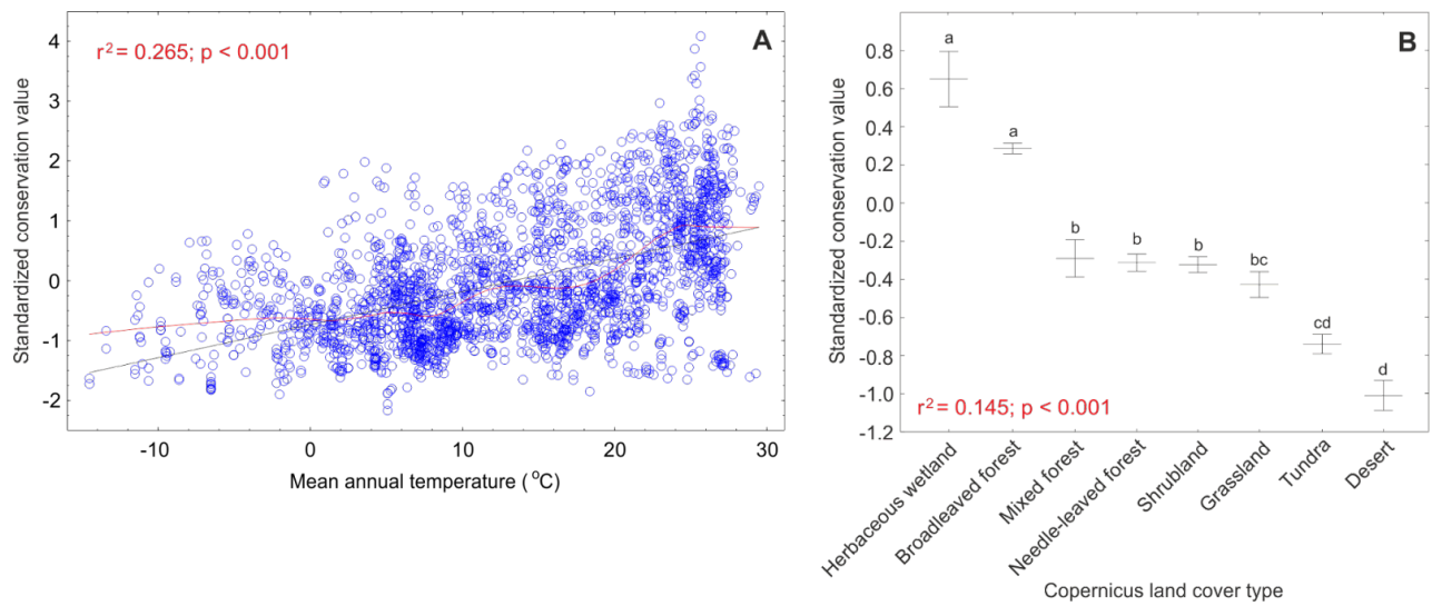
Fig. 10. Relationships between conservation priority areas with mean annual temperature (A) and Copernicus land cover types (B). In A, black and red lines indicate best-fitting linear and lowess functions, respectively. In B, central lines and whiskers indicate mean and standard errors, respectively; letters above whiskers indicate statistically significant differences among land cover types.
