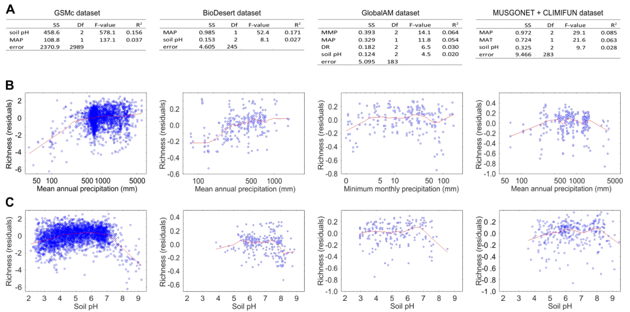
Fig. 5. Comparison of \alpha -diversity patterns in all fungi across four most inclusive datasets: (A) best models (only bioclimatic variables and soil pH were included in model selection), (B) lowess regression curves for the best-fitting climatic predictor, and (C) lowess regression curves for soil pH.
