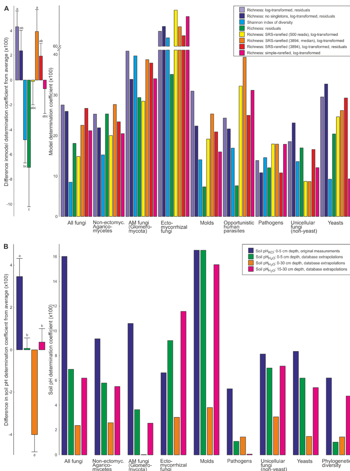
Fig. 2. Comparison of (A) richness proxies (use of log-transformation, residuals of sequencing depth, SRS or simple rarefaction) and (B) measures of soil pH on analytical performance. Relative goodness was estimated based on the determination coefficients of the best models (A) or pH-only models (B). In left panels, significant among-group differences are indicated with different letters based on Tukey Posthoc tests; bars, means; whiskers, SE. Soil pH KCl were determined experimentally, whereas pH H 2 O were obtained from Poggio et al. (2021).
