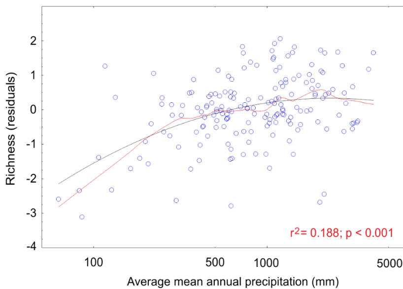
Fig. 6. The effect of average mean annual precipitation on \gamma -diversity of fungi at the ecoregion scale. Black line, best quadratic fit; red line, lowess curve.
