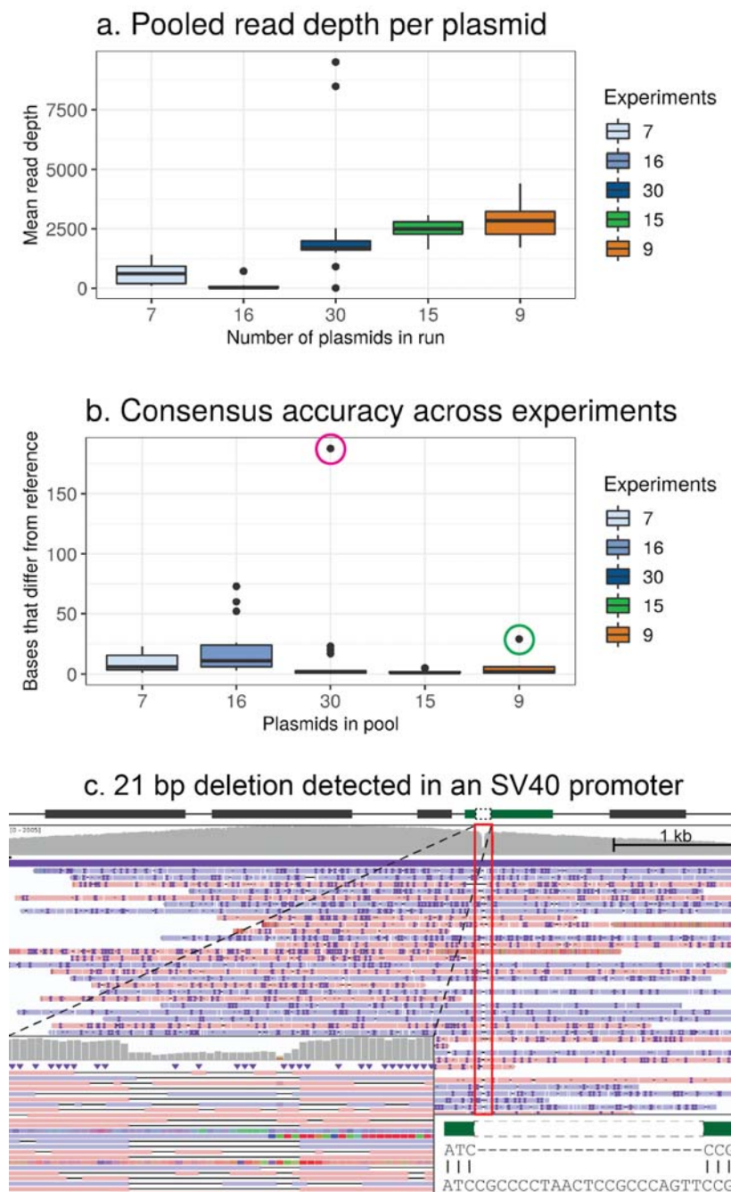
Figure 3. Characteristics of plasmid sequencing experiments and an example of variant detection
