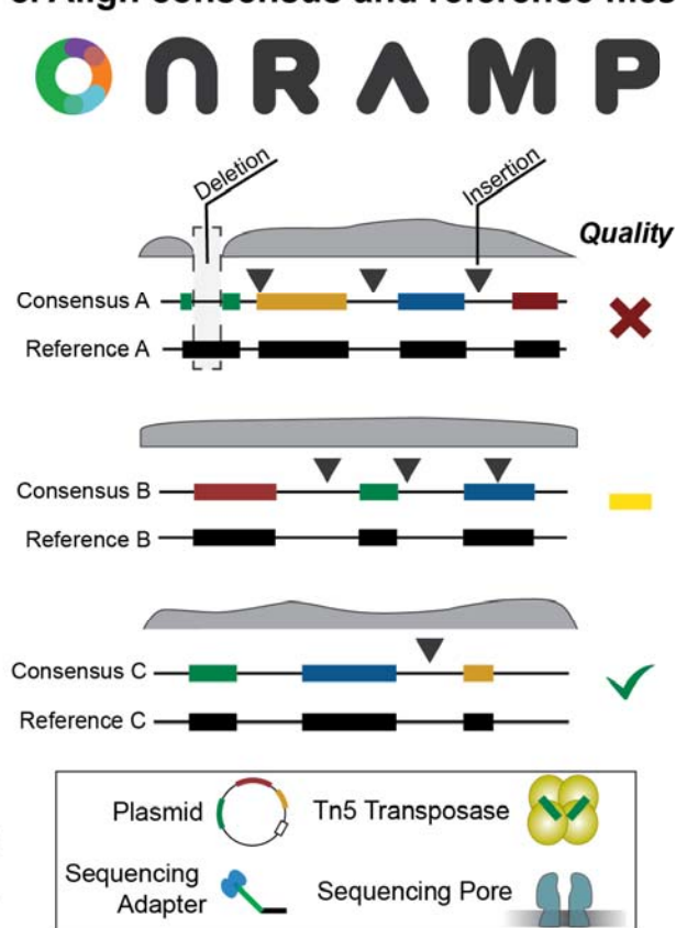
Figure 1. Plasmid library preparation and consensus sequence generation using On-Ramp.
