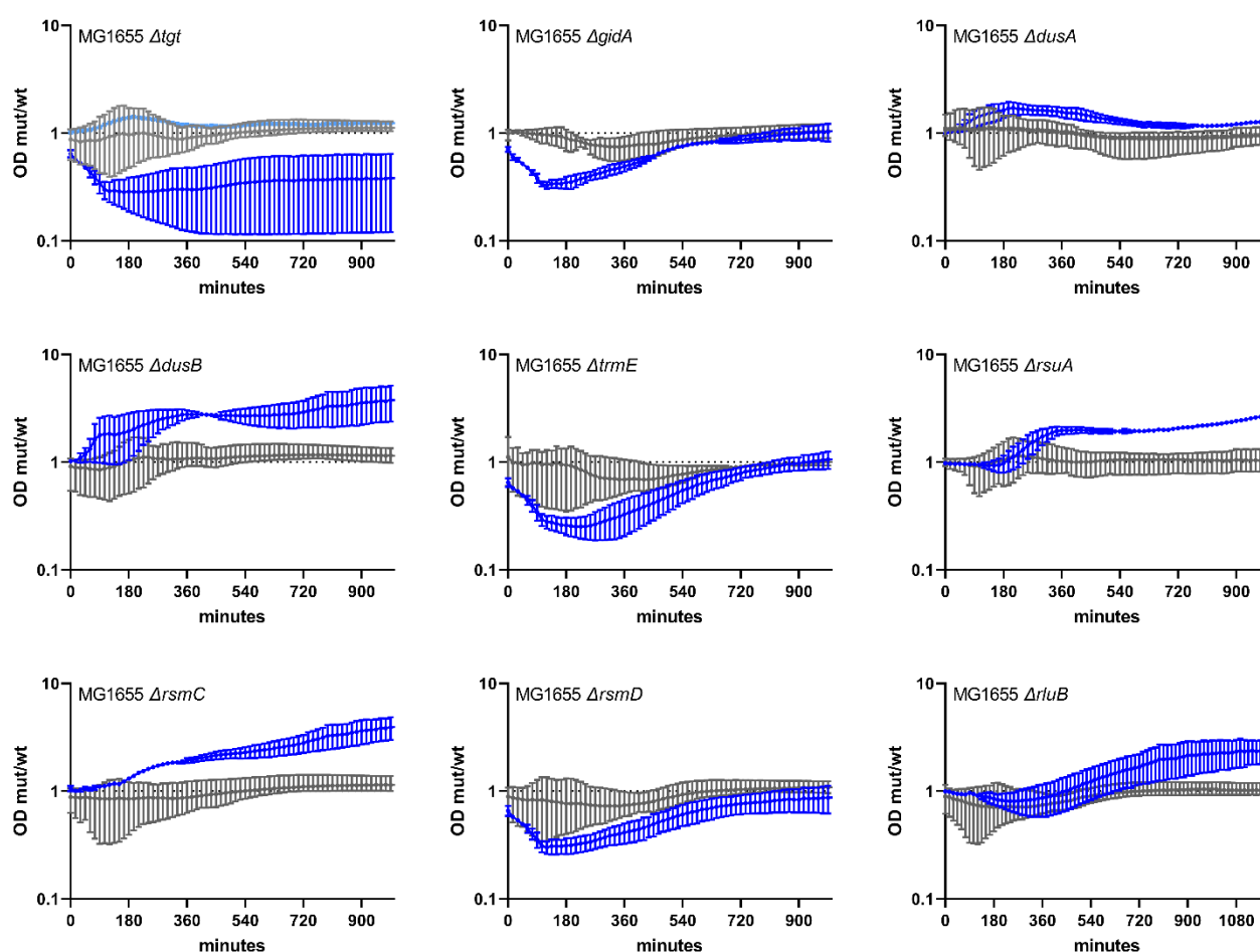
Figure 4. Growth of E. coli MG1655 WT and derivatives deleted for selected RNA modification genes in sub-MIC TOB. Overnight cultures were diluted 100x in fresh MH medium, on 96 well plates. Each well contained 200 µl. Plates were incubated with shaking in TECAN plate reader device at 37°C, OD 620 nm was measured every 15 minutes. Grey: no treatment. Blue: sub-MIC TOB, at 0.2 µg/ml (50% of the MIC for MG1655 in MH liquid culture). The Y-axis represents the OD of the mutant divided by the OD of the WT strain in the same growth conditions, and thus reflects slower (below 1) or faster (above 1) growth. Standard deviation is shown.
