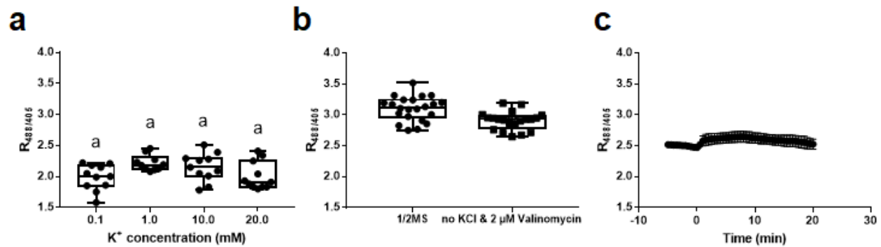
Supplementary Figure 10. GINKO2 responses in plants under various conditions. a Effect of increasing concentrations of KCl on g10-90::GINKO2 R 488/405 without K + depletion pre-treatment. n ≥ 10 individual seedlings. Letters indicate the significantly different statistical groups with P < 0.05 minimum. Statistical analysis was conducted with nonparametric multiple comparisons. b Effect of a six-hour K + depletion treatment with 0 mM KCl and 2 μM valinomycin on g10-90::GINKO2 R 488/405 . 1/2MS: Murashige and Skoog medium half strength. n ≥ 20 individual seedlings. P < 0.01. c Effect of 100 mM NaCl on g10-90::GINKO2 R 488/405 in root tip without prior K + depletion. Treatment was applied at time zero. n = 9 individual seedlings.
