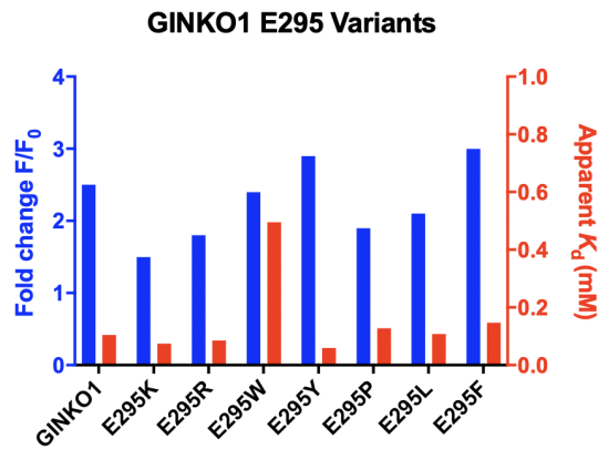
Supplementary Figure 3. Comparison of E295 variants of GINKO1. The bulky hydrophobic residues Y and F lead to improved F_{\max}/F_0 . E295W retained the F_{\max}/F_0 , but simultaneously increased the apparent K_d substantially. E295K and E295R resulted in a smaller F_{\max}/F_0 than template GINKO1.
