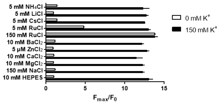
Supplementary Figure 6. Ion competition assay of GINKO2. To examine whether other cations in the environment could affect the K + response of GINKO2, a specificity test was performed in both 0 and 150 mM K + buffer (n=3). Without K + , only Rb + was able to induce a fluorescence change. In presence of 150 mM K + , the fluorescence change induced by K + was not affected by any other cations.
