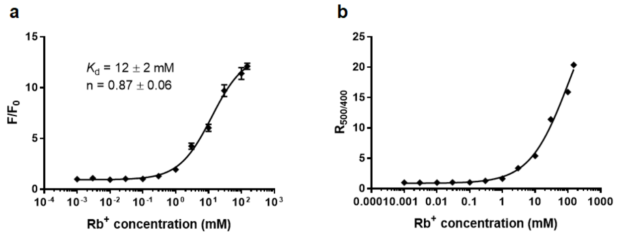
Supplementary Figure 7. Rb + titration of GINKO2. a The fluorescence change (F/F 0 ) of GINKO2 versus Rb + concentration. n=3. b R 500/400 versus Rb + concentration. GINKO2 responds to Rb + ratiometrically.
