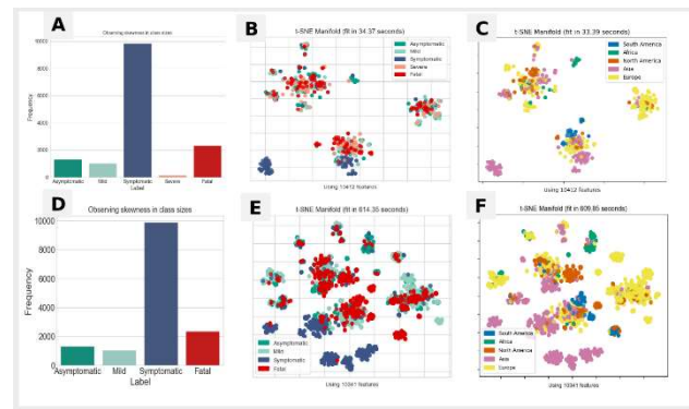
Figure 2. tSNE plot to explore spatial grouping of genomes based on associated infection outcome. Panel (A): a bar plot indicating the class size of various 'patient status' specific genome sequences selected for the unfiltered machine learning task. Panel (B): the tSNE plot generated using stratified sampling for all chosen outcome labels (randomly picked 168 genomes, i.e. minority class size, from each of category of genome sequences). Panel (C): the plots for genomes presented in panel B, but overlaid with geographical information about location of data submission. Panel (D): the class size of samples after excluding the minority class/outcome (Severe). Panel (E) represents the tSNE plot using stratified sampling for labels other than severity group (smallest class of 168 genomes) with geographical information overlaid in Panel (F).
