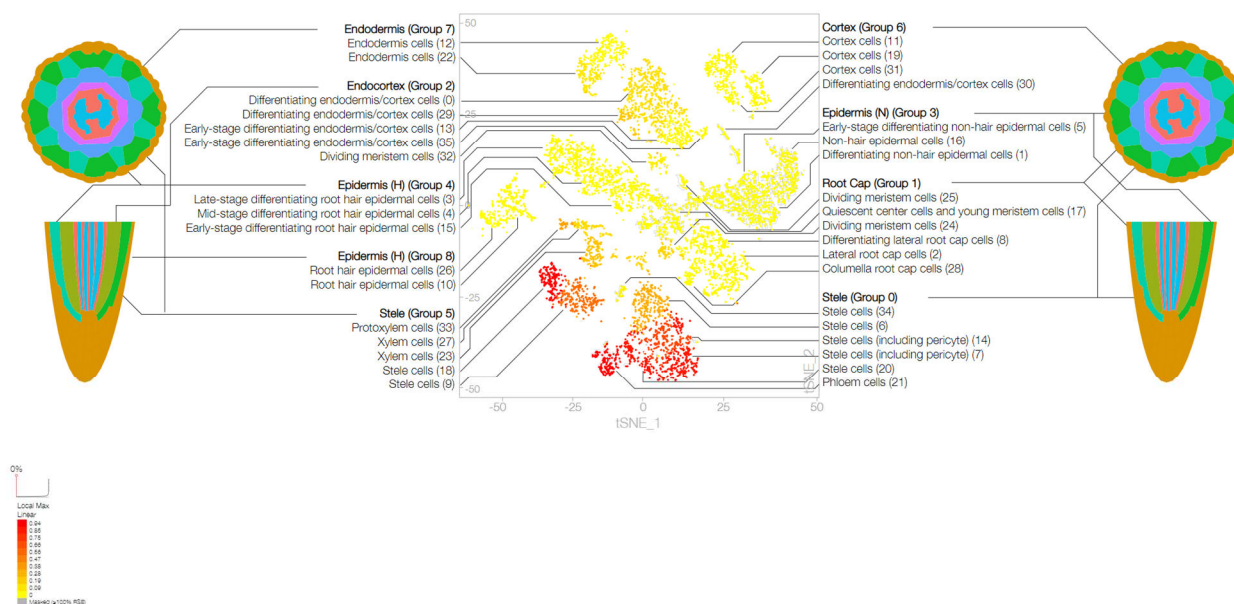
Figure 8: Single Cell RNA-seq eFP View for the gene At5g60200
