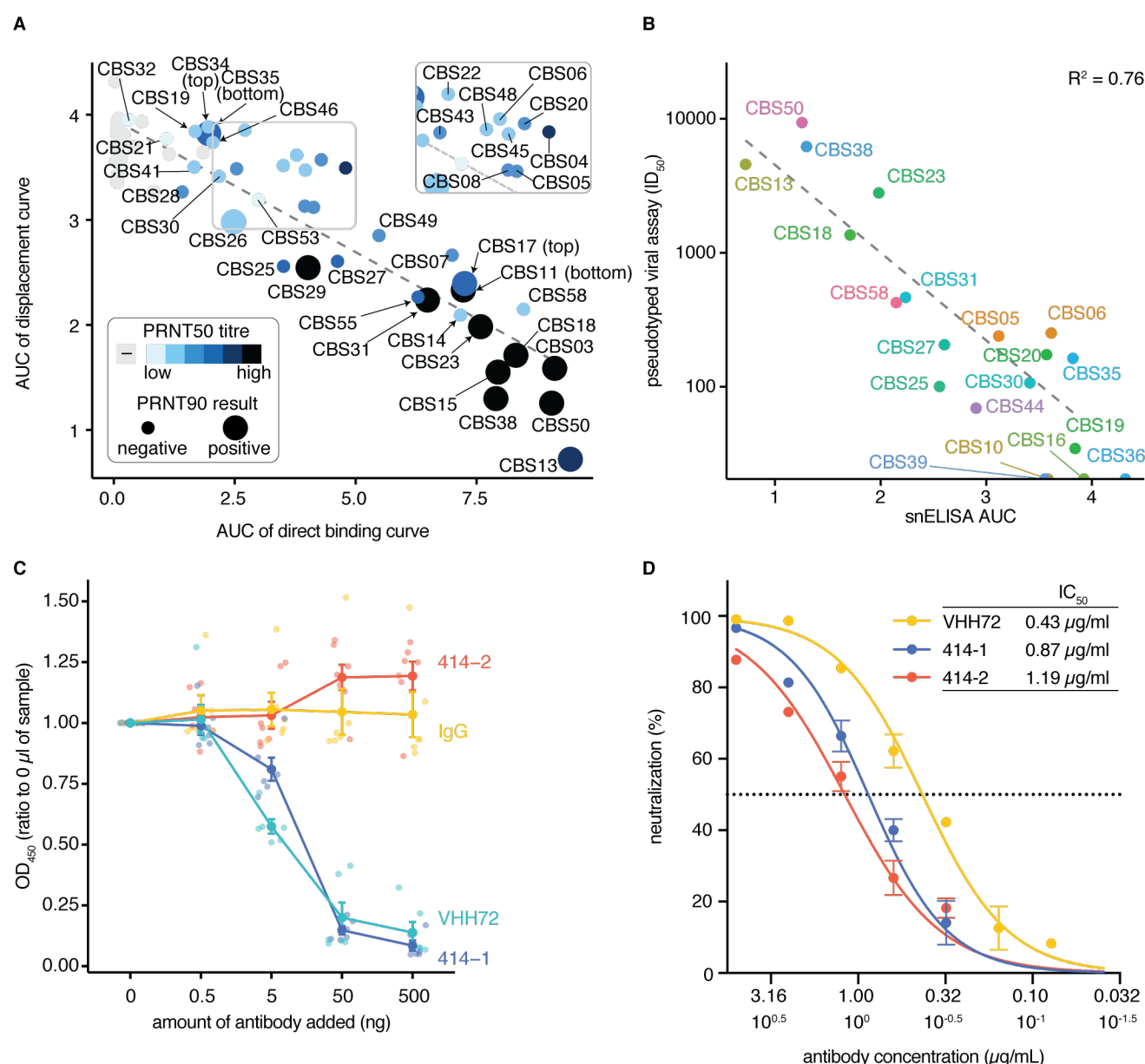
Figure 3. Validation of the snELISA results using orthogonal methods. (A) Results of the plaque reduction neutralization tests on the same samples overlaid on the AUC curves from Figure 2C (n=57 samples). Color coding indicates the PRNT50 titers while negative/positive hits on the PRNT90 assay are displayed with a different sized dot (see Supplemental Figure 11 for additional PRNT results and Supplemental Figure 12 for spike pseudotyped virus results). (B) Correlation between the lentiviral spike pseudotyped virus assay calculated IC_{50} values and the AUC results from the snELISA. Assessment of the ability of monoclonal or affinity reagents to block the interaction between ACE2 and the RBD in (C) the snELISA or (D) the lentiviral spike pseudotyped assay (see Supplemental Figure 13-16 for the direct binding and viral neutralization assays and additional reagents tested). Values for panel C were generated from three independent experiments, and underlaid points have been jittered along the x-axis. Values for panel D were obtained in one experiment in technical triplicate. Error bars represent the mean \pm standard error of the mean (SEM).
