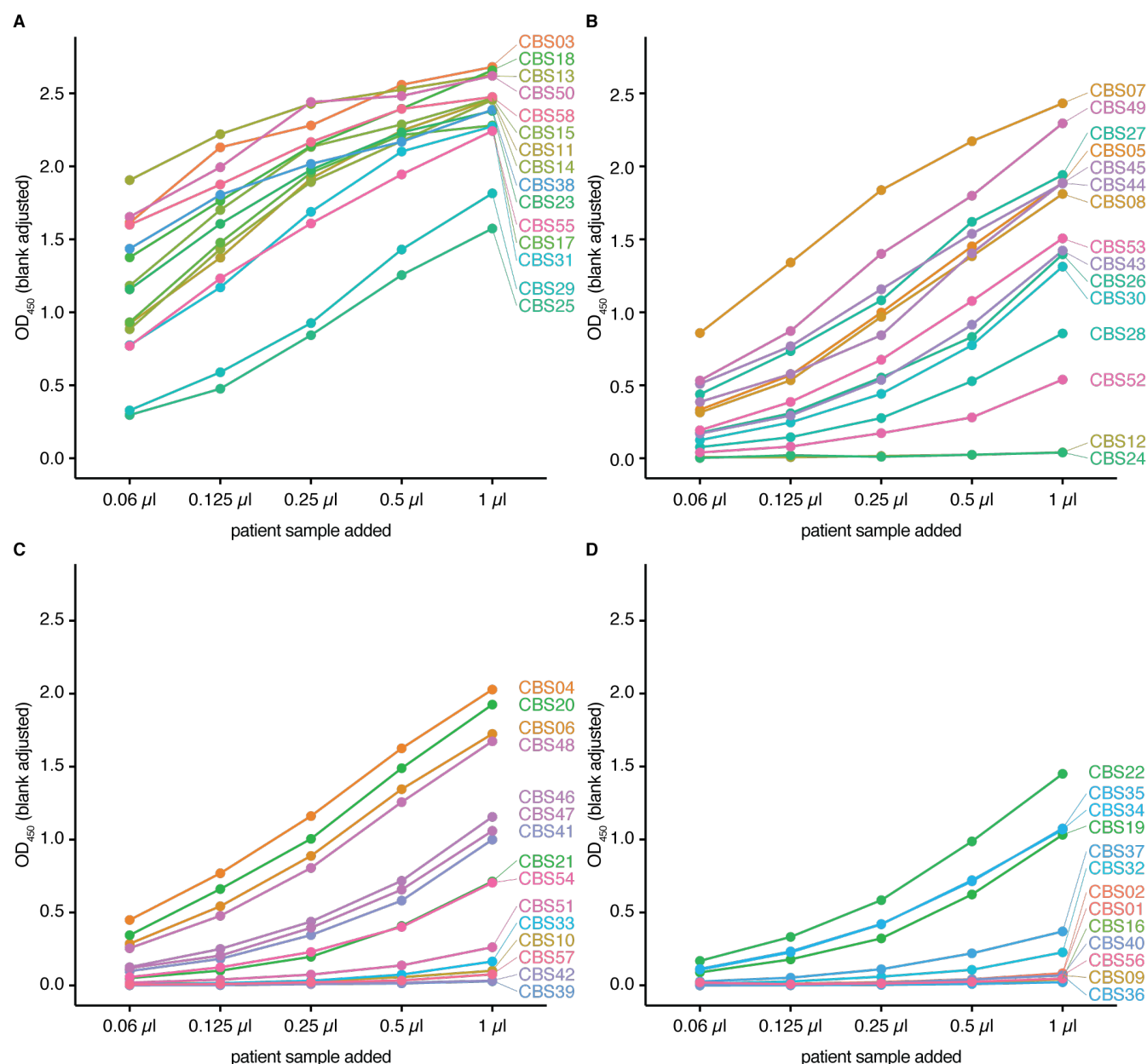
Supplemental Figure 6. The entire set of direct binding ELISAs with titrations on different samples of the Canadian Blood Services cohort. Samples were ranked based on the AUC of the snELISA curve and were plotted in four batches starting with samples most effective at blocking the RBD-ACE2 interaction (A), to the lowest (D). Related to Figure 2B and Supplemental Figure 8 . The five-point curves were generated from one experiment (n = 58).
