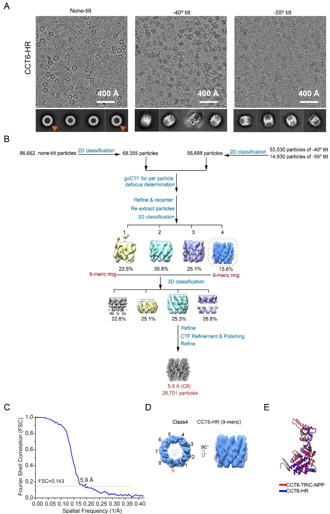
Fig. S6 Cryo-EM data processing of CCT6-HR. (A) Representative cryo-EM
