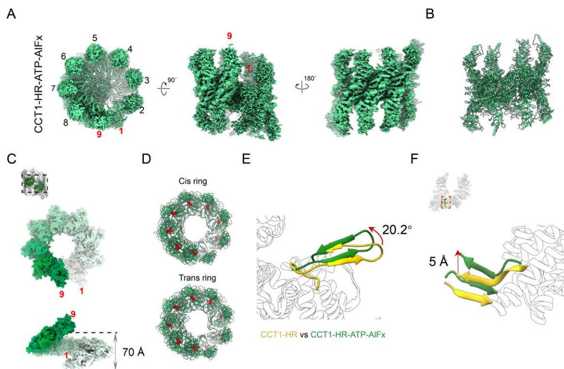
Fig. 2 Cryo-EM structure of CCT1-HR-ATP-AIFx remaining in an open conformation. (A) The cryo-EM map of CCT1-HR-ATP-AIFx, from left to right: top view (with the subunit pair numbered from the lowest 1 to the highest 9), and side views from the seam/the back of the seam regions. (B) The pseudoatomic model of CCT1-HR-ATP-AIFx. (C) The spiral conformation of the E domain of CCT1-HR-ATP-AIFx, with the rise between the lowest subunit pair 1 to the highest 9 being labeled. (D) Nucleotide occupancy status of CCT1-HR-ATP-AIFx. (E and F) Model alignment for the neighboring subunits between CCT1-HR (gold) and CCT1-HR-ATP-AIFx (forest green), aligned by the left subunit. Showing is that ATP-hydrolysis could lead to an obvious upward lift of \sim 20.2^\circ in the stem loop of the left subunit (E), coupled with a simultaneous lift of \sim 5 \text{ \AA} of the N/C termini of the right neighboring subunit (F).
