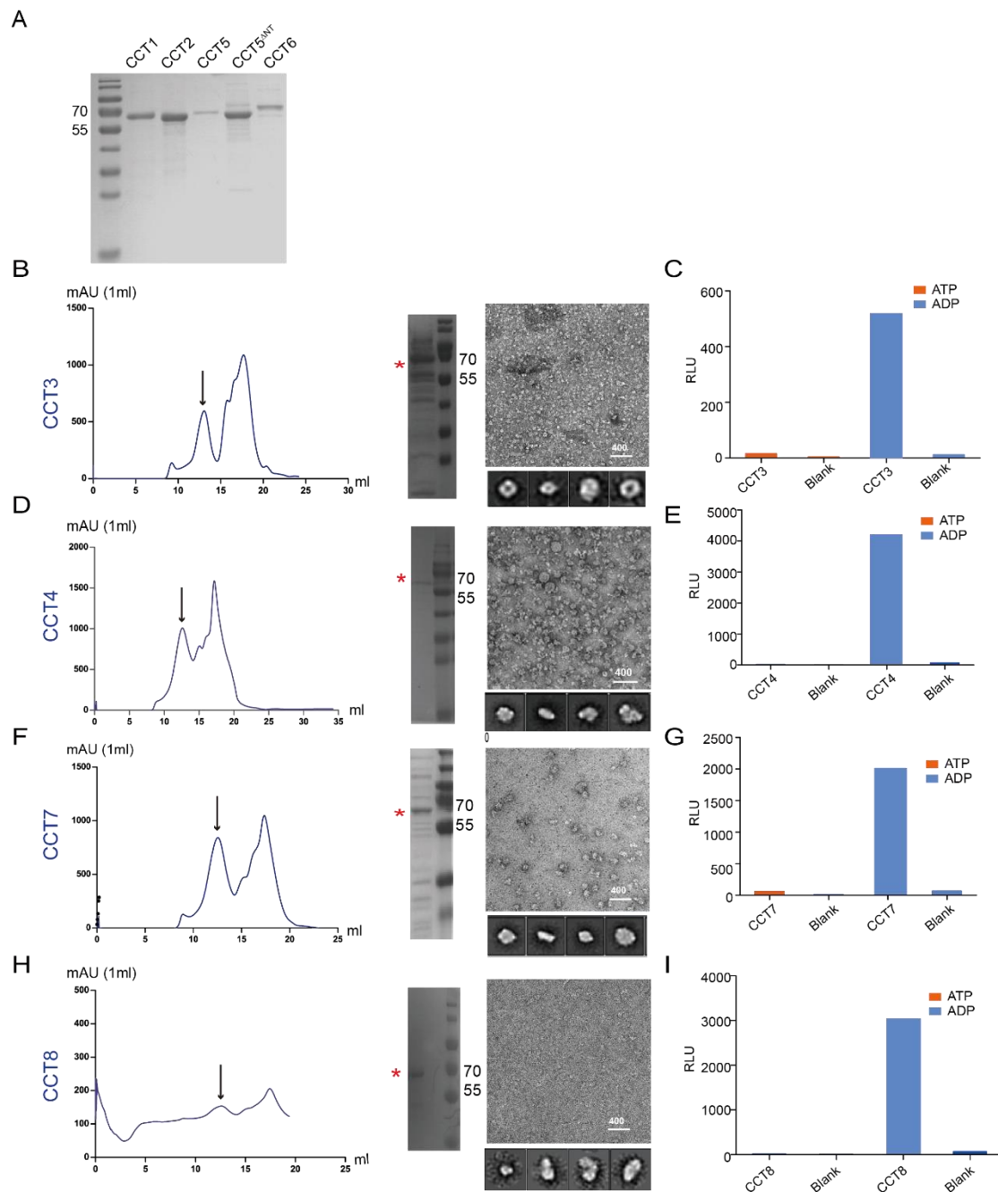
Fig. S1 Purification and characterization of the \gamma TRiC subunits expressed in E. coli . (A) SDS-PAGE of the subunits that could form ring-shaped structure (including CCT1, CCT2, CCT5-ATP, CCT5 \Delta NT-ATP, and CCT6), stained with Coomassie Brilliant Blue. (B, D, F, H) Gel-filtration graph, SDS-PAGE result, representative NS-EM micrograph, and reference-free 2D class averages for CCT3 (B), CCT4 (D), CCT7 (F),
