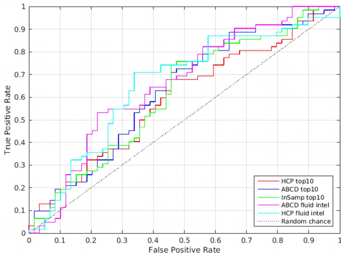
Figure 2 Whole Brain Receiver Operator Characteristic Curve plotting the false positive rate versus true positive rate for the top k=10 HCP, ABCD, and In-sample models and the fluid intelligence HCP and ABCD models. All of these models were tested using 10-fold cross validation logistic regression models. The diagonal dotted line shows chance accuracy. For most all subjects, the big data models (blue, red, cyan, magenta lines) are above the in-sample model (green line) meaning that big data models help improve the classification for most subjects in the clinical dataset.
