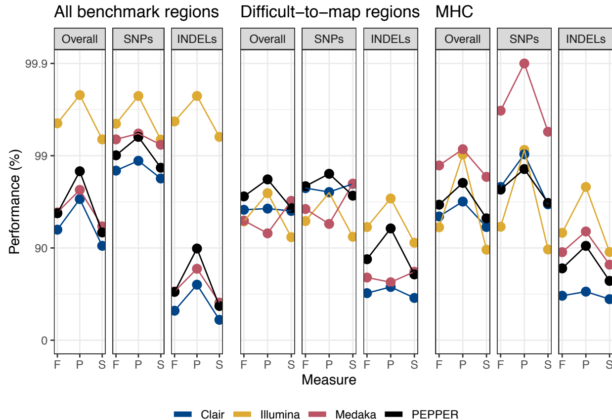
Figure 1. Performance metrics measured against the Genome in a Bottle v4.2 truth set. All benchmark regions: Complete truth set. MHC: Intersect of major histocompatibility complex and truth set. Difficult-to-map regions: Intersect of the truth set with segmental duplications and regions where 100 bp read pairs have \leq 2 mismatches and \leq 1 indel difference from another part of the genome. MHC: Major histocompatibility complex; F: F-measure; P: Precision; S: Sensitivity
