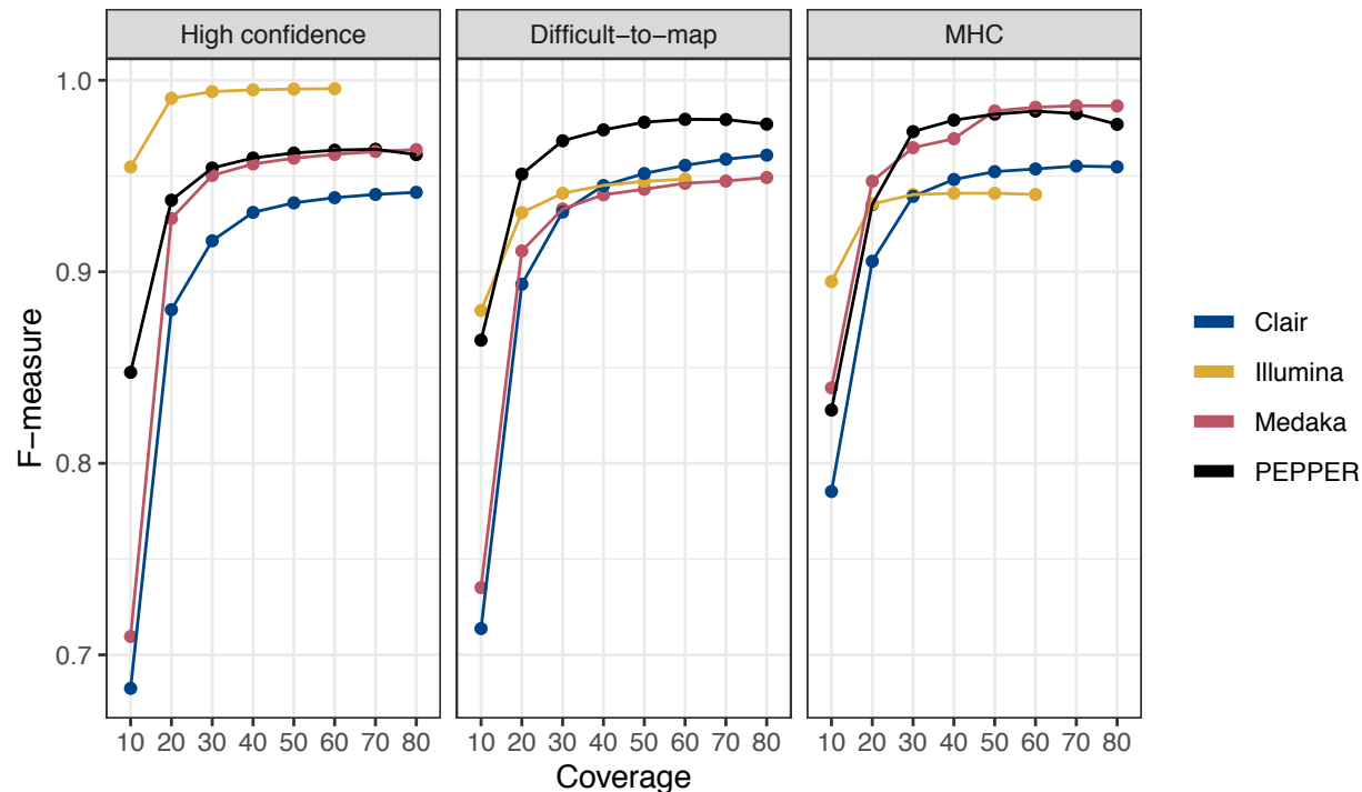
Figure 2. Variant calling performance as a function of sequence coverage. F-measure was determined between 10 and 80X coverage in 10X increments for each evaluation region. Numbers are average of HG003 and HG004. MHC: Major histocompatibility complex.
