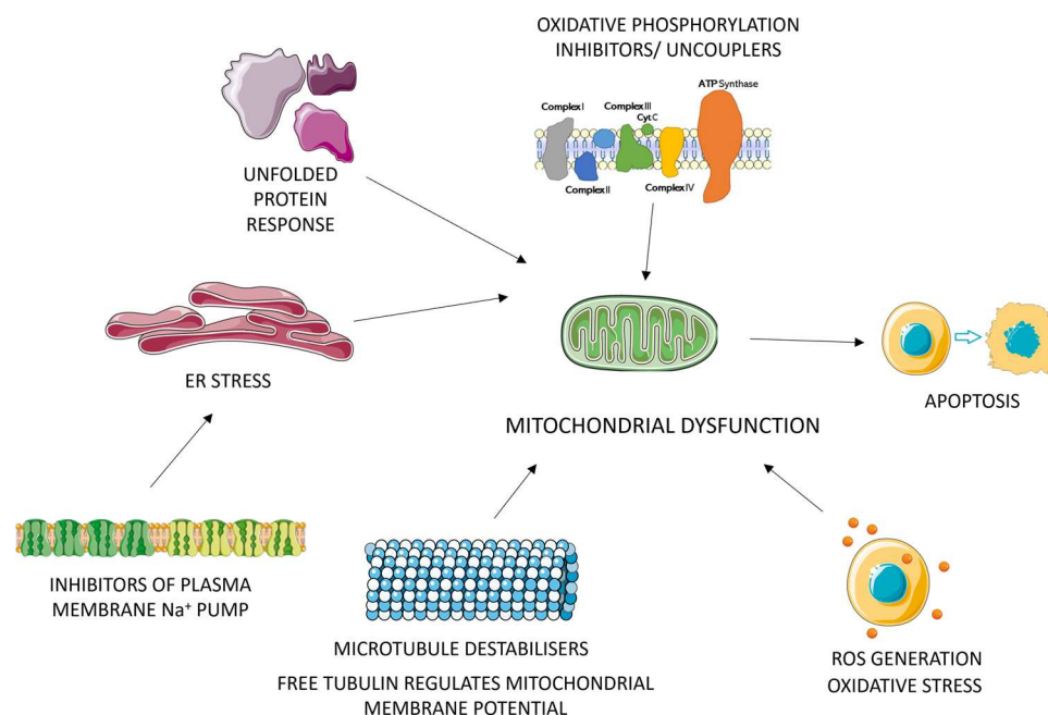
Fig. 1 Some of the major mechanisms of action of mitochondrial toxicants. Toxicants act on multiple pathways to exhibit mitochondrial toxicity, including but not limited to, unfolded protein response, inhibition of mitochondrial respiratory chain or uncoupling of oxidative phosphorylation, oxidative stress from responses including generation of reactive oxygen species (ROS), microtubule disruption and ER stress from various responses including inhibition of Na + pumps etc. The Figure was partly generated using Servier Medical Art, provided by Servier, licensed under a Creative Commons Attribution 3.0 unported license.
