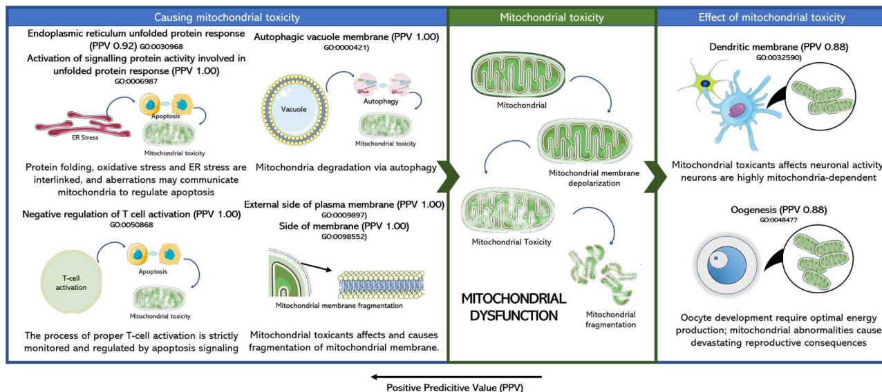
Fig. 7 Biological implication of gene expression features in relation to mitochondrial toxicity. Biological implication of mitochondrial toxicity translated from the Gene Expression features. Features causing mitochondrial toxicity mainly related to unfolded protein response (possibly related to ER stress) and plasma membrane (related to membrane depolarisation). Some effects of mitochondrial toxicity were also captured by Gene Expression features such as oogenesis and dendritic plasma membrane; both processes are heavily mitochondria dependent. Further details in Supplementary Data 5. The Figure was partly generated using Servier Medical Art, provided by Servier, licensed under a Creative Commons Attribution 3.0 unported license.
