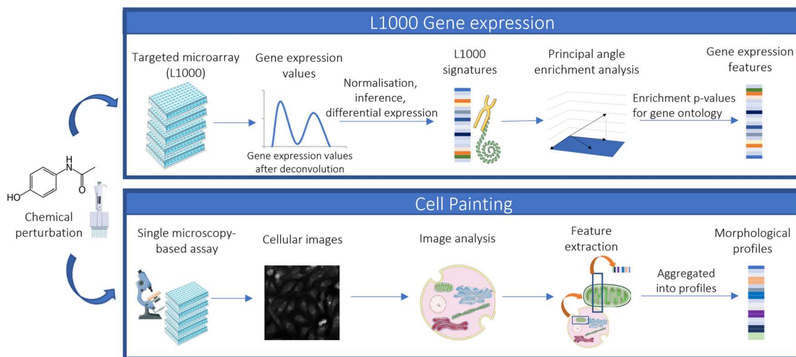
Fig. 2 Overview of the workflow employed in this study. L1000 technology for Gene Expression and Cell Painting Technology for cell morphology statistics. The LINCS L1000 gene expression technology profiles changes in 978 landmark genes before and after chemical perturbations on different human cell lines. Raw unprocessed flow cytometry data from Luminex is converted to quantile-normalized gene expression profiles for all replicates of each compound. We use Gene Expression data from Wang et al. 45 , who for each compound, computed the strongest gene expression signature using the Characteristic Direction (CD) method and computed enrichment p values for each CD signature in the space of all genes against gene set libraries using Principal Angle Enrichment Analysis (PAEA). The Cell Painting assay, on the other hand, captures cellular morphological changes in the form of numerical statistics which are converted from microscopic image data of cells treated with chemical perturbations. The Figure was partly generated using Servier Medical Art, provided by Servier, licensed under a Creative Commons Attribution 3.0 unported license.
