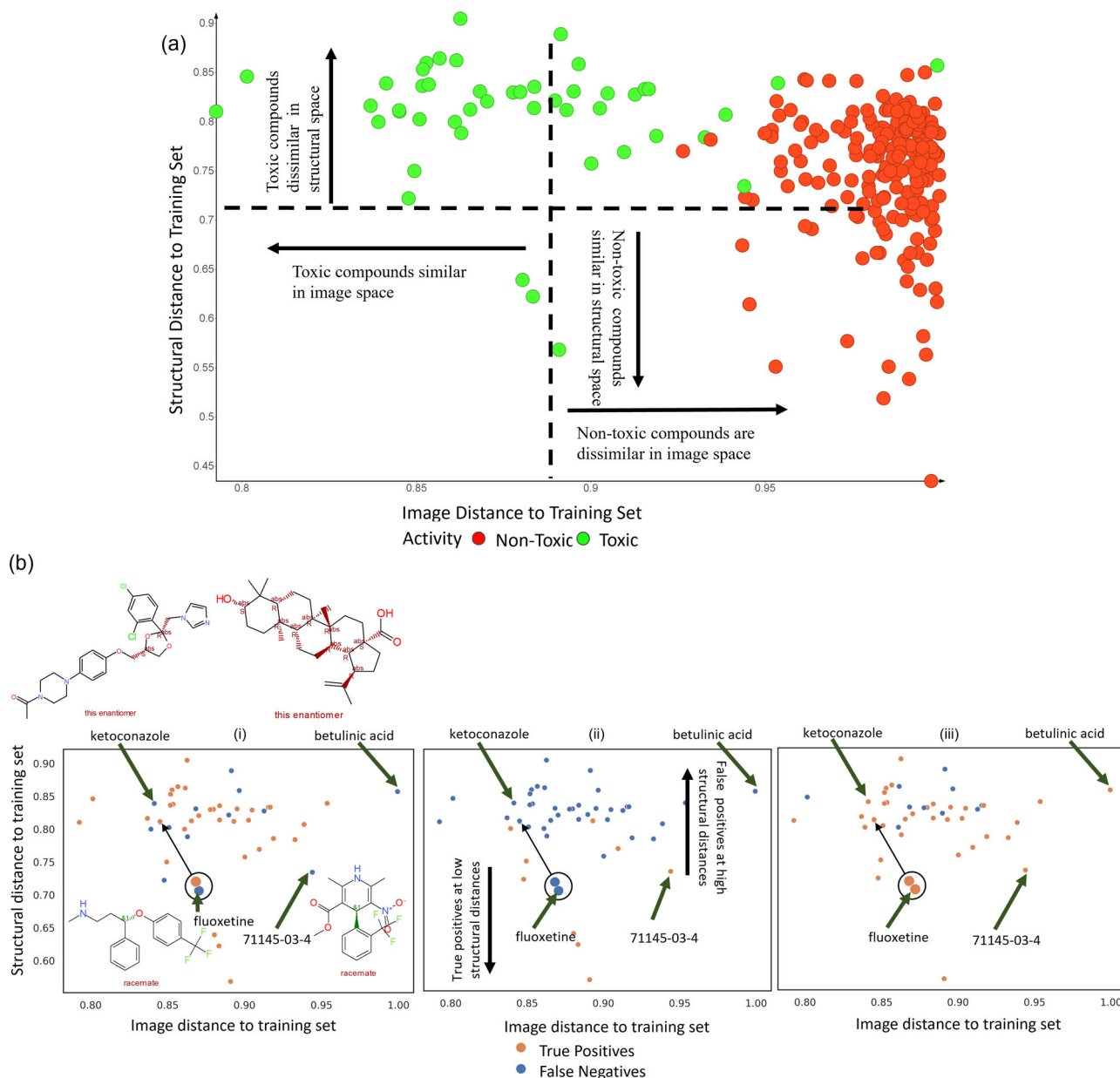
Fig. 9 Predictions of mitochondrial toxicants in the external test set in relation to structural and morphological distance to training set. a Most mitotoxic compounds are similar in image space for training ( n = 382 compounds) and external test set ( n = 244 compounds), however, non-toxic compounds in the external test set were dissimilar to non-toxic compounds in training set in the image space. Further, toxic compounds are often dissimilar in structural space, indicating the need for fusion models. b Structural and morphological distance for mitotoxic compounds in external test set ( n = 244 compounds) to the training set ( n = 382 compounds) for models using (i) Cell Painting features, (ii) Morgan fingerprints and the (iii) Late-stage fusion models. Morgan fingerprints failed to correctly classify mitotoxic compounds (eg. betulinic acid) at high structural distances while models using Cell Painting features could extrapolate well into structurally diverse compounds. The late-stage fusion models correctly classified mitotoxic compounds (eg. 71145-03-4 or methyl 2,6-dimethyl-5-nitro-4-[2-(trifluoromethyl)phenyl]-1,4-dihydropyridine-3-carboxylate, ketoconazole and fluoxetine) in both diverse morphological and structural space where individual models failed demonstrating the synergistic effect of the features spaces.
