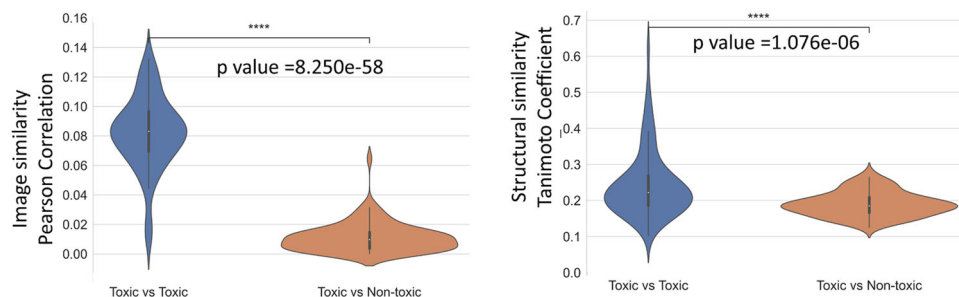
Fig. 3 Mitotoxic compounds are considerably different from non-toxic compounds in morphological space. Intra- and inter-class pairwise similarity for 486 compounds (85 mitotoxic) Median of five highest Tanimoto similarity coefficients of Morgan fingerprints and (B) Absolute value of the median of fifteen most positively and fifteen most negatively Pearson correlation effect sizes of selected 110 Cell Painting features for mitochondrial toxic and non-toxic compounds. Mitotoxic compounds considerably vary from non-toxic compounds in morphological space (median Pearson correlation of 0.140 vs 0.038, t test independent p value = 3.301e-20) while also varying in structural space (median Tanimoto Similarity of Morgan fingerprints 0.208 vs 0.183, t test independent samples p value = 6.329e-03).
