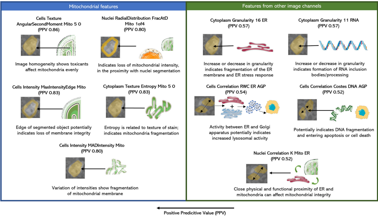
Fig. 6 Biological implication of Cell Painting features in relation to mitochondrial toxicity. Biological implication of mitochondrial toxicity translated from the computational image statistics of Cell Painting features. Features were mainly related to edge intensity of cells (possibly related to integrity of cell wall), radial distribution and intensity in mitochondria (related to mitochondrial death) and granularity features (related to cell death and amount of information contained in cellular images). Further details in Supplementary Data 4. AGP Actin Golgi Plasma membrane, DNA Deoxyribonucleic acid, ER endoplasmic reticulum, Mito Mitochondria, RNA Ribonucleic acid. The Figure was partly generated using Servier Medical Art, provided by Servier, licensed under a Creative Commons Attribution 3.0 unported license.
