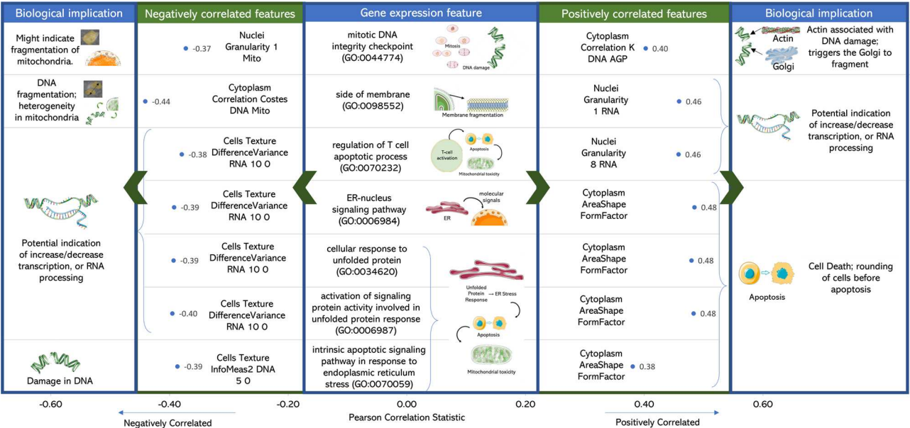
Fig. 5 Biological implication in mitochondrial toxicity of the cell painting features correlated to gene expression. Computational significance and biological implication in mitochondrial toxicity of the Cell Painting features that are most positively or negatively correlated to Gene Expression descriptors particularly unfolded protein response and endoplasmic reticulum stress (RNA variance and cell area shape), T cell apoptotic processes (mitochondrial granularity and DNA fragmentation) and side of the membrane (RNA granularity and heterogeneity in mitochondria). Further details in Supplementary Data 3. The Figure was partly generated using Servier Medical Art, provided by Servier, licensed under a Creative Commons Attribution 3.0 unported license.
