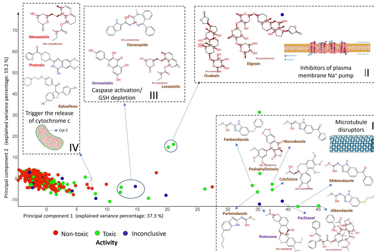
Fig. 4 Compound having similar mechanisms of action cluster in morphological space. Principal Component Analysis of 542 compounds in 110-dimensional Cell Painting feature space. Certain compounds clustered further away from the distribution of majority of compounds having similar mechanisms of actions such as of microtubule destabilisers, or compounds inducing apoptotic signalling cascades, compounds causing oxidative stress due to GSH depletion or those that are inhibitors of plasma membrane \text{Na}^+ pump (all of which reduce mitochondrial membrane potential). Cluster I (microtubule destabilisers): rotenone, albendazole, parbendazole, mebendazole, nocodazole, fenbendazole, colchicine, paclitaxel and podophyllotoxin; Cluster II (inhibitors of plasma membrane \text{Na}^+ pump): ouabain and digoxin; Cluster III (caspase activation and GSH depletion): devazepide, simvastatin, simvastatin; and Cluster IV (trigger the release of cytochrome c into the cytosol): mevastatin, prazosin, and raloxifene. The Figure was partly generated using Servier Medical Art, provided by Servier, licensed under a Creative Commons Attribution 3.0 unported license.
