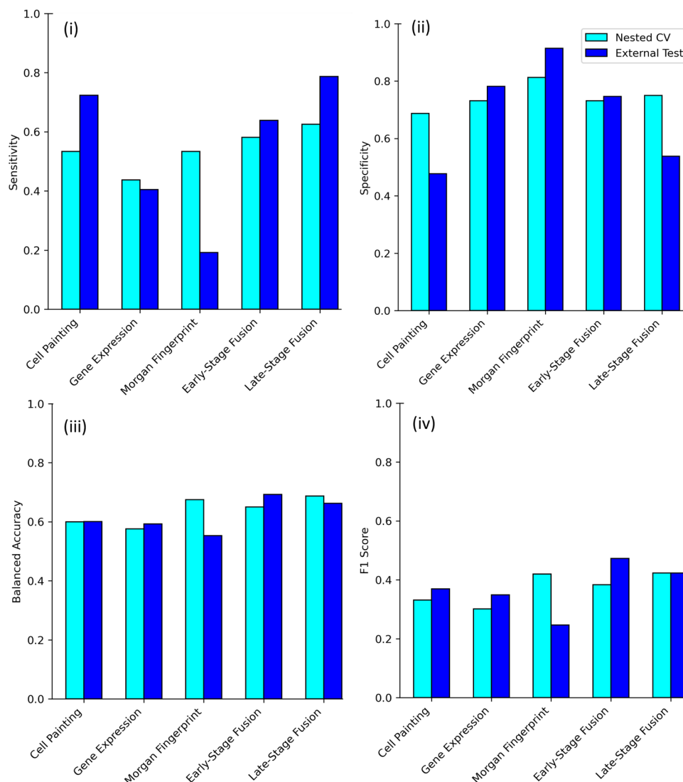
Fig. 8 Performance of models used in this study from nested-cross validations and external validation. Evaluation metrics, namely from (i) sensitivity, (ii) specificity, (iii) balanced accuracy and (iv) F1 score for five models from a Nested CV (median of repeated nested cross validations) from the training data ( n = 382 compounds) and b external test set ( n = 244 compounds). Early-stage fusion and Late-stage fusion models combining all three feature sets of Cell Painting, Gene Expression and Morgan have higher F1 score for compounds exhibiting mitochondrial toxicity and extrapolate well into new structural space in external test set compared to models using Morgan fingerprints where F1 Score performance falls by 60% (0.25–0.40 in absolute terms).
