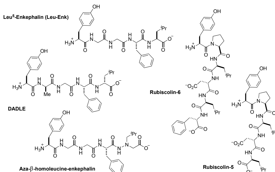
Figure 1. Overview of unbiased (Leu 5 -enkephalin and DADLE ) and biased (Aza-β-Homoleucine-Enkephalin, Rubiscolin-5 and -6) \delta OR peptides.
