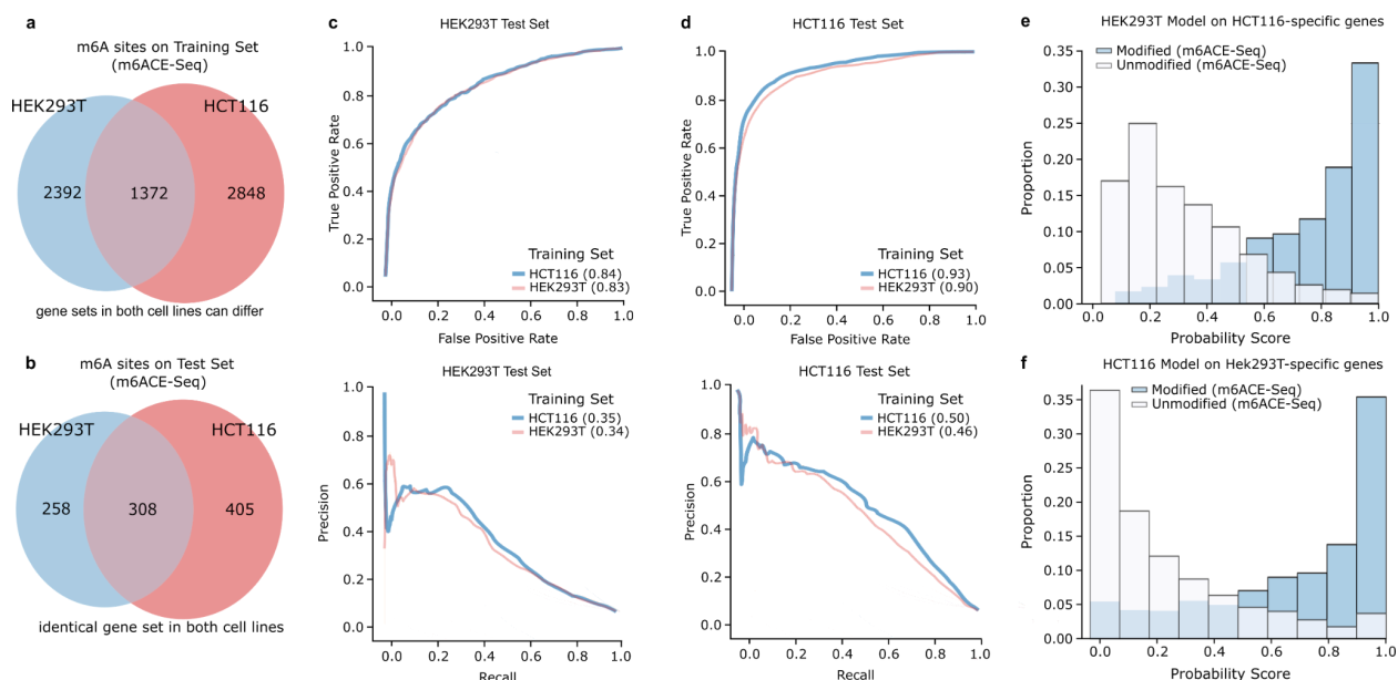
Figure 3. Comparison of m6Anet model across two different cell lines.
