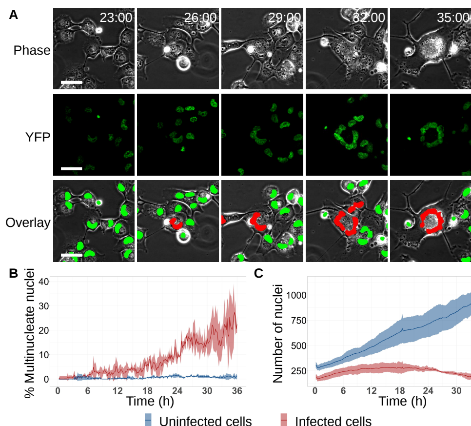
Figure 1: SARS-CoV-2 infected cells fuse to form multinucleated cellular structures with clustered nuclei. (A) Phase contrast (first row), YFP fluorescence (second row), and overlay images (third row) of infected cells, where cell nuclei express YFP. Red in the overlay image denotes nuclei detected as clustered by automated image analysis, while green denotes nuclei detected as non-clustered. Time of image post-infection is on the top right of the phase image as hours:minutes, bar is 50 \mu m. (B) Percent of nuclei in multi-nucleate cells as a function of time. Shown are the mean and standard deviation for infected cells (red) versus uninfected cells (blue). (C) Number of nuclei through time in the timelapse movie. Shown are the mean and standard deviation of the absolute number of nuclei per experiment. Three independent experiments were performed, where each experiment used a different clone of H1299-ACE2 cells.
