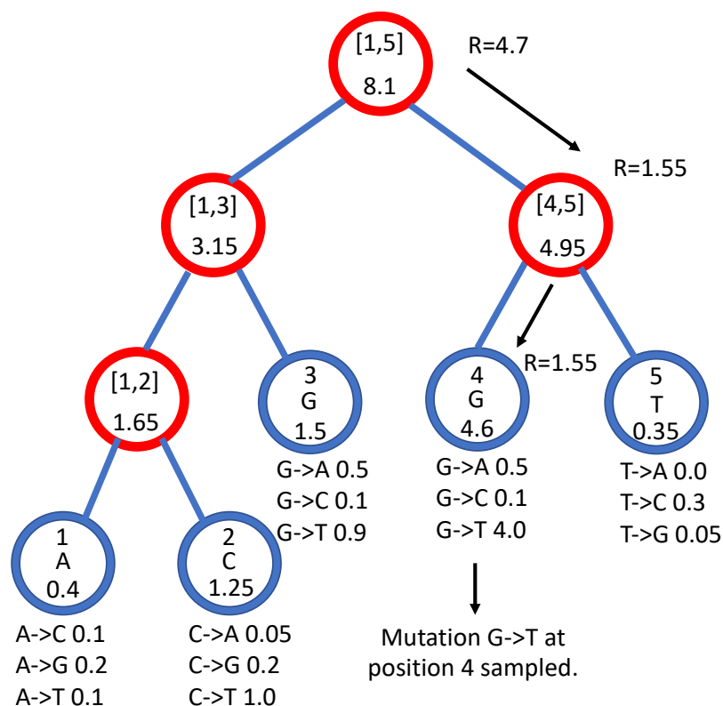
Fig 1. Example genome tree and genome tree search. An example genome search tree for ancestral genome ACGGT. Blue nodes are terminal and red nodes are internal. Inside each node we represent on top the genome positions represented by the node; at the center inside terminal nodes we show the allele of the node; at the bottom of nodes is their total rate. Under each terminal node we show the example relevant mutation rates. The black arrows show an example sampling of one mutation event. A parameter R is assigned an initial random number sampled uniformly between 0 and the total rate 8.1, in this case it is R = 4.7 . As we move downward, the value of R can decrease, as described in Algorithm 2, determining which site will mutate and how. Here, an initial R = 4.7 results in the sampling of a G→T mutation at genome position 4.
