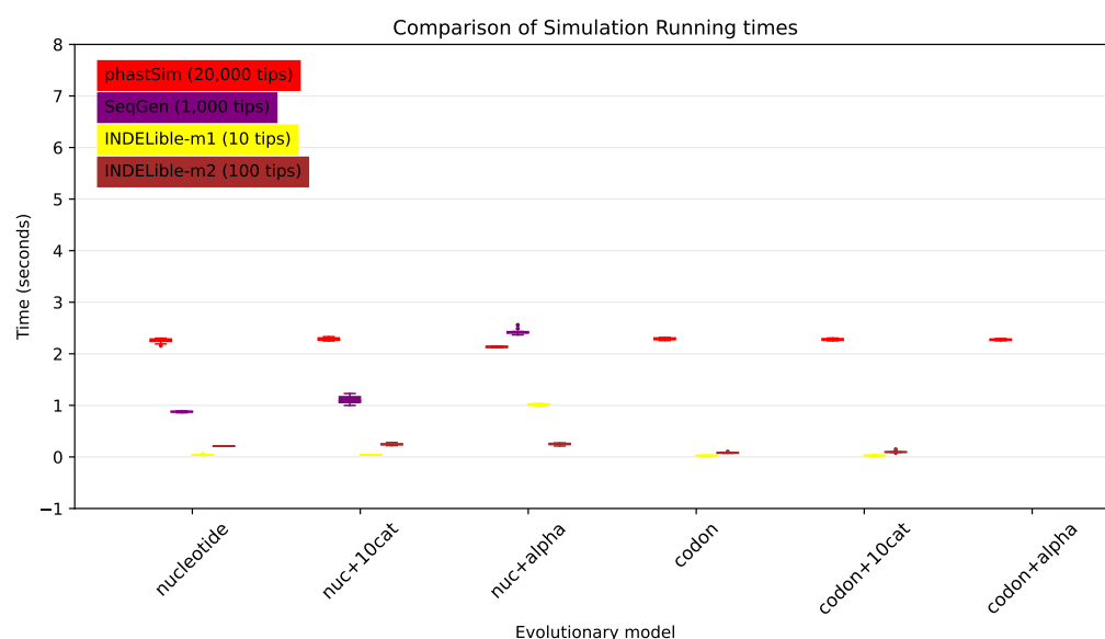
Fig 5. Comparison of running times of different simulators in a SARS-CoV-2 scenario using different evolutionary models. On the Y axis we show the number of seconds it takes to perform simulations using different software. On the X axis is the model used for simulations: “nucleotide” is a nucleotide substitution model without variation; “nuc+10cat” is a nucleotide model with 10 rate categories; “nuc+alpha” is a nucleotide model with continuous variation in rate (each site has a distinct rate sampled from a Gamma distribution); “codon” represents a codon substitution model; “codon+10cat” represents a codon substitution model with 10 categories for \omega ; “codon+alpha” is a codon model with continuous rate variation in mutation rate and in \omega (only allowed in phastSim). Each boxplot represents ten replicates. Seq-Gen does not allow codon models. Colors are as in Fig 3. To aid the visual comparison, we use trees of different sizes for different simulators: 10 tips for INDELible-m1; 100 tips for INDELible-m2; 1,000 tips for SEq-Gen; 20,000 tips for phastSim.
