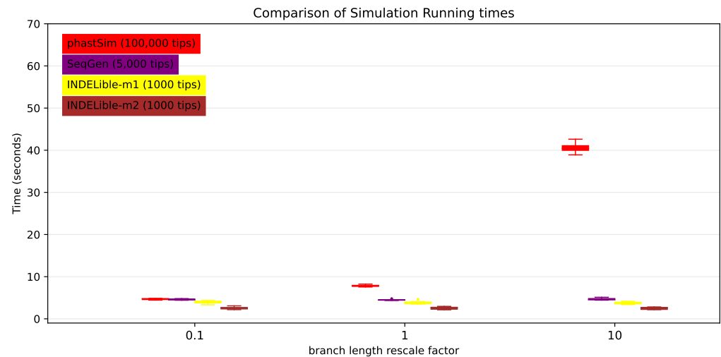
Fig 7. Comparison of running times of different simulators in a SARS-CoV-2 scenario after rescaling the tree branch lengths by different factors. On the Y axis we show the number of seconds it takes to perform simulations using different software. On the X axis is the rescaling factor we use to make the phylogenetic tree branch lengths longer or shorter. Colors are as in Fig 3. To aid the visual comparison, we use trees of different sizes for different simulators: 1000 tips for INDELible; 5,000 tips for Seq-Gen; 100,000 tips for phastSim.
