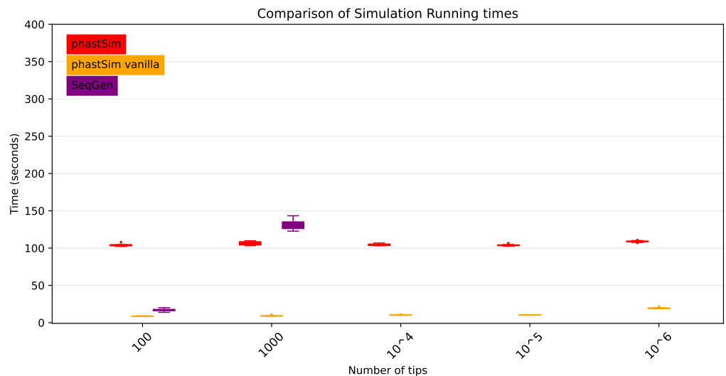
Fig 4. Comparison of running times of different simulators in a scenario similar to E. Coli outbreak data. On the Y axis we show the number of seconds it takes to perform simulations using different software. On the X axis is the number of tips simulated. Each boxplot represents ten replicates. We do not run Seq-Gen for more than 1000 tips due to high computational demand. In red is the time to run phastSim, and in orange is the time for phastSim with the “vanilla” approach. In purple is the time demand of Seq-Gen.
