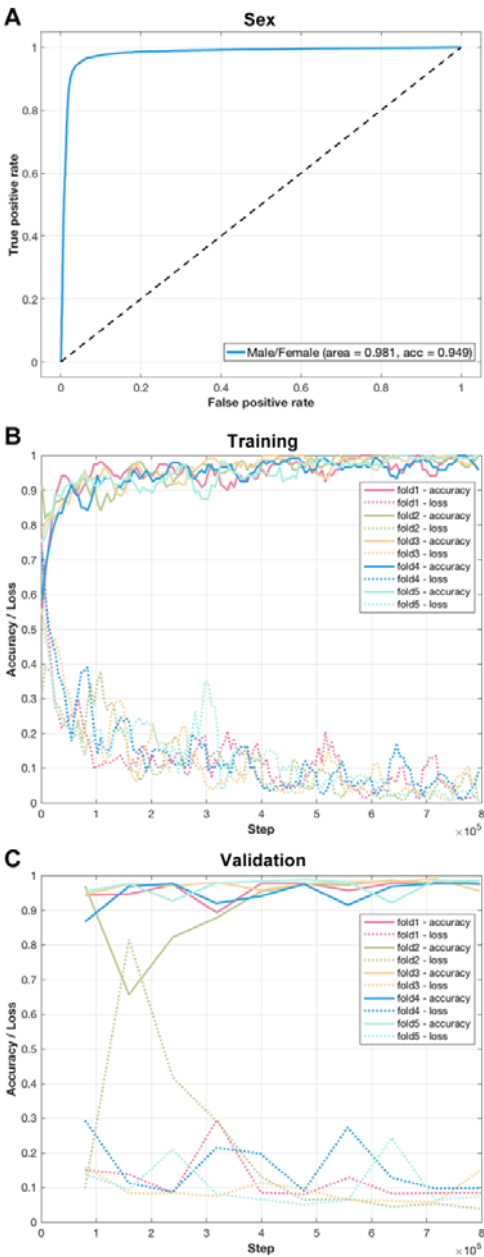
296 Fig. 2 | Performance of the sex classifier. (A) The receiver operating characteristic curve of 297 the sex classifier. (B) The tensorboard monitor graph of the sex classifier in the training 298 sample. The curve was smoothed for better visualization. (C) The tensorboard monitor graph 299 of the sex classifier in the validation sample.
