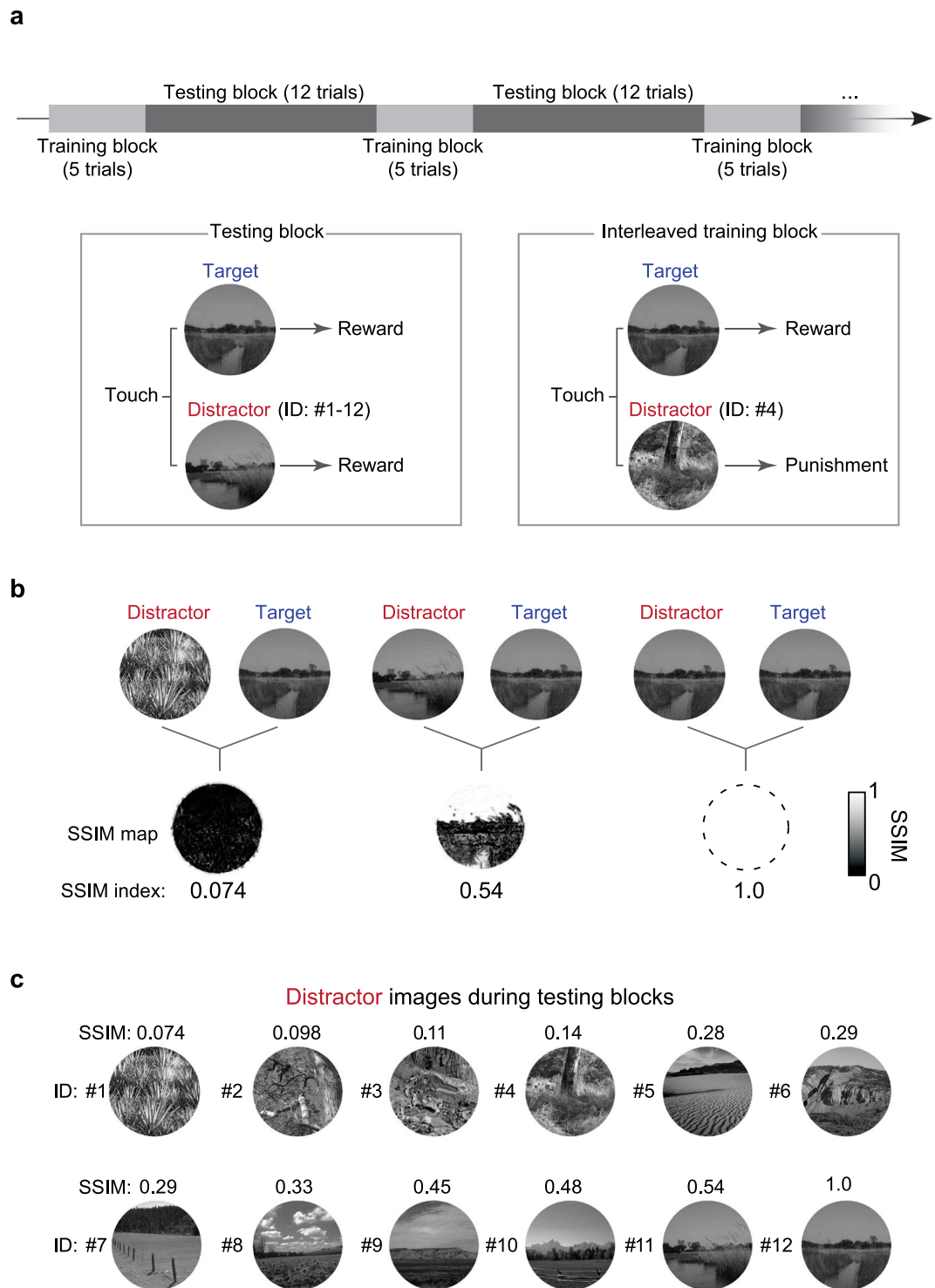
Figure 2. Testing procedure and SSIM index for quantifying expected difficulty. (a) NID testing sessions were composed of two types of blocks, testing blocks and interleaved training blocks. In testing block trials, one of 12 distractor images was presented with a target image. In interleaved training trials, the same distractor image was always presented with a target image. The incorrect choices were only punished (with a time-out and no reward) in the interleaved training trials. (b) Distractor and target images displayed in a trial were compared using structural similarity (SSIM). An SSIM map was obtained for each pair, and averaged yield a scalar SSIM index for the image pair. (c) Twelve distractor images were used, which varied in SSIM index with the target image (see also Supplementary Table 1). One distractor (ID: 12) was the same as the target image, and served as an internal control.
