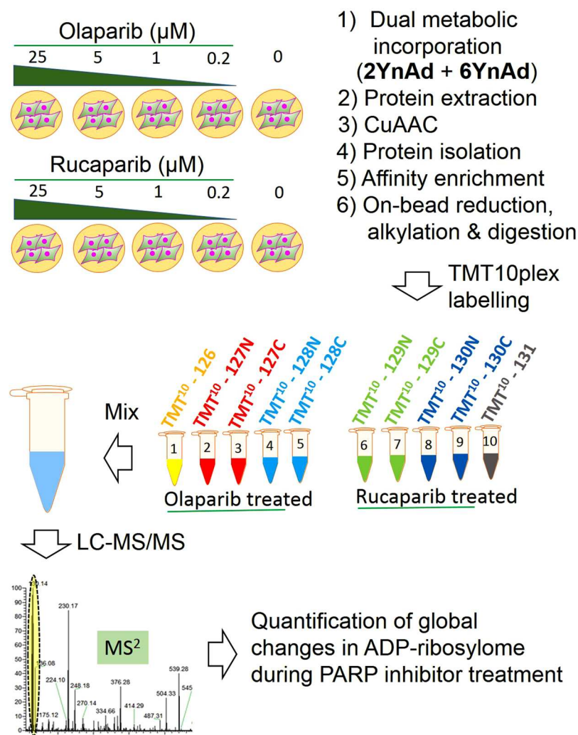
Figure 4. Schematic illustrating the workflow involving parallel treatment of PARP inhibitors Olaparib and Rucaparib followed by dual metabolic labelling of 6YnAd and 2YnAd, click chemistry, affinity enrichment of the labelled proteins on NeutrAvidin-Agarose beads and TMT10plex-based quantification of global changes in the cellular ADP-ribosylome.
