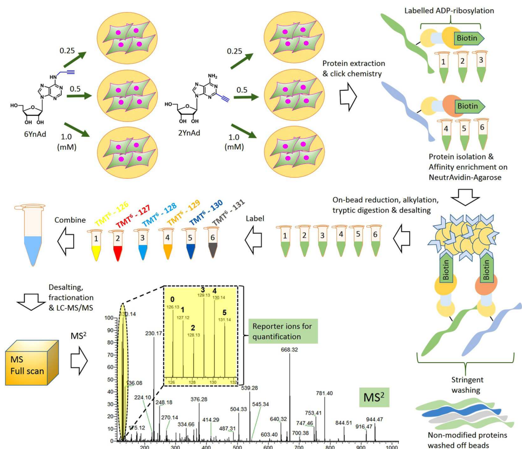
Figure 2. Schematic illustrating the experimental workflow for quantitative comparison of metabolic labelling between 2YnAd and 6YnAd. MDA-MB-231 cells were metabolically labelled with 3 different concentrations of 2YnAd and 6YnAd in parallel. After cell lysis and click reaction with a biotin-containing capture reagent, the labelled proteins are affinity enriched on NeutrAvidin-Agarose resins. Stringent washing at this stage removes unmodified proteins from the beads. After on-bead reduction, alkylation and tryptic digestion, the eluted peptides are desalted and each sample is labelled using a unique TMT6plex channel. After quenching the TMT reactions, the 6 samples are mixed together, fractionated and subjected to nanoflow LC-MS/MS analysis. Quantification of reporter ions from the MS/MS spectra provides relative quantification of labelling efficiencies of the two compounds at all three tested concentrations.
