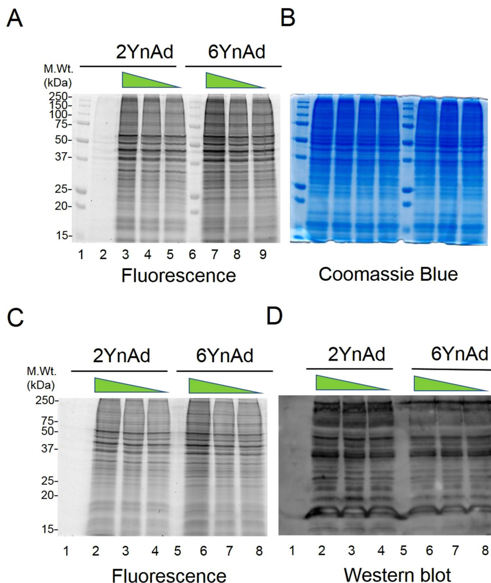
Figure 1. (A) Qualitative assessment of 2YnAd and 6YnAd labelling in MDA-MB-231 cells by in-gel fluorescence scanning. Lanes 1 and 6: molecular weight marker; lane 2: DMSO control; lanes 3, 4 and 5 (1 mM, 0.5 mM and 0.25 mM 2YnAd respectively) and lanes 7, 8 and 9 (1 mM, 0.5 mM and 0.25 mM 6YnAd respectively). (B) Coomassie blue staining of the same gel. (C) In-gel fluorescence scan following the metabolic incorporation, cell lysis, click chemistry and affinity enrichment. Lane 1: DMSO control; Lanes 2, 3 and 4: 1 mM, 0.5 mM and 0.25 mM respectively of 2YnAd was used for the metabolic labelling; lane 5: empty and lanes 6, 7 and 8: 1 mM, 0.5 mM and 0.25 mM respectively of 6YnAd was used for the metabolic labelling. (D) Western blot of the same gel after electrotransfer of proteins onto a nitrocellulose membrane probed using an anti-pan-ADP-ribose antibody (MABE1016, EMD Millipore).
