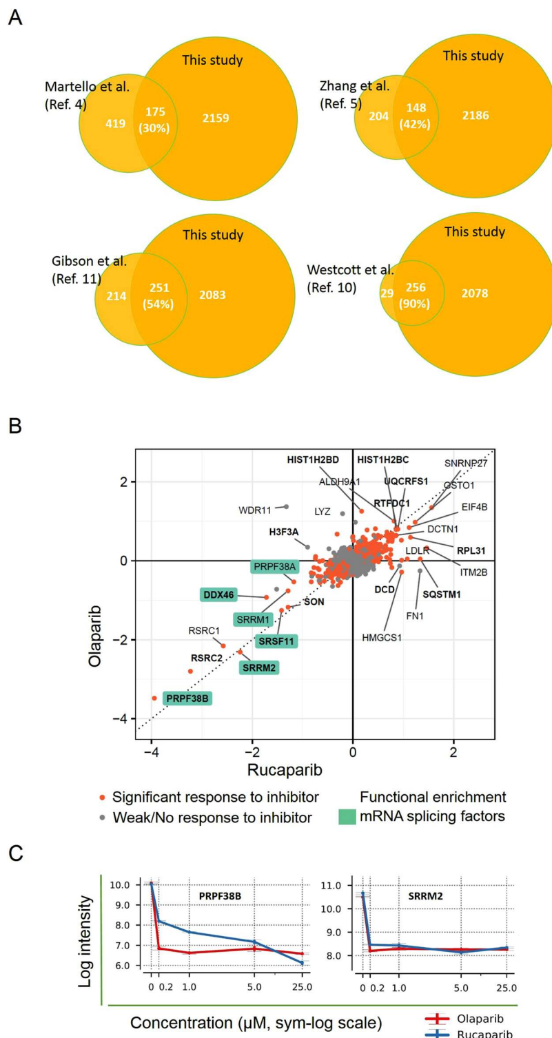
Figure 5. (A) Venn diagram assessment of the overlap between the proteins identified to be ADP-ribosylated in this study and previously published data sets. (B) Scatter plot showing mean log 2 responses in the level of ADP-ribosylation of endogenous proteins to 25 \mu M of the inhibitors Olaparib and Rucaparib after removing the effects associated with technical replicate bias. Proteins whose response to inhibitors is significant (see LIMMA processing and statistical testing) are highlighted in orange. Proteins reported to be ADP-ribosylated in other studies from ADPrBoDB 14 are highlighted in bold. Factors involved in mRNA splicing are highlighted with a cyan rectangle around their labels. (C) Quantitative changes in the reporter intensities (log 2 scale) of mRNA splicing proteins pre-mRNA splicing factor 38B (PRPF38B) and serine/arginine repetitive matrix protein 2 (SRRM2) as a function of concentration of the inhibitors Olaparib (red) and Rucaparib (blue).
