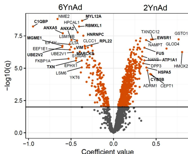
Figure 3. Volcano plot for the cofactor effect coefficients in the linear model, where positive values on the x-axis indicate preference for 2YnAd and negative values indicate preference for 6YnAd. The significance of the cofactor effect coefficients is computed using a moderated t-test based on the hierarchical Bayesian model as implemented in LIMMA, and adjusted p values ( -\log_{10} scale) are plotted on the y-axis with significantly enriched proteins coloured in red. Proteins reported to be ADP-ribosylated in other studies from ADPrigoDB 22 are highlighted in bold.
