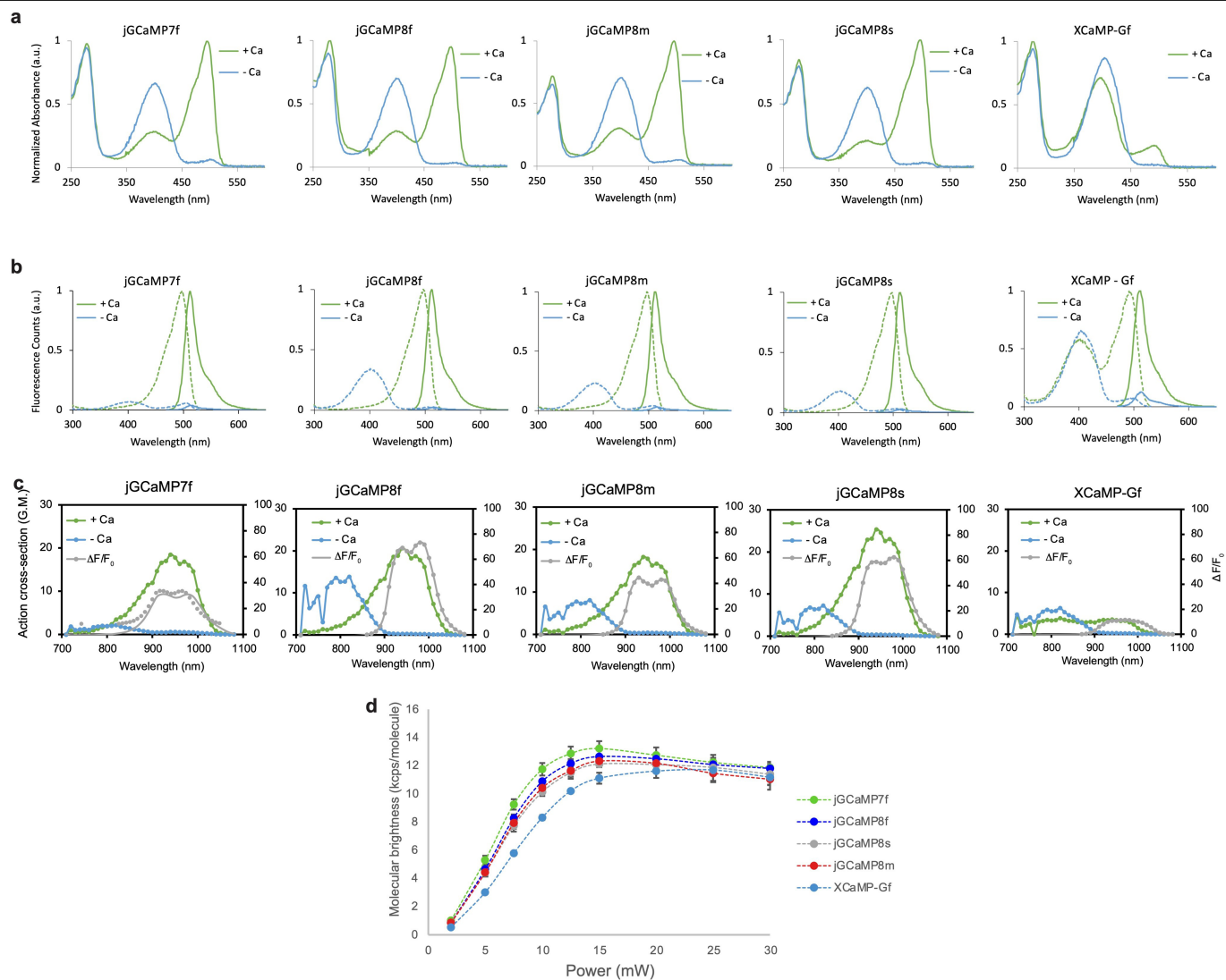
Extended Data Fig. 5 | Photophysical characterization of jGCaMP8 sensors.
