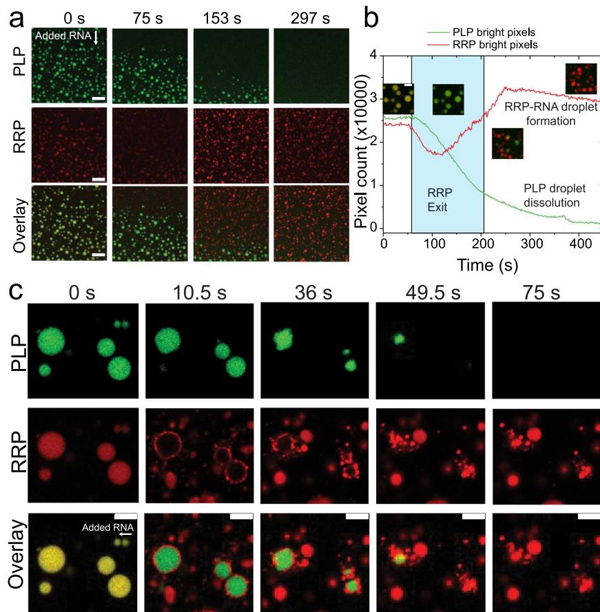
Fig. 2 RNA induces condensate switching from PLP-RRP to RRP-RNA. a Multicolor confocal fluorescence time-lapse images showing dissolution of PLP-RRP (RRP: FUS RGG3 ) droplets and subsequent formation of RRP-RNA droplets upon addition of poly(rU) RNA. Scale bar = 20 \mu m. b A plot of the total area covered by condensates in the green (PLP) and red (RRP) channels for the data shown in ( a ) and in Movie S1. The areas were calculated by counting the green pixels (for PLP) and the red pixels (for RRP) and plotted as a function of time. The images indicate the various stages of sample evolution after RNA addition. The white region (left) indicates the time-window where PLP and RRP co-localize; the cyan shaded region indicates the time-window when RRP is leaving the PLP-RRP condensates; the white region (right) indicates the subsequent dissolution of PLP-RRP condensates and the formation of RRP-RNA condensates. Source data are provided as a Source Data file. Scale bar represents 5 \mu m. c Same assay as ( a ) but with poly(rA) RNA. (RRP: [RGRGG] 5 ). Scale bars represent 4 \mu m. All samples were prepared in 25 mM Tris-HCl, 150 mM NaCl, and 20 mM DTT buffer. PLP: FUS PLP .
