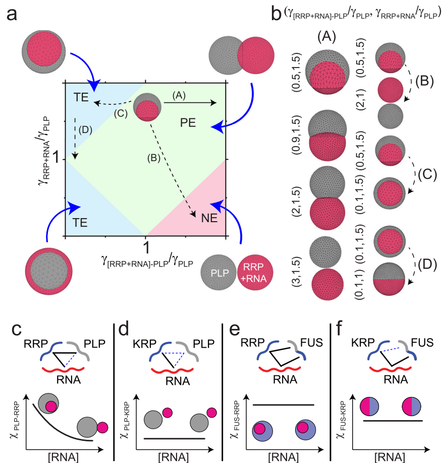
Fig. 6 The stability diagram of a pair of coexisting condensates provides a link between intermolecular interactions and multiphasic morphology.
